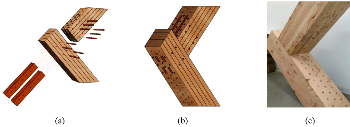
Fig. 8. Beam-column connection for CWDLT members (a) exploded view, (b) assembled connection utilising CWDLT members and (c) manufactured connection prior to testing.
