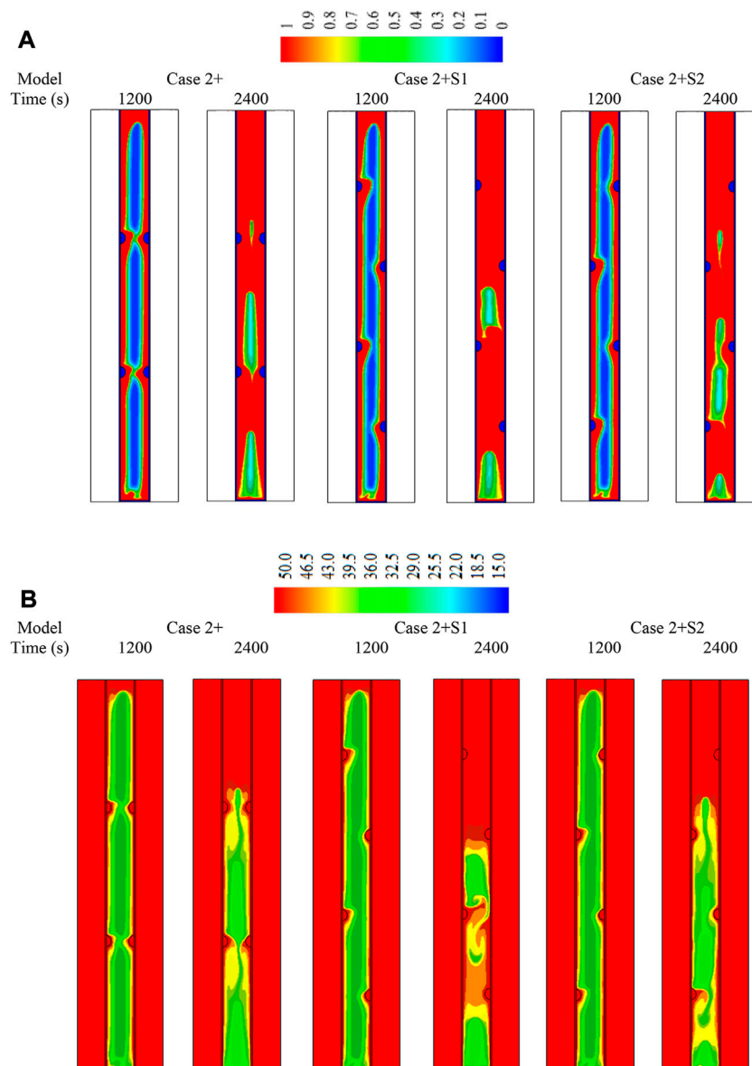
FIGURE 9 (A) Liquid fraction and (B) temperature contours of the PCM for different numbers of hemispherical fins ( N equals 2) and left- and right-staggered fins, with an added flat fin to the base of the PCM domain for all the cases.
