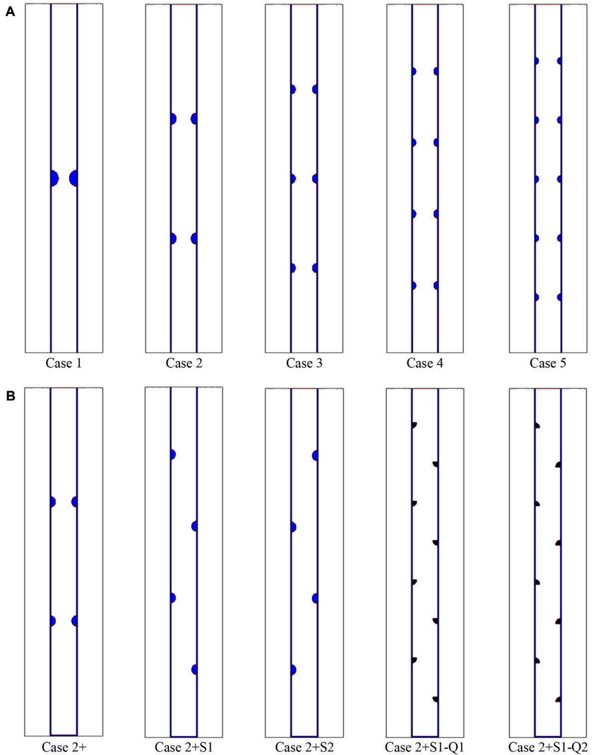
FIGURE 2 Schematic of the proposed system on the effect of (A) the number of hemispherical fins without an added fin to the bottom and (B) case 2 modified to several configurations to reach a better thermal performance of the system.
