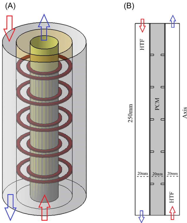
FIGURE 3 The boundary conditions and dimensions of the proposed system in (A) full domain and (B) axisymmetric condition.
