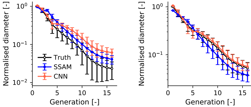
Figure 6: Generated airway diameter for our image-processing modalities on two cases from the LUNA16 dataset. Markers show the normalised mean diameter per generation. Error bars show \pm 1S.D. where S.D. is the standard deviation.
