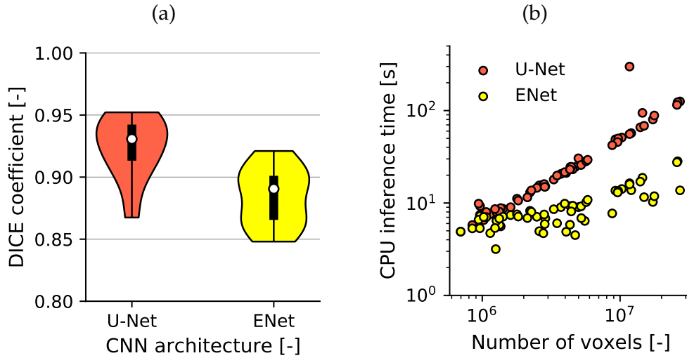
Figure S3: Comparison of accuracy and speed for U-Net and ENet architectures. Panels show (a) DICE coefficient from 10 scans in validation set, and (b) inference time relative to size of image, computed on combined training and validation set.
