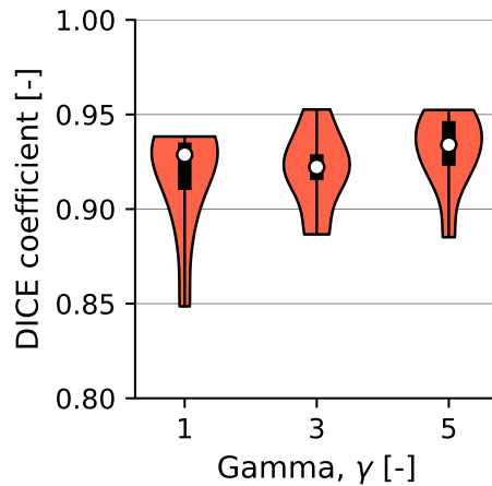
Figure S2: Sensitivity analysis of focal loss parameter \gamma in Equation 11 to optimise CNN DICE coefficient. CNNs were trained with no augmentations and results were computed from 10 scans in validation set.
