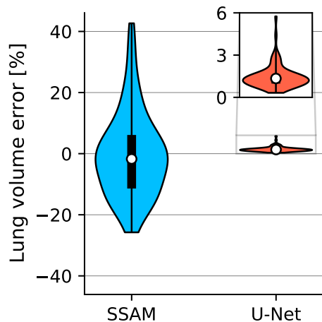
Figure 3: Lung space volume error from SSAM and U-Net reconstructions of patients from LUNA16 dataset. Inset shows U-Net lung space volume error, where the U-Net results were produced using the pretrained U-Net from Hofmanninger et al. (2020).
