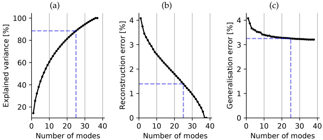
Figure 2: Assessment of sensitivity of SSAM metrics to number of modes included in the model. Panels show (a) explained variance based on number of modes, (b) reconstruction error for shapes in training set, (c) generalisation error for unseen shapes. When the model describes 90% of the population variance (indicated by blue dashed line), the generalisation error in adapting the model to unseen shapes is saturated.
