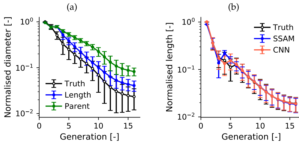
Figure S6: Comparison of diameter error in full conducting airway tree from a SSAM with varying models to calculate diameter. The ‘truth’ results were generated from ground truth segmentations with the ‘parent’ model for diameter (Bordas et al., 2015).
