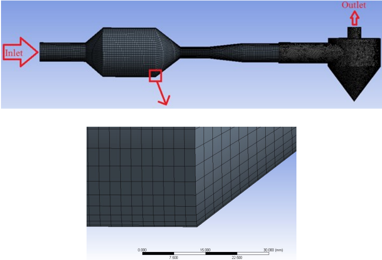
Figure 2. The meshing illustration of design A, which has a larger diameter expansion pipe and venturi between expansion pipe and swirl chamber
