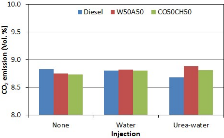
Figure 12. CO 2 emissions of diesel, W50A50 and CO50CH50 with the modified SNCR application.
