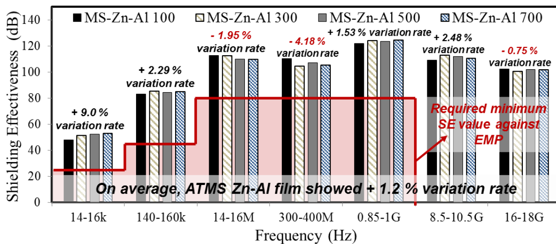
Figure 4. SE test result of ATMS coatings by Zn-Al in regards to thickness.
