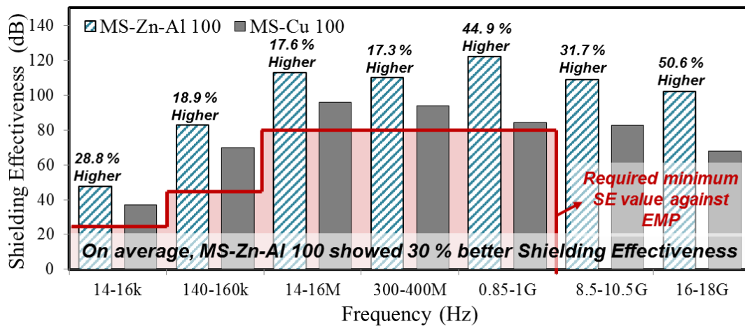
Figure 6. SE test result between MS-Zn-Al 100 and MS-Cu 100.
