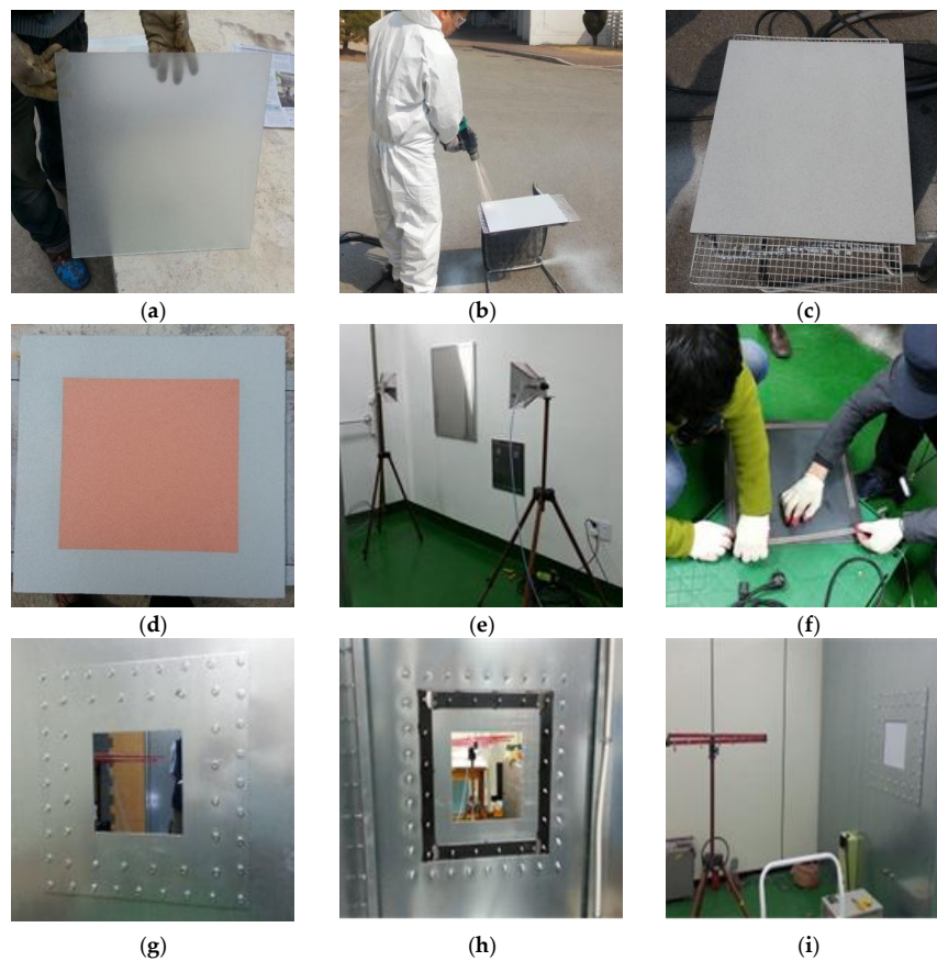
Figure 2. Experimental process. (a) Substrate preparation; (b) application of ATMS; (c) specimen after ATMS (Zn-Al coating); (d) specimen after ATMS (Cu coating); (e) calibration work; (f) gasket installation; (g) EMP shielding wall (outside); (h) EMP shielding wall (inside); and (i) SE test.
