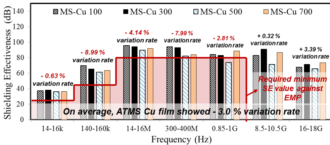
Figure 5. SE test result of ATMS coatings by Cu in regards to thickness.
