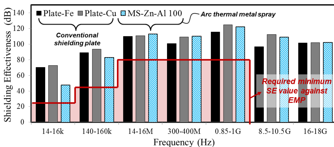
Figure 9. SE test result between metal plate and ATMS coating by Zn-Al.
