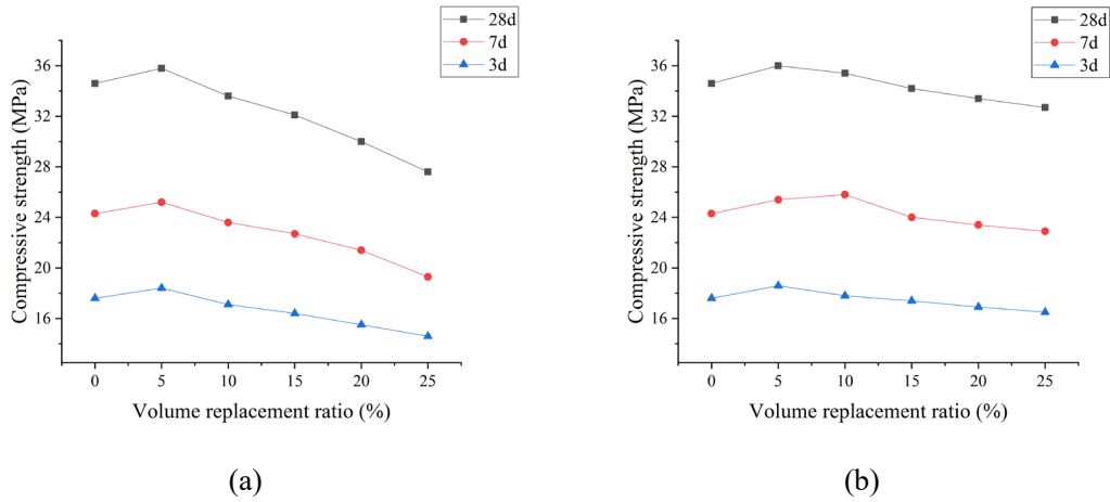
Fig. 5. Concrete compressive strength:(a) unmodified concrete, (b) modified concrete
