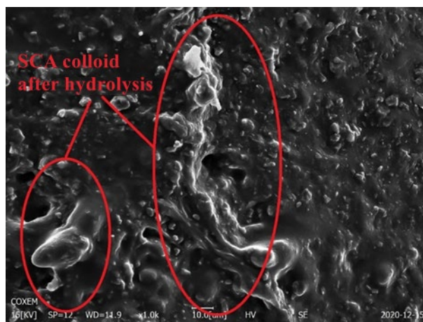
Fig. 15. surface morphology of modified recycled PVC particles
