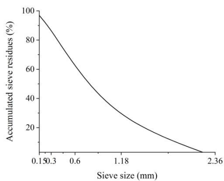
Fig. 1. Particle size distributions of sand
