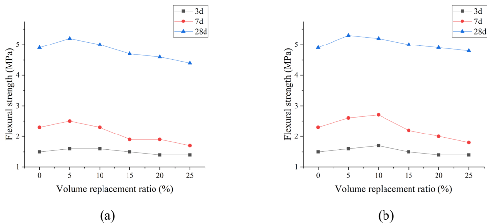
Fig. 10. Concrete flexural strength:(a) unmodified recycled PVC concrete, (b) modified recycled PVC concrete
