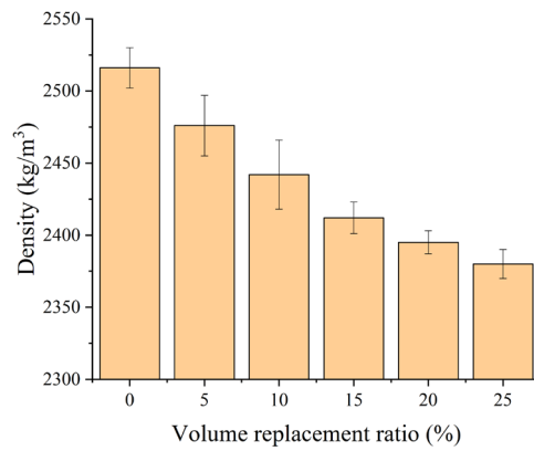
Fig. 3. Relationship between concrete density and recycled PVC particle volume replacement ratio
