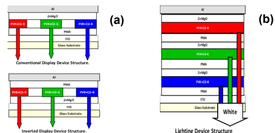
Figure 1. (a) Conventional and Inverted device structure for Display. (b) Conventional Tandem device structure for Lighting panels.
