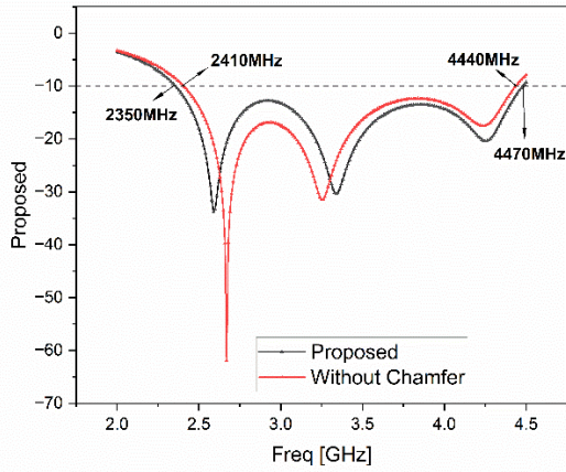
Figure 2. Simulated reflection coefficient
