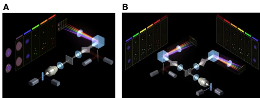
Figure 219. The optical layout of the ImageStreamX Mk-II one camera, six channel (left), and two camera, 12 channel (right) systems
