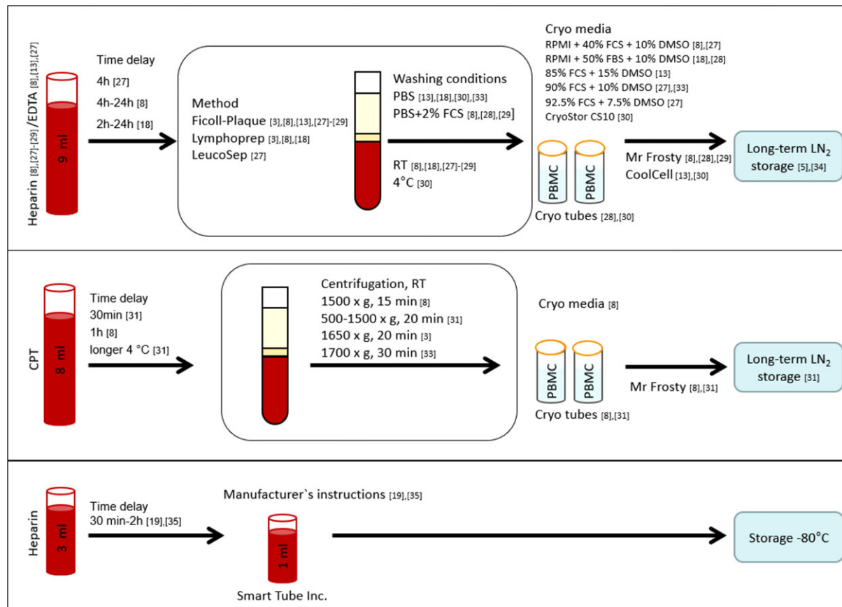
Figure 241. Brief overview of PBMC isolation or whole blood stabilization. References for each process are indicated.
