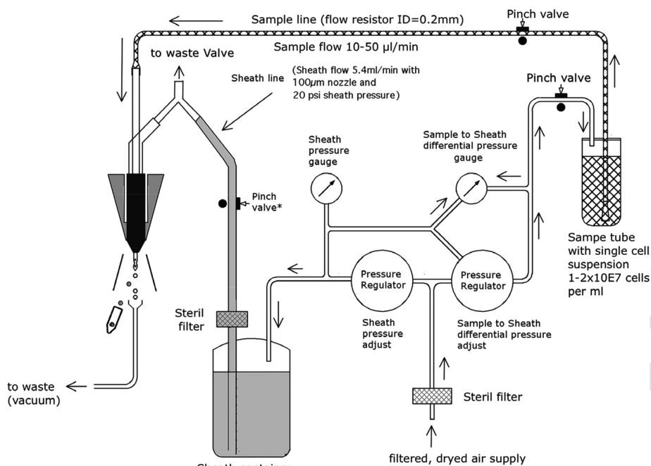
Figure 4. Schematics of fluidics of a jet in air sensing cell sorter.
