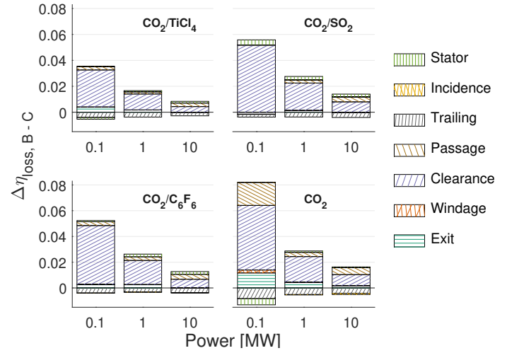
FIGURE 12: DIFFERENCE IN LOSS CONTRIBUTIONS BETWEEN CASE-B AND CASE-C
