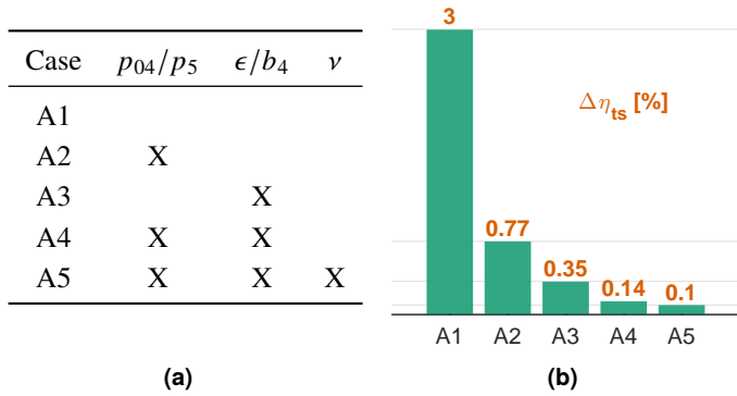
FIGURE 16: (A) PARAMETERS ASSUMED FIXED IN EACH SUB-CASE. (B) DIFFERENCE IN EFFICIENCY BETWEEN \text{CO}_2/\text{TiCl}_4 AND \text{CO}_2 0.1 MW TURBINES FOR EACH SUB-CASE
