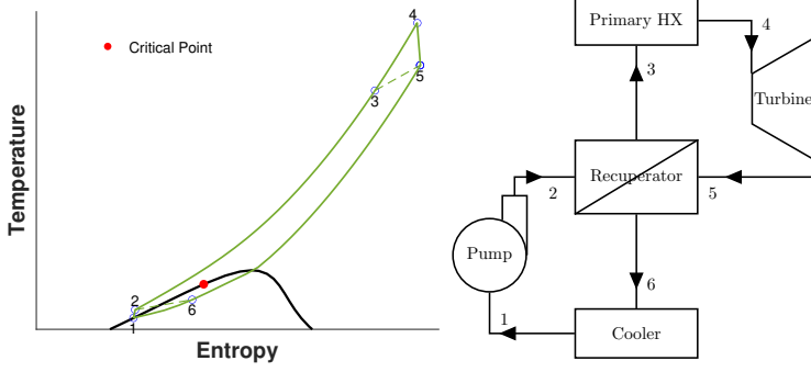
FIGURE 1: T - s DIAGRAM AND SCHEMATIC OF A SIMPLE RECUPERATED \text{TCO}_2 CYCLE
