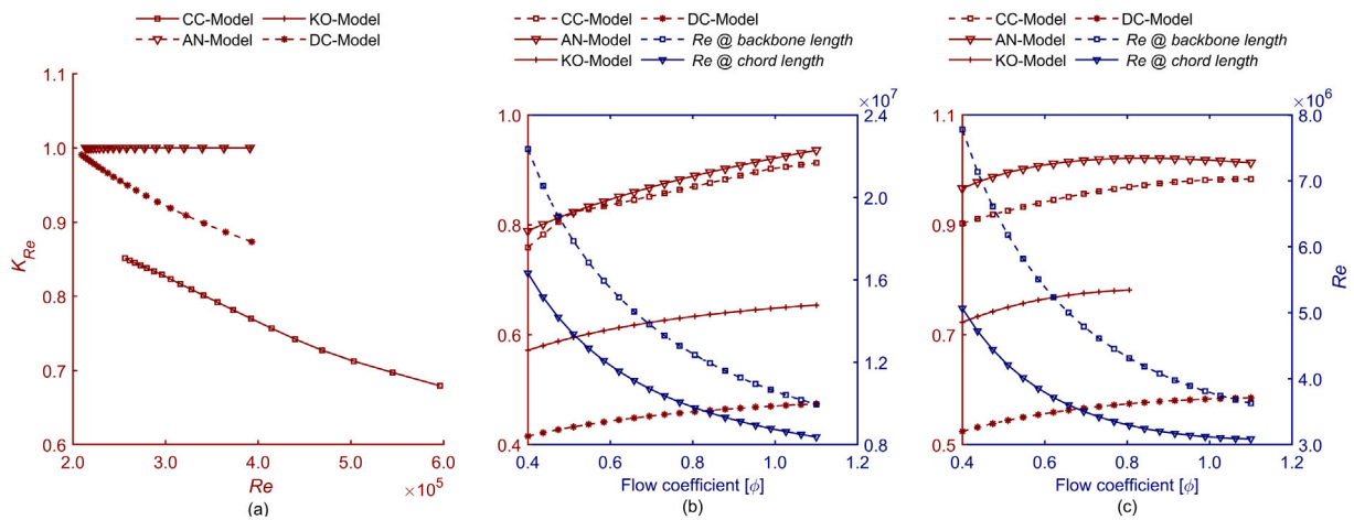
Fig. 5. (a) Reynolds number [ Re ] versus Reynolds number correction factor [ K_{Re} ] for the 1st stage of the 100 MW air turbine, flow coefficient versus [ Re ] and [ K_{Re} ] for the 1st stage of (b) 100 MW sCO_2 turbine (c) 1 MW ORC turbine.
