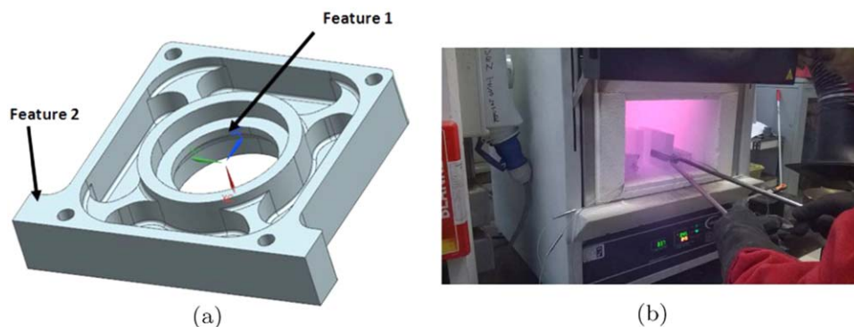
Figure 1. (a) CAD model of the manufactured part. Two features were measured for the purpose of surface metrology analysis. Each feature labelled is associated with one or two operations which correspond to the machining process component which produced the feature. (b) Heat treatment of the steel blocks.
