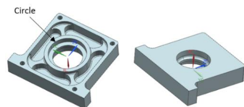
Fig. 1. CAD model of the bearing housing part.
