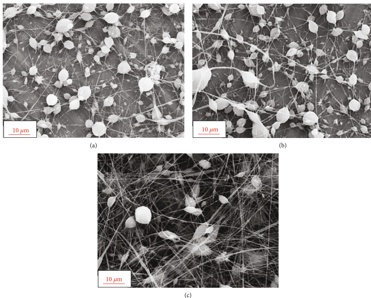
FIGURE 8: SEM microscopy shows the electrospun membrane morphology and quality from suspensions: (a) GO-0.5%, (b) GO-1.5%, and (c) GO-2.5%. Many beads and relatively fewer fibers were observed in GO-0.5% and GO-1.5%, while a decent nonwoven fibrous structure with a reduced number of beads was produced in GO-2.5%.
