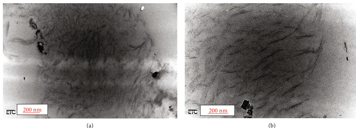
FIGURE 9: TEM image of cross-section of the membrane cast from (a) CNT-0.03% to (b) CNT-0.05% suspensions. The MWCNTs or small nanotube bundles were well dispersed with a certain degree of orientation in the MWCNT composites.
