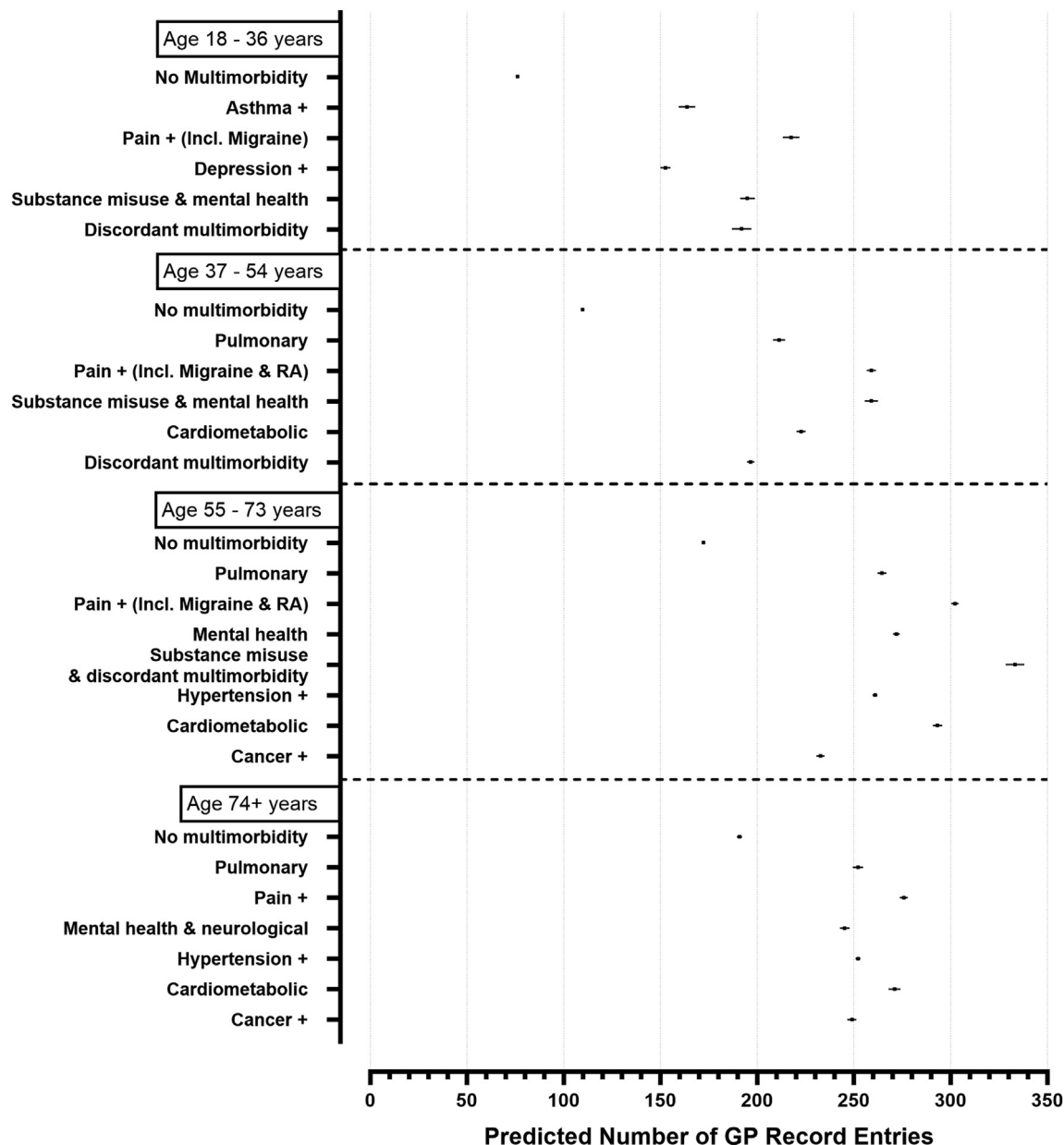
Fig. 3: Predicted number of GP use by MLTC clusters over a 10-year follow up in SAIL. All other covariates in the model were set to their mean value in the respective age group. Error bars represent 95% confidence intervals.
