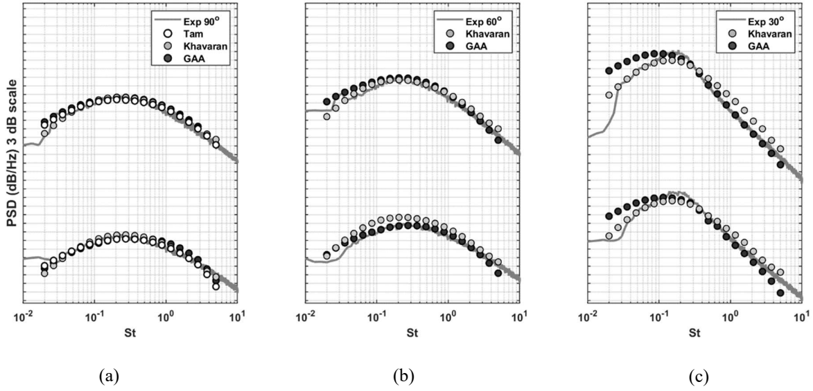
Fig. 5. Noise spectra predictions of the cold (bottom) and hot (top) SILOET jet using the correlation scales based on the turbulent kinetic energy and meanflow vorticity reconstructed from RANS: comparison of the Tam and Auriault, Khavaran, and GAA models with the experiment for 90° (a), 60°(b), and 30° (c) observer angles. The unit scale on the PSD axis is 3dB.
