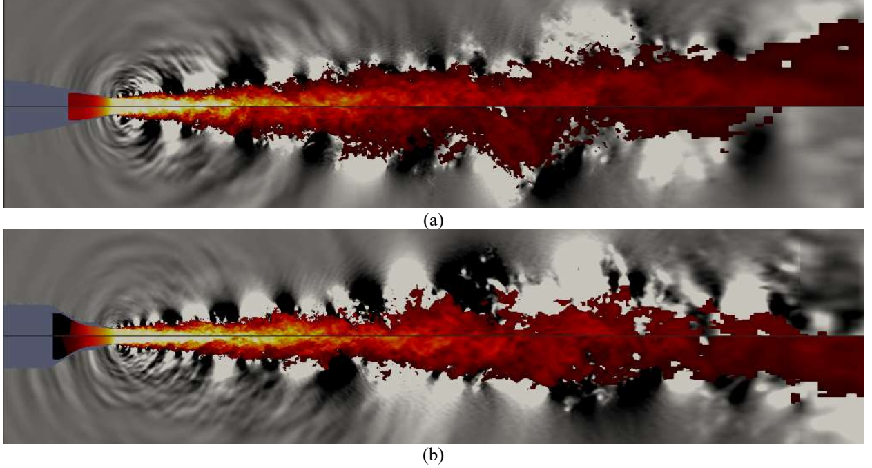
Fig. 1 Instantaneous velocity and pressure field distributions from the LES solution of the cold (top) and hot (bottom) SILOET jets (a); and NASA SHJAR SP 3 (top) and SP 7 (bottom) jets (b).
