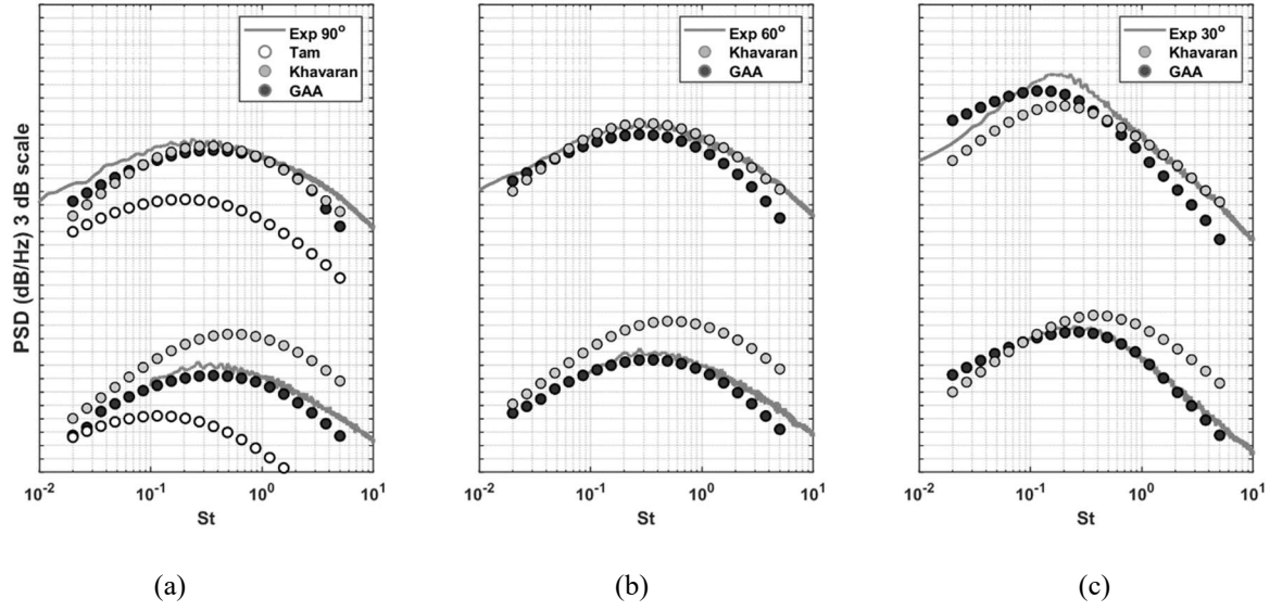
Fig. 9 Noise spectra predictions of the SHJAR SP3 (bottom) and SP7 (top) jets jet using the correlation scales based on the turbulent kinetic energy and meanflow vorticity reconstructed from RANS with dimensionless parameters of the cold SILOET jet model: comparison of the Tam and Auriault, Khavaran, and GAA models with the experiment for 90° (a), 60°(b), and 30° (c) observer angles. The unit scale on the PSD axis is 3dB.
