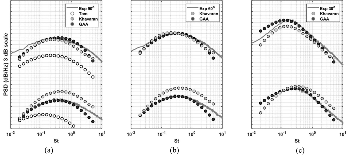
Fig. 10 Noise spectra predictions of the SHJAR SP3 (bottom) and SP7 (top) jets jet using the correlation scales based on the turbulent kinetic energy and meanflow vorticity reconstructed from LES with dimensionless parameters of the cold SILOET jet model: comparison of the Tam and Auriault, Khavaran, and GAA models with the experiment for 90° (a), 60°(b), and 30° (c) observer angles. The unit scale on the PSD axis is 3dB.
