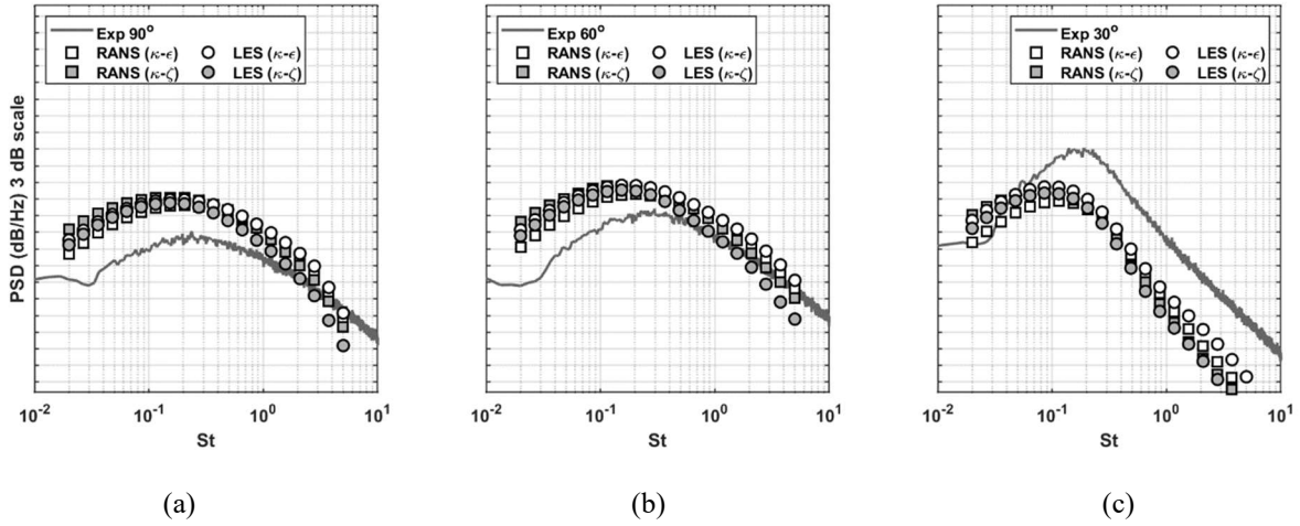
Fig. 12 Noise spectra predictions for the cold SILOET jet using Tam and Auriualt's model using the dimensionless parameters computed from the NASA SP7 jet model: comparison of the RANS- and LES-based acoustic predictions for dissipation rate- and vorticity-based acoustic scales with the experiment for 90° (a), 60°(b), and 30° (c) observer angles. The unit scale on the PSD axis is 3dB.
