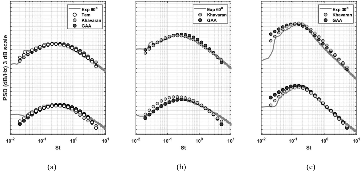
Fig. 6. Noise spectra predictions of the cold (bottom) and hot (top) SILOET jet using the correlation scales based on the turbulent kinetic energy and meanflow vorticity reconstructed from LES: comparison of the Tam and Auriault, Khavaran, and GAA models with the experiment for 90° (a), 60°(b), and 30° (c) observer angles. The unit scale on the PSD axis is 3dB.
