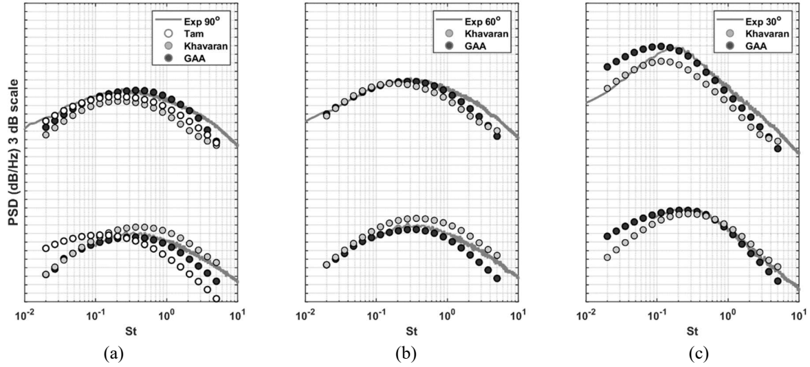
Fig. 8 Noise spectra predictions of the SHJAR SHJAR SP3 (bottom) and SP7 (top) jets using the correlation scales based on the turbulent kinetic energy and dissipation rate reconstructed from LES with dimensionless parameters of the cold SILOET jet model: comparison of the Tam and Auriault, Khavaran, and GAA models with the experiment for 90° (a), 60°(b), and 30° (c) observer angles. The unit scale on the PSD axis is 3dB.
