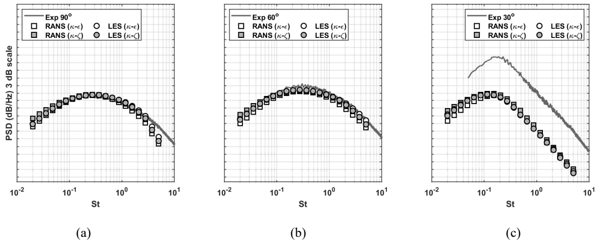
Fig. 11 Noise spectra predictions of the SHJAR SP7 jet using Tam and Auriault' model: comparison of the RANS- and LES-based acoustic predictions for dissipation rate- and vorticity-based acoustic scales with the experiment for 90^\circ (a), 60^\circ (b), and 30^\circ (c) observer angles. The unit scale on the PSD axis is 3dB.
