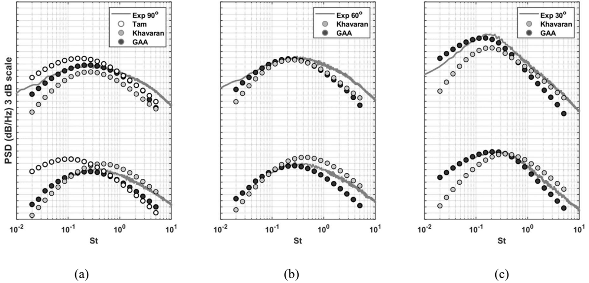
Fig. 7 Noise spectra predictions of the SHJAR SP3 (bottom) and SP7 (top) jets using the correlation scales based on the turbulent kinetic energy and dissipation rate reconstructed from RANS with dimensionless parameters of the cold SILOET jet model: comparison of the Tam and Auriault, Khavaran, and GAA models with the experiment for 90° (a), 60°(b), and 30° (c) observer angles. The unit scale on the PSD axis is 3dB.
