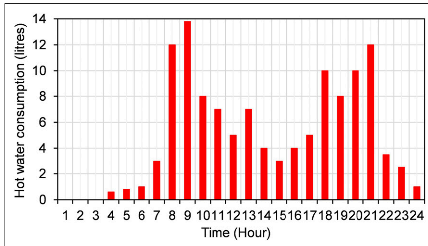
Figure 2. Average hourly hot water demand profiles derived from 12 months of measured data in LEEDR for 24 hours.
