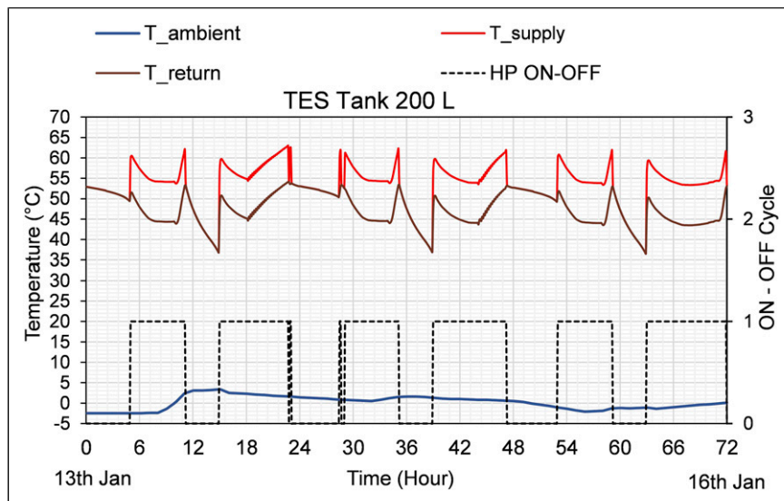
Figure 8. Heat pump operation and supply and return from 200 L storage tank.
