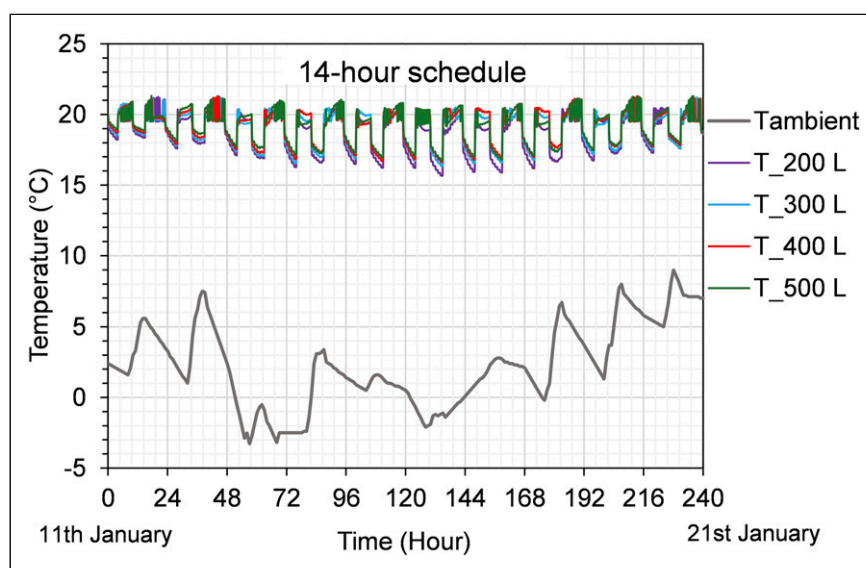
Figure 12. Variation in temperature in the living room for different hot water storage volumes during a 14-hour operating schedule.
