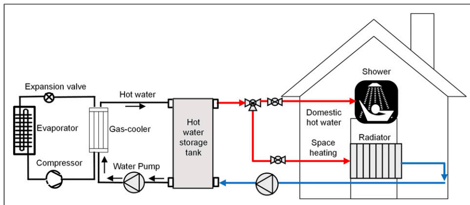
Figure 4. The schematic of the whole system.
