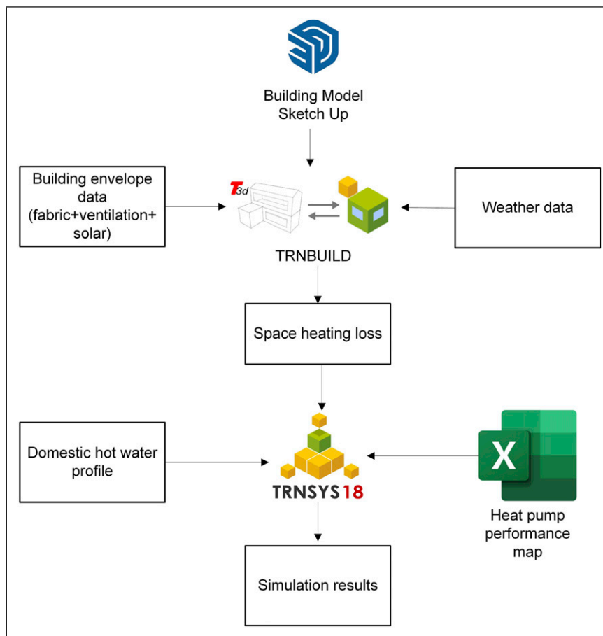
Figure 5. TRNSYS simulation flow chart.
