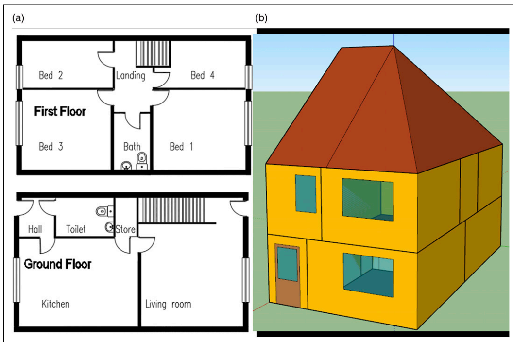
Figure 1. (a) Floor plan of the studied semi-detached four-bedroom house, (b) 3D model of the dwelling.
