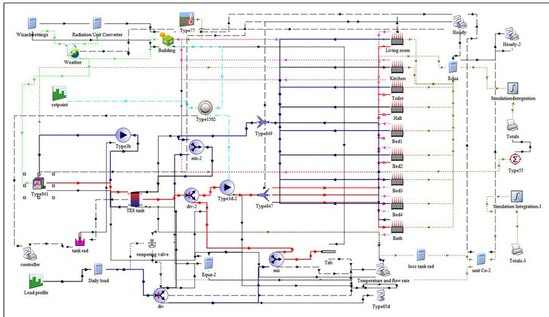
Figure 6. TRNSYS model of the proposed system.
