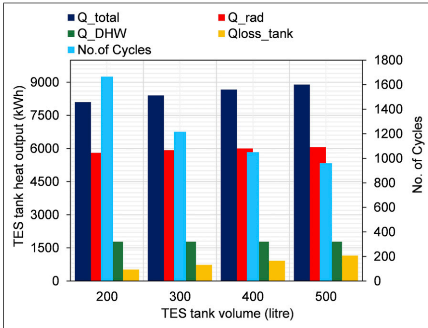
Figure 10. Thermal energy generated and losses for different storage tank sizes.
