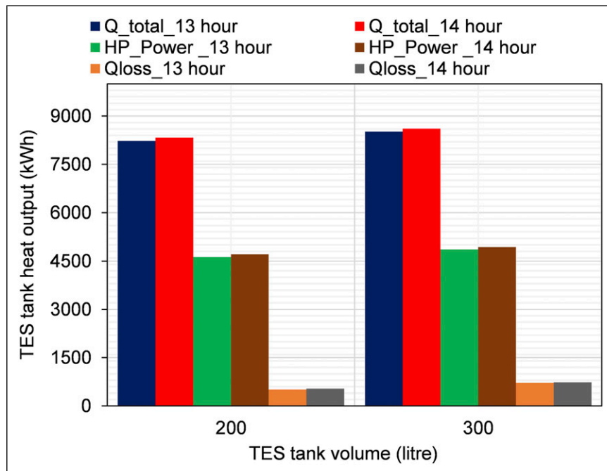
Figure 13. Energy comparison between 200 L and 300 L storage tanks.
