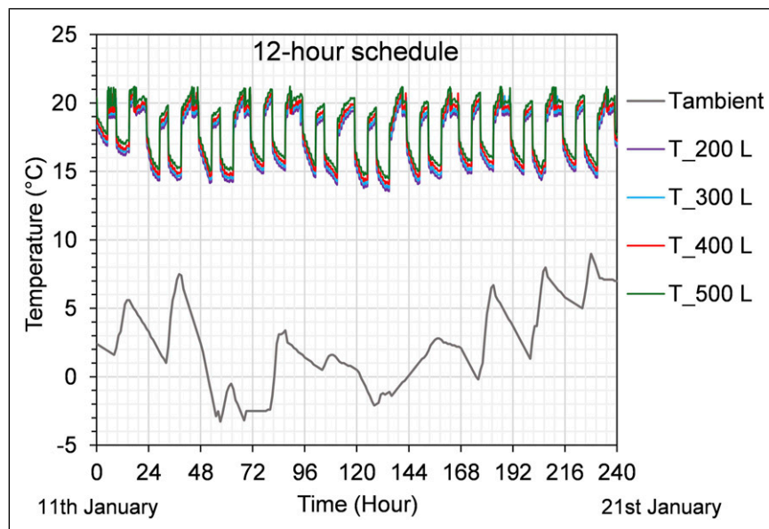
Figure 9. Variation in temperature in the living room for different hot water storage volumes during a 12-hour operating schedule.
