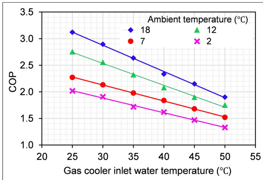
Figure 3. Performance map of the CO 2 AWHP.
