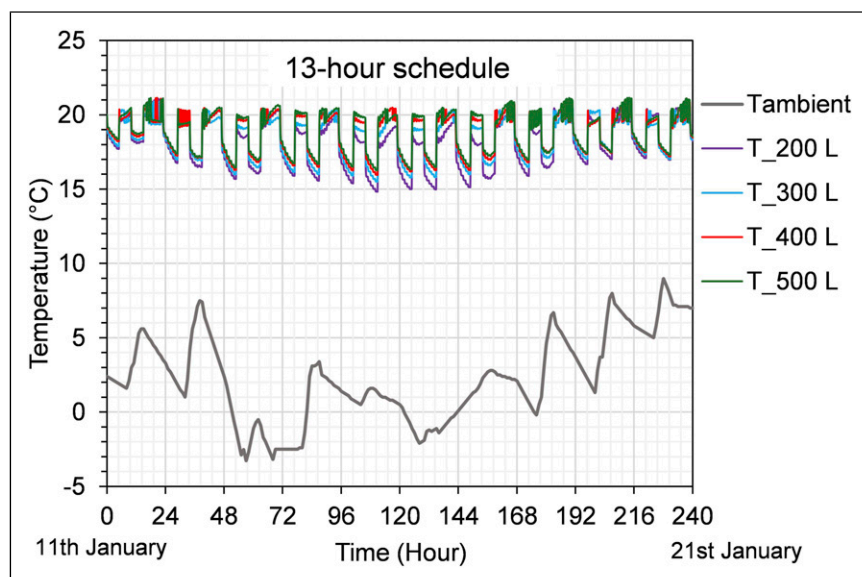
Figure 11. Variation in temperature in the living room for different hot water storage volumes during a 13-hour operating schedule.
