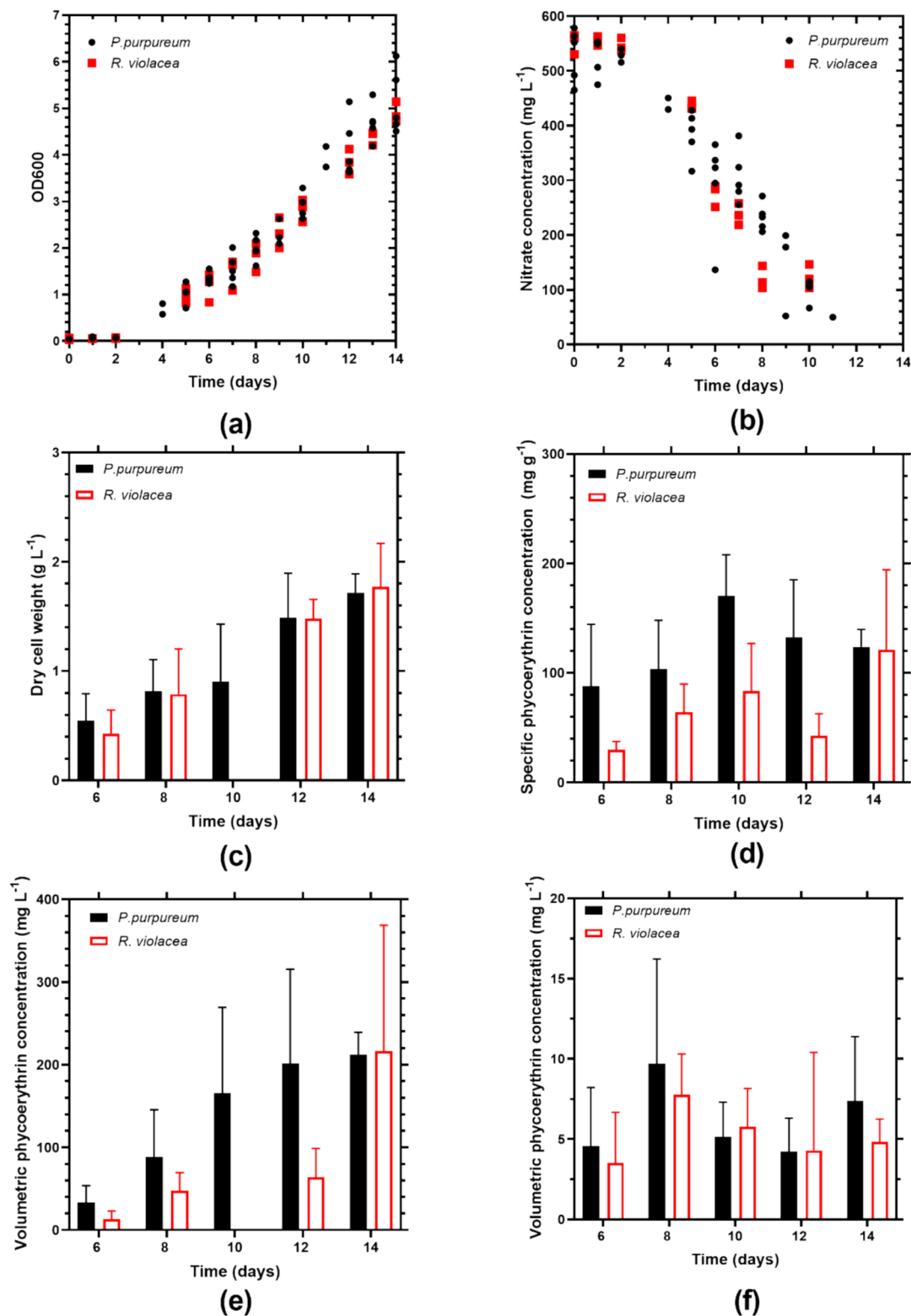
Fig. 4 Results from experiments in PBRs using increased lighting ( 450 \mu\text{mol photons m}^{-2} \text{s}^{-1} ) and 5f medium. Panel (a) shows the optical density at 600 nm, panel (b) shows the nitrate concentration, panel (c) shows the dry cell weight, panel (d) shows the specific phycoerythrin concentration, panel (e) shows the volumetric phycoerythrin concentration and panel (f) shows the same data for
