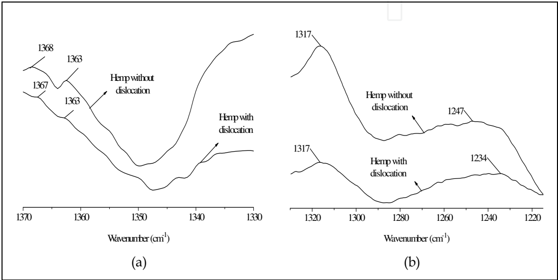
Fig. 11. FTIR spectra of hemp fibres from 1370 cm -1 to 1330 cm -1 (a) and from 1330 cm -1 to 1215 cm -1 (b) with and without dislocation [32]
