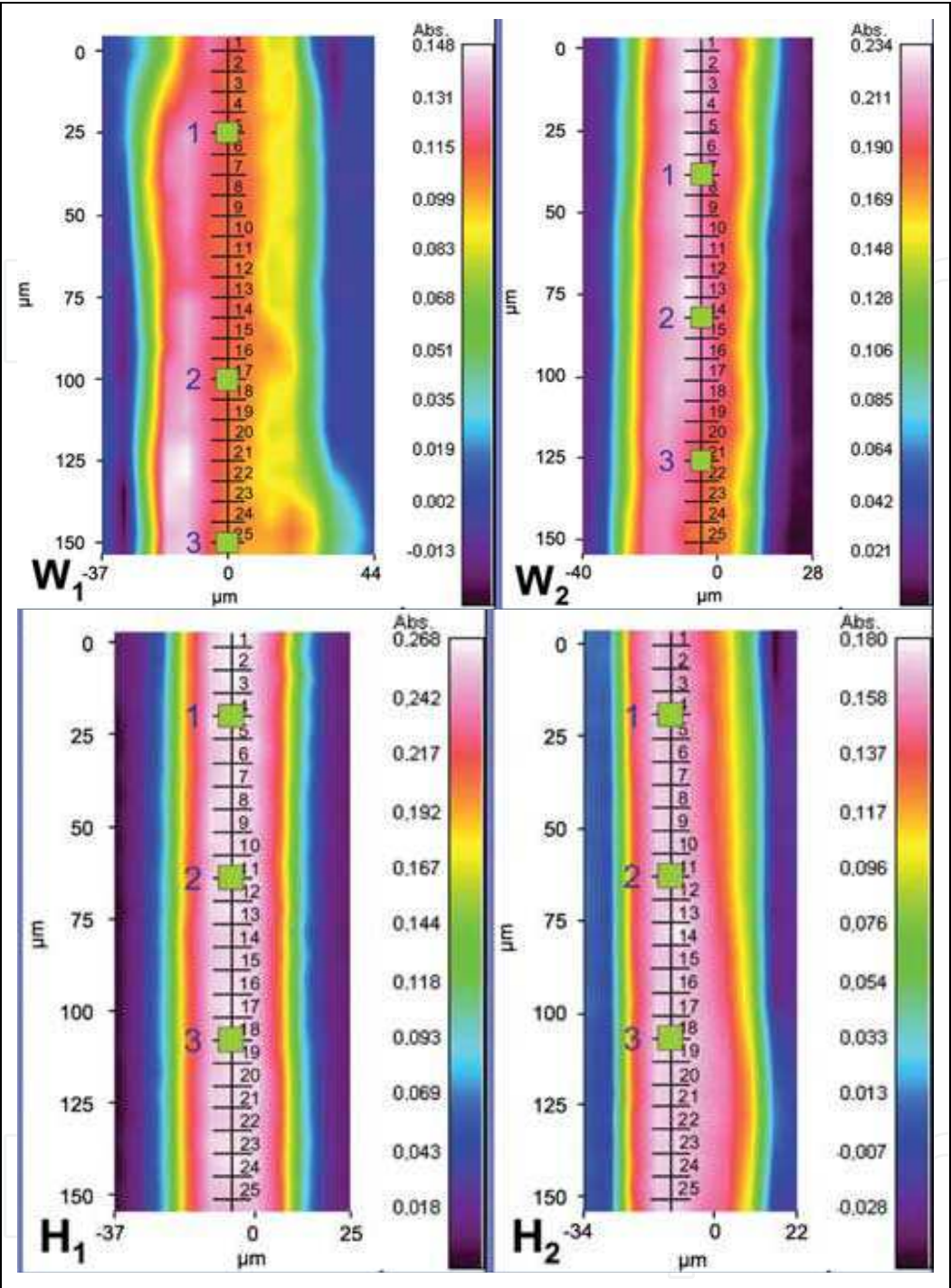
Fig. 17. Total IR absorbance full-spectral images of the two W fibres ( W 1 and W 2) and the two H fibres ( H 1 and H 2), showing the 25 pixel positions for each fibre used for evaluating the average orientation spectra as well as the three pixel positions for each fibre selected for evaluating the orientation of the different wood polymers in the fibres [86]
