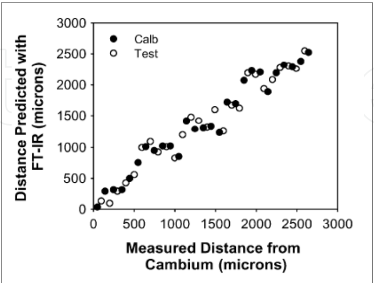
Fig. 16. PLS model predicting the distance from the bark to pith based on changes in the chemical composition. (Filled circles=calibration and open circles =test set) [85]
