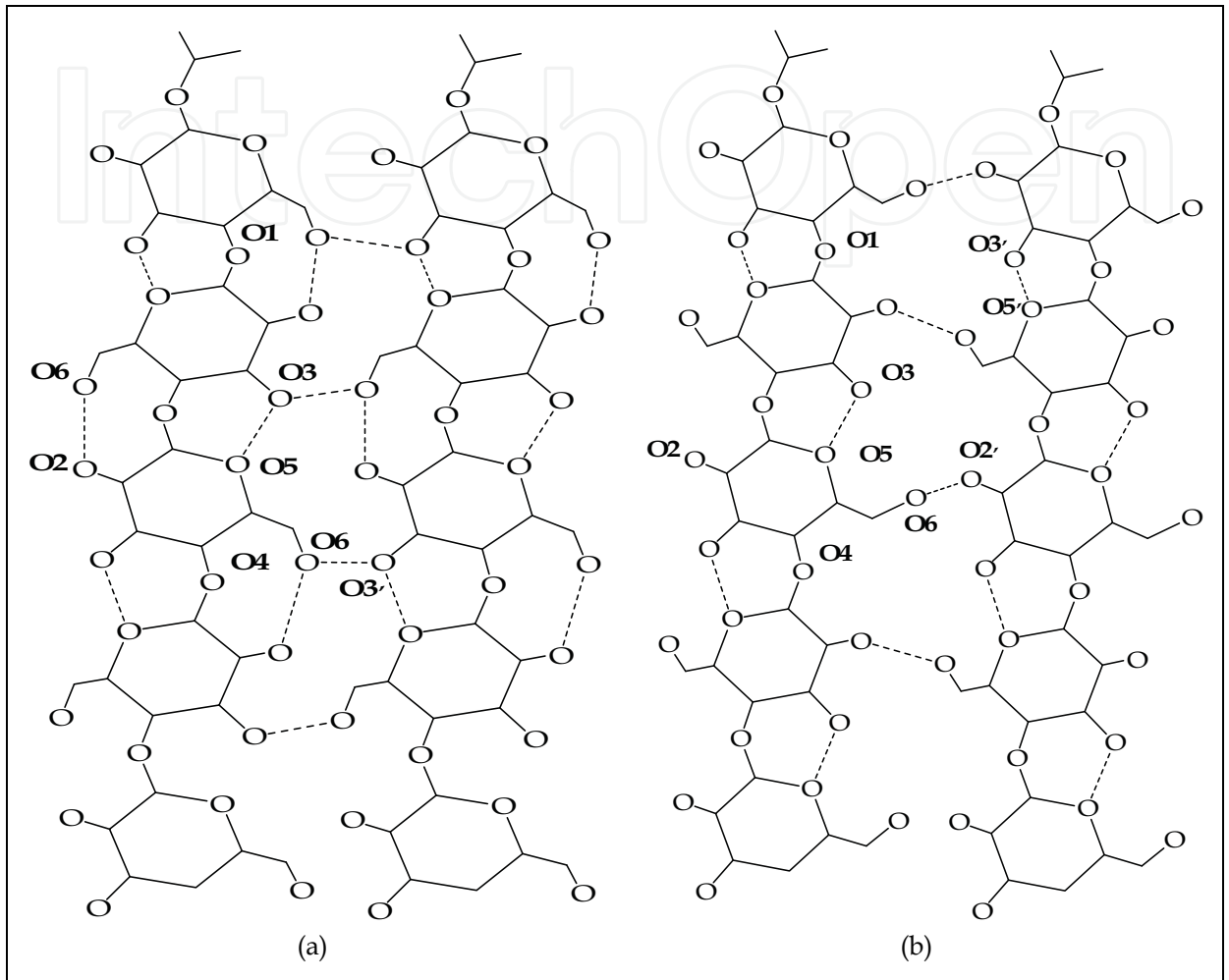
Fig. 9. Hydrogen-bonding network: (a) parallel to the bc plane (cellulose I); (b) in the centre chains (Cellulose II)
