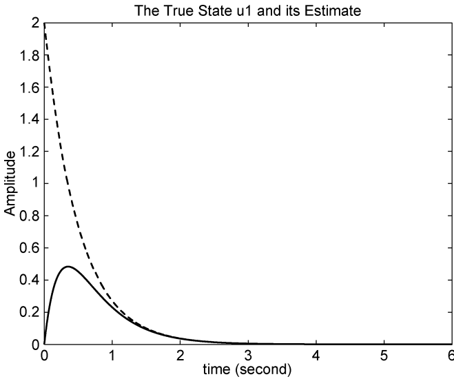
Fig. 2. u_1 (dashed), \hat{u}_1 (solid).
