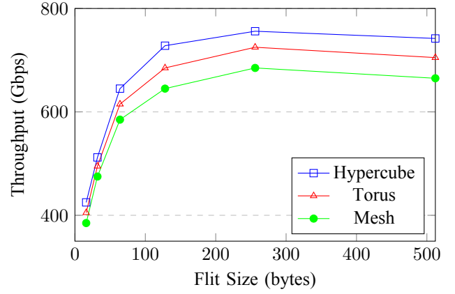
Fig. 5. Flit size vs Throughput correlation analysis across topologies (correlation coefficient: 0.892)
