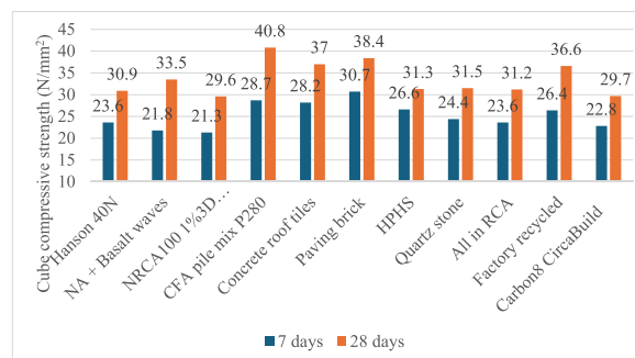
Fig. 2.21. Third-generation recycled aggregate compressive strength.
