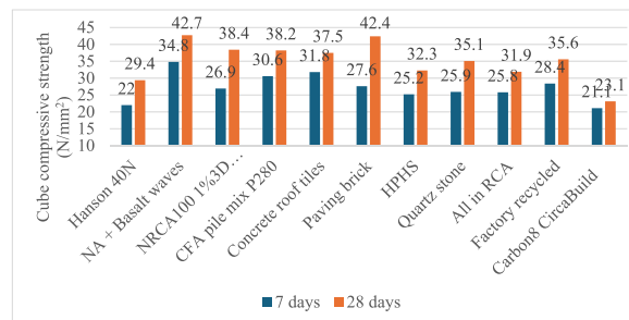
Fig. 2.20. Second-generation recycled aggregate compressive strength.
