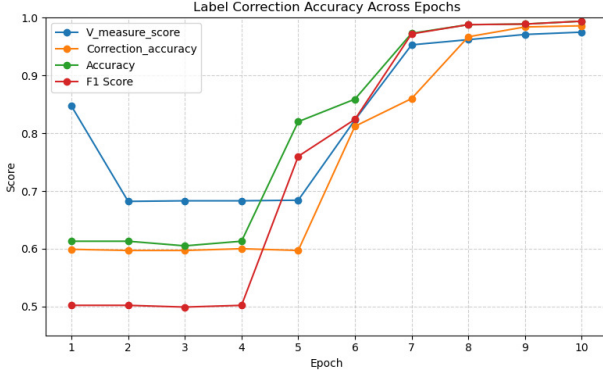
Fig. 7. The label correction performance across epochs under 70% symmetric noise.
