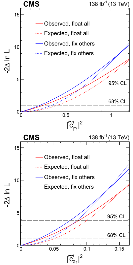
FIG. 8. Constraints on the square of |c_{\gamma\gamma}| (or |\tilde{c}_{\gamma\gamma}| ) and |c_{z\gamma}| (or |\tilde{c}_{z\gamma}| ) from the combination of the H \rightarrow b\bar{b} and 4\ell channels. The other couplings are either fixed to the null SM expectation (blue) or are left floating in the fit (red). Observed (solid) and expected (dashed) likelihood scans are shown. The dashed horizontal lines show the 68% and 95% CL intervals.
