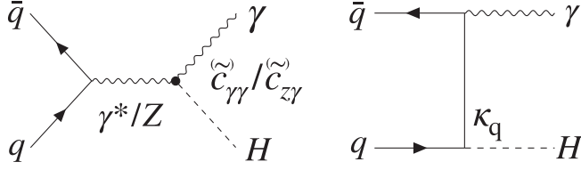
FIG. 1. Examples of Feynman diagrams illustrating \gamma H production at the LHC, highlighting the relevant couplings as discussed in the text. Left: production occurs via an effective loop-generated H\gamma\gamma or HZ\gamma interaction, denoted by a dot, which is the primary focus of this paper. Right: production proceeds through H boson production in q\bar{q} annihilation with photon radiation.
