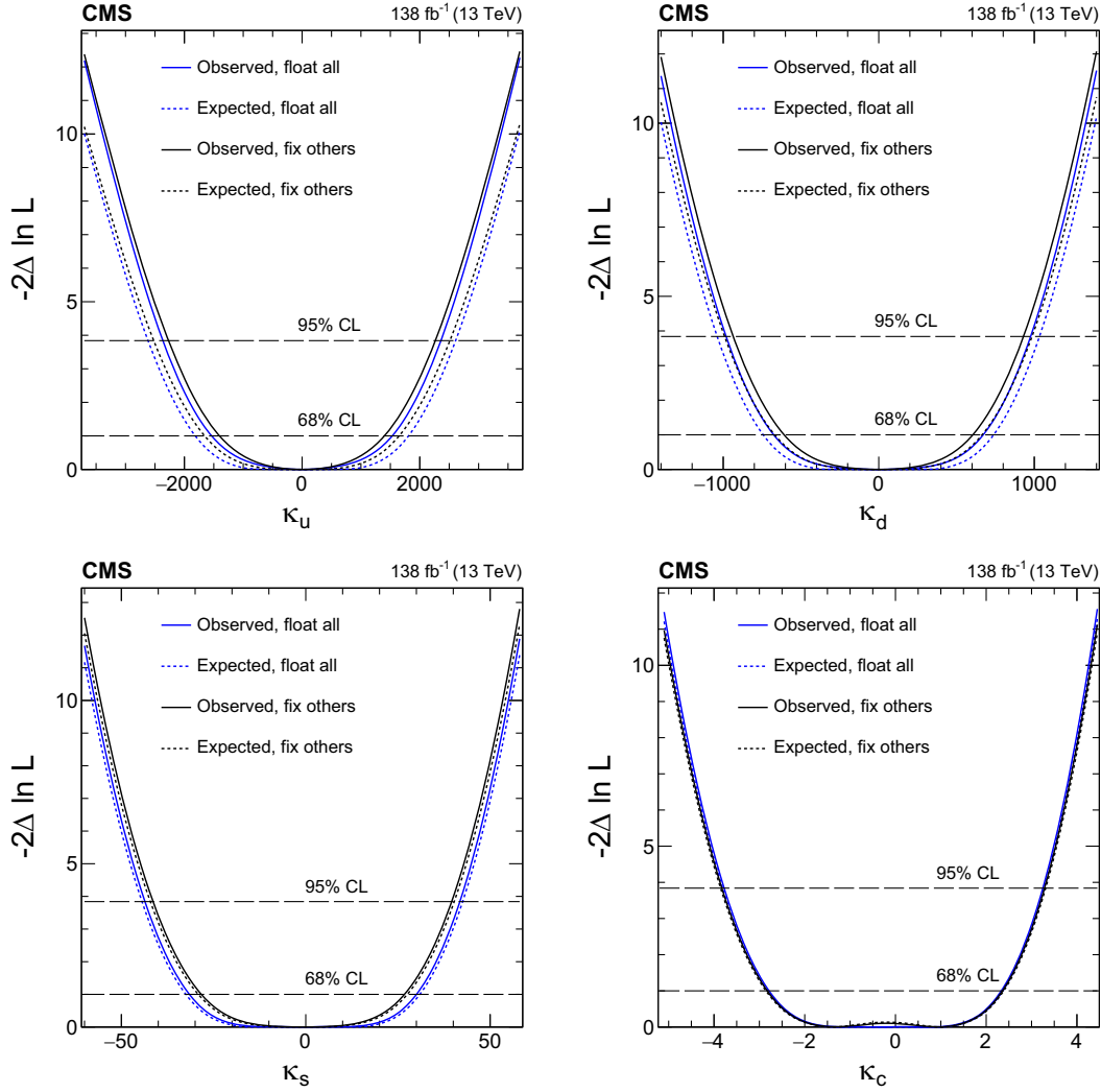
FIG. 9. Constraints on \kappa_u , \kappa_d , \kappa_s , and \kappa_c are shown using the H \rightarrow 4\ell channel. In scenario one (black), all couplings except the one being shown are fixed at their SM values. In scenario two (blue), the Yukawa couplings for the three other light quarks are left unconstrained, and BSM contributions are allowed: \kappa_{ZZ}^2 \leq 1 and \Gamma_H^{\text{BSM}} \geq 0 . Both observed (solid) and expected (dashed) constraints are presented. The crossings of dashed horizontal lines and the likelihood curves indicate the 68% and 95% CL intervals.
