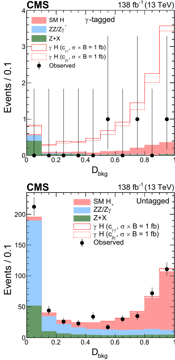
FIG. 5. Distributions of events for the D_{\text{bkg}} observable in the \gamma -tagged (upper) and Untagged (lower) categories of the H \rightarrow 4\ell candidate events. Observed events (black markers) and expected background estimates (solid histograms) from MC simulation ( ZZ/Z\gamma^* ) or control samples in data ( Z + X ) are shown. The \gamma H signal contribution, stacked on top of background, is shown with an open histogram for an assumed cross section of \sigma_{\gamma H} \mathcal{B}_{4\ell} = 1 fb for either the c_{\gamma\gamma} (solid) and c_{z\gamma} (dashed) coupling hypothesis.
