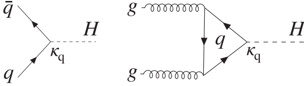
FIG. 4. Feynman diagrams describing the H boson production at LHC through direct q\bar{q} annihilation (left) and gluon fusion production (right).
