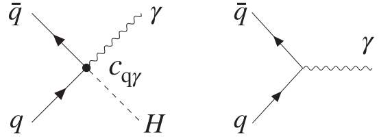
FIG. 3. Feynman diagrams describing the q\bar{q} annihilation with production of \gamma H through a pointlike EFT operator (left) and with photon production (right).
