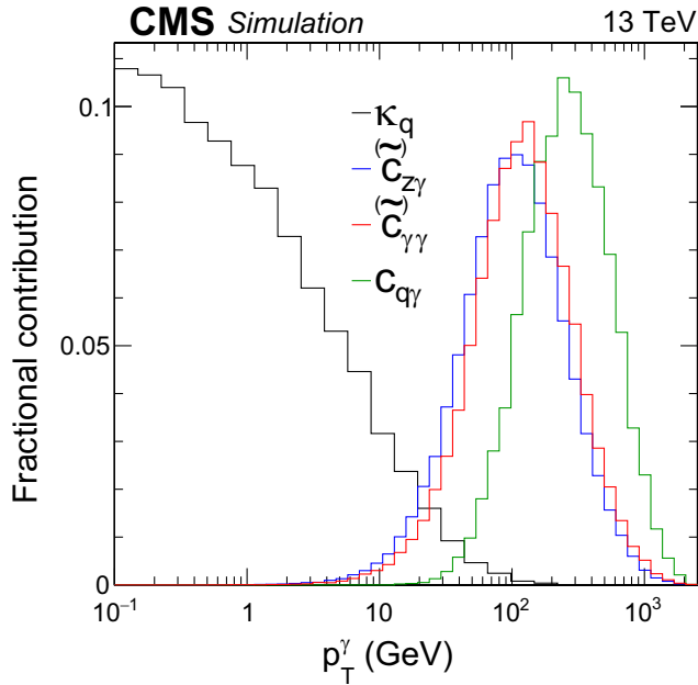
FIG. 2. Spectrum of the photon transverse momentum in \gamma H production, as generated by the leading-order diagrams shown in Figs. 1 and 3. The four distributions correspond to production resulting from couplings \kappa_q , c_{z\gamma} ( \tilde{c}_{z\gamma} ), c_{\gamma\gamma} ( \tilde{c}_{\gamma\gamma} ), and c_{q\gamma} .
