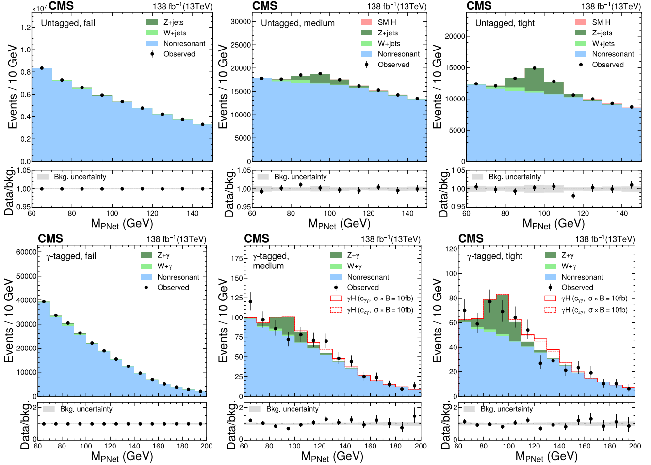
FIG. 6. M_{\text{PNet}} distributions for the number of observed events (black markers) compared with the backgrounds estimated in the fit to the data (filled histograms) in the b\bar{b} channel. Fail (left), medium (middle) and tight (right) regions of the \gamma -tagged (lower) and Untagged (upper) categories are shown. The signal contribution, stacked on top of background, is shown with an open histogram for an assumed cross section of \sigma_{\gamma H} \mathcal{B}_{b\bar{b}} = 10 fb.
