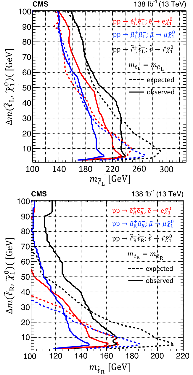
FIG. 33. Slepton pair production. Observed 95% CL exclusion regions for direct pair production of the superpartners of the left-handed leptons (upper) and direct pair production of the superpartners of the right-handed leptons (lower) followed by decay of both sleptons to the corresponding lepton and neutralino with 100% branching fraction. The limits are shown as a function of the slepton mass and the mass difference between the slepton and the lightest neutralino. The regions to the left of the lines denote the excluded regions. Median expected limits are displayed with dashed lines.
