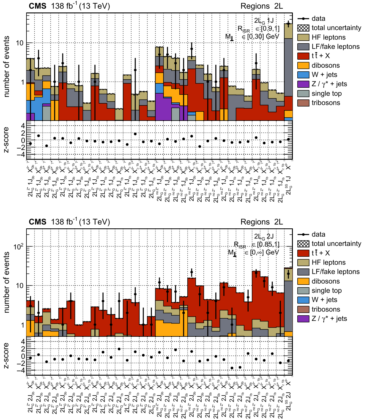
FIG. 24. Postfit distributions of data with the background-only model for the full dataset for the highest R_{\text{ISR}} bin in each analysis category. (Upper) 2L 1J regions with gold leptons. (Lower) 2L \geq 2 J regions with gold leptons. The subpanels below the panels indicate the postfit z-score for each bin.
