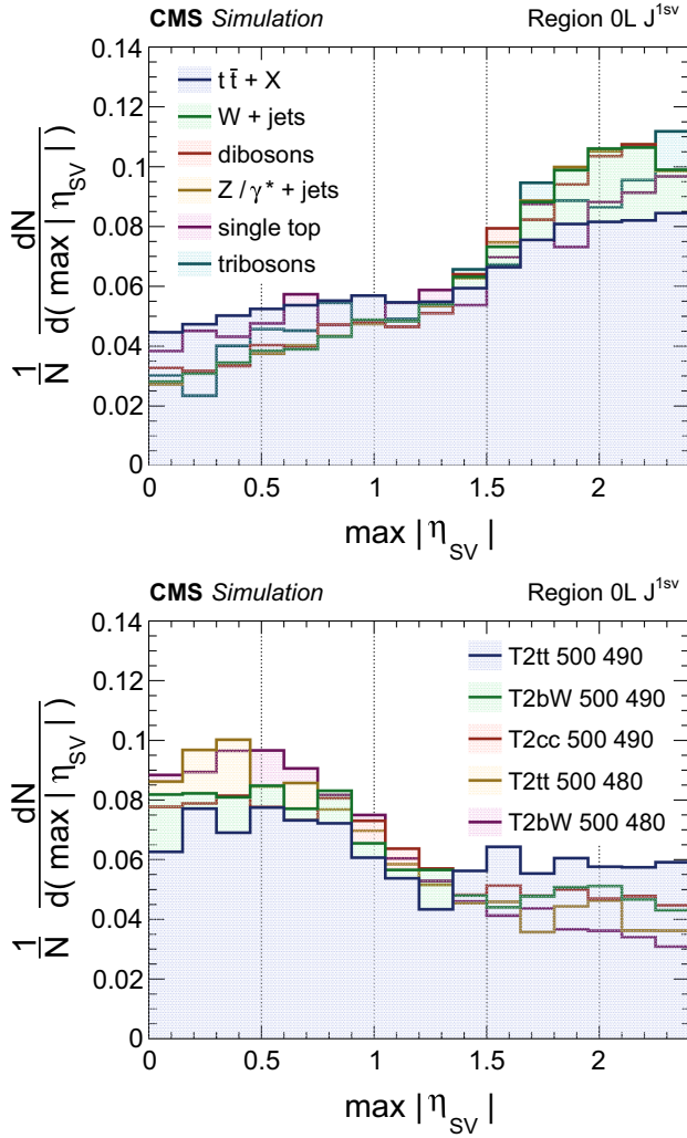
FIG. 13. Distributions of \max |\eta_{SV}^S| in final states with 0 leptons and \geq 1 SVs associated with the S system, for simulated SM background events (upper) and various top squark signal models (lower).
