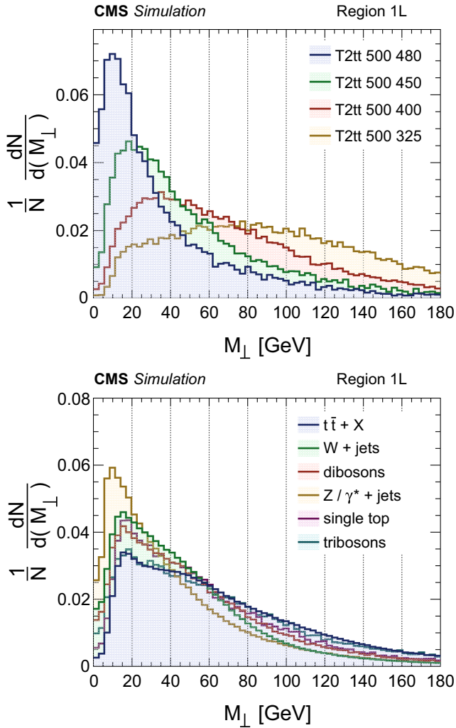
FIG. 11. Distributions of M_\perp in one lepton final states for simulated events: compressed T2tt signal events with a parent top squark mass of 500 GeV and LSP masses ranging from 325 to 480 GeV (upper) and the SM backgrounds (lower).
