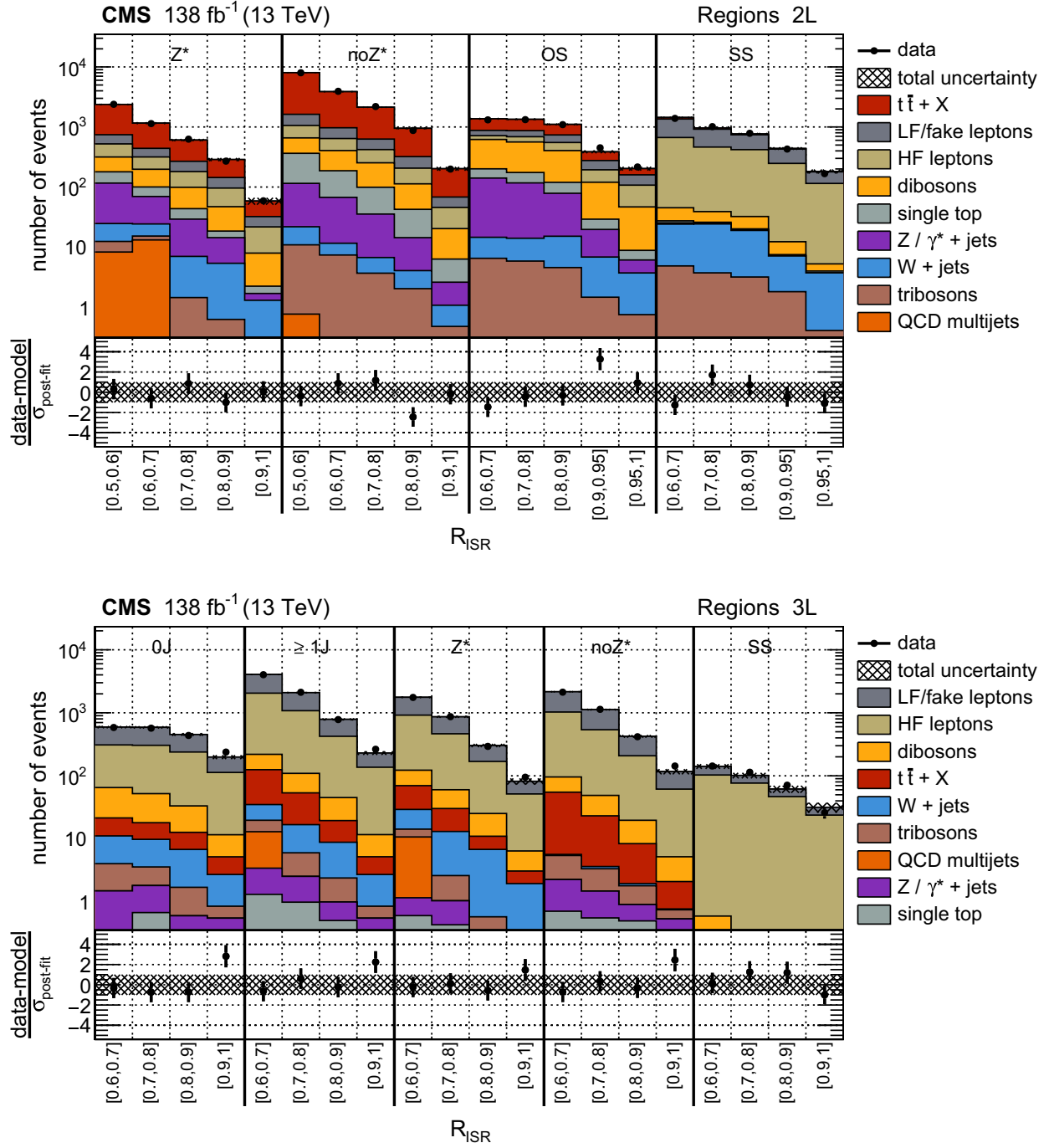
FIG. 17. Postfit distributions of data with the background-only fit model for the full dataset in the 2L region (upper) and 3L region (lower). Bins are split by R_{\text{ISR}} along with lepton categorization. Yields are integrated over all other subcategorizations and M_{\perp} . The subpanels below the panels show the data minus fit model scaled by the postfit model uncertainty. This uncertainty neglects correlations among the individual fitted bin event yields.
