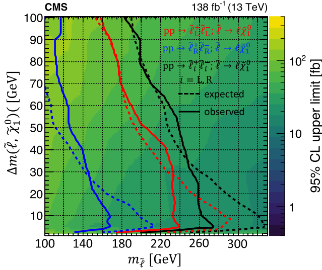
FIG. 30. Slepton pair production. Observed 95% CL upper limits on the product of the cross section and branching fraction squared for direct slepton pair production followed by decay of both sleptons to the corresponding lepton and neutralino (color scale). Slepton \tilde{\ell}_{L/R} indicates the scalar supersymmetric partner of left- and right-handed electrons and muons. The limit is shown as a function of the slepton mass and the mass difference between the slepton and the lightest neutralino. The regions to the left of the lines denote the regions excluded for a branching fraction of 100%. The median expected exclusion regions for 100% branching fraction are delimited by the dashed lines.
