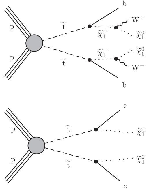
FIG. 2. Diagrams for top squark pair production. The upper panel shows the T2bW model with decay via an intermediate mass chargino and the lower panel shows the T2cc model with decay via charm quarks.
