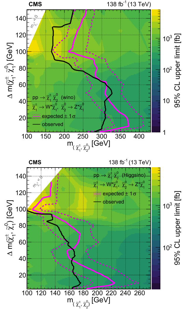
FIG. 27. Chargino-neutralino production. Observed upper limits at 95% CL on the product of the cross section and the two branching fractions, \sigma(\tilde{\chi}_1^\pm \tilde{\chi}_2^0) \mathcal{B}(\tilde{\chi}_1^\pm \rightarrow W^\pm \tilde{\chi}_1^0) \mathcal{B}(\tilde{\chi}_2^0 \rightarrow Z \tilde{\chi}_1^0) , are shown using the color scale where the \tilde{\chi}_1^\pm/\tilde{\chi}_2^0 mass is on the x axis and the mass difference between the \tilde{\chi}_1^\pm/\tilde{\chi}_2^0 and the LSP is on the y axis. For these results, based on the TChiWZ simplified model, the \tilde{\chi}_1^\pm and \tilde{\chi}_2^0 masses are set equal. The expected lower mass limits (magenta line) together with their \pm 1\sigma uncertainties (magenta dashed lines) and the observed lower mass limits (black line) are indicated for 100% branching fractions for wino-like cross sections (upper) and for Higgsino-like cross sections (lower).
