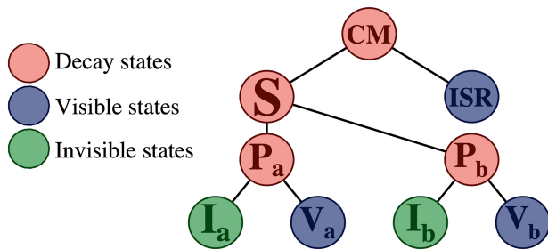
FIG. 8. Decay tree diagram used to analyze events. Here S represents the total system of candidate sparticles, with \mathbf{P}_{a/b} representing pair-produced SUSY parent particles; \mathbf{I}_{a/b} and \mathbf{V}_{a/b} represent the systems of invisible and visible sparticle decay products, respectively. The S system, along with the recoiling ISR system, are viewed as decay products of the entire CM system of the colliding partons with constituent center-of-mass energy, \sqrt{s} .
