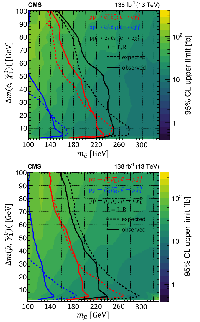
FIG. 31. Slepton pair production. Observed 95% CL upper limits on the cross section times branching fraction squared for direct selectron pair production (upper) and smuon pair production (lower) followed by decay of both sleptons to the corresponding lepton and neutralino (color scale). The limits are shown as a function of the slepton mass and the mass difference between the slepton and the lightest neutralino for the three different simplified possibilities of only RR, only LL, and both RR and LL where it is assumed that the R and L masses are identical. The regions to the left of the lines denote the regions excluded for a branching fraction of 100%. Median expected limits for 100% branching fraction are delimited by the dashed lines.
