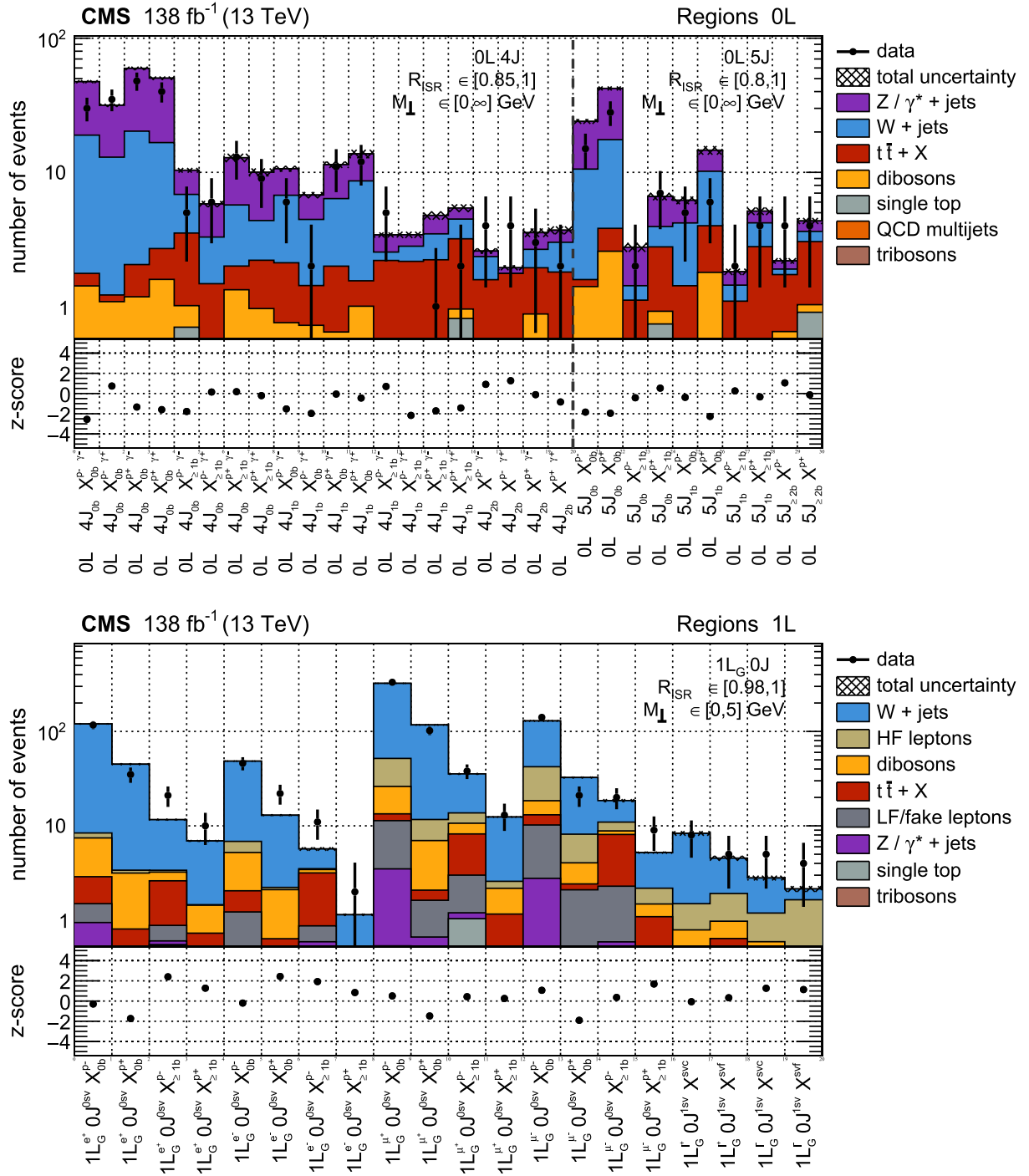
FIG. 21. Post fit distributions of data with the background-only model for the full dataset for the highest R_{\text{ISR}} bin in each analysis category. (Upper) 0L 4J and \geq 5 J regions. (Lower) 1L 0J regions with a gold lepton. The subpanels below the panels indicate the postfit z-score for each bin.
