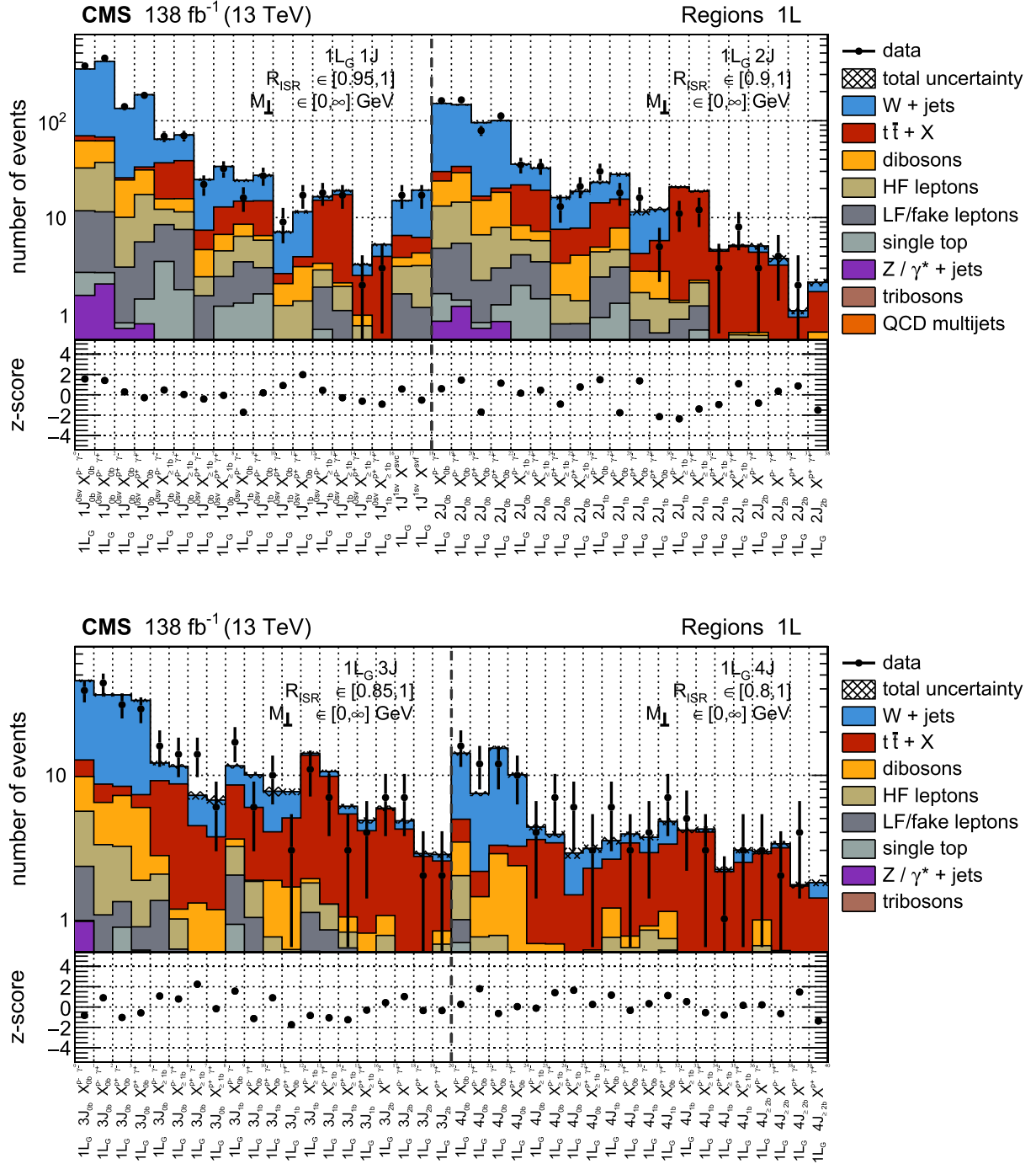
FIG. 22. Postfit distributions of data with the background-only model for the full dataset for the highest R_{\text{ISR}} bin in each analysis category. (Upper) 1L 1J and 2J regions with a gold lepton. (Lower) 1L 3J and \geq 4 J regions with a gold lepton. The subpanels below the panels indicate the postfit z-score for each bin.
