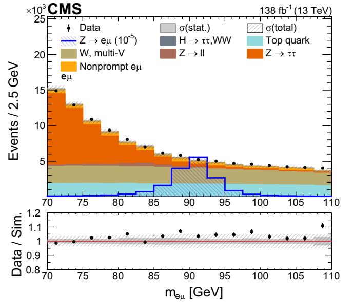
FIG. 1. Invariant mass of the e\mu system for data (points, with bars denoting statistical uncertainty) and simulated background (stacked filled histograms) for events passing the baseline selection. In the legend, “W, multi-V” refers to W + jets events having a jet that is misidentified as a lepton, together with multiple vector boson production. The hatched histogram shows a hypothetical Z \rightarrow e\mu signal normalized to a branching fraction of 10^{-5} . The lower panel shows the ratio of the data to simulated background yields, with the statistical (combined systematic and statistical) uncertainty in the simulated yield indicated by the filled (hatched) gray band.
