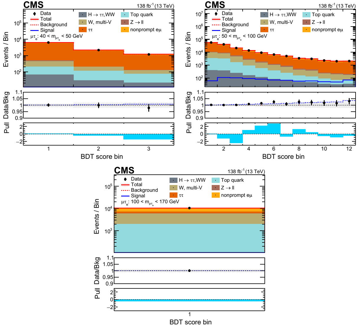
FIG. 12. Transformed BDT score distributions for the Z \rightarrow \mu\tau_e channels in the m_{\mu\tau} ranges: (upper left) 40–50 GeV, “ \tau\tau ”; (upper right) 50–100 GeV, “signal-like”; (lower) 100–170 GeV, “misID”. In each plot, the upper panel shows the data (points), the total yield from the signal + background fit (red open histogram), the signal component (blue open histogram), and the background components (stacked filled histograms). The middle panel shows the ratio to the background of the data (points with bars showing the statistical uncertainty in the data) and the combined signal + background (blue dotted histogram). The shaded band shows the systematic uncertainty in the background estimate. The lower panel shows the pull defined in the text (light-blue filled histogram).
