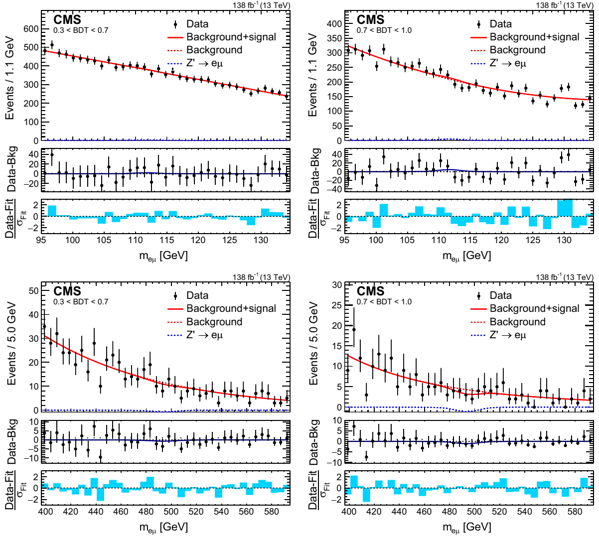
FIG. 14. Distributions in m_{e\mu} for the scan points 111 GeV (upper row) and 496 GeV (lower row) from the Z' search. In each row the BDT score range for the left (right) plot is 0.3–0.7 (0.7–1.0). In each plot, the upper panel shows the data (points with bars showing the statistical uncertainty) together with the fit distribution curve (red solid) and its separate signal (blue dotted) and background (red dotted) components, the middle panel shows the background subtracted data with the fit signal distribution, and the lower panel shows the deviations of the data from the fit function divided by the fit uncertainty.
