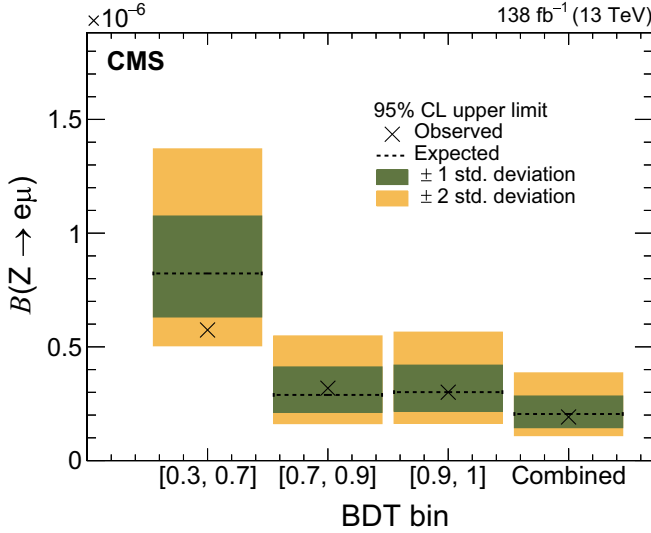
FIG. 8. Upper limits at 95% CL on the branching fraction B(Z \rightarrow e\mu) , for each BDT score range and for the final combined fit. The observed limits are denoted by the markers, while the expected limits with their 68% and 95% uncertainties are denoted by the horizontal dashed lines and green and yellow bands, respectively.
