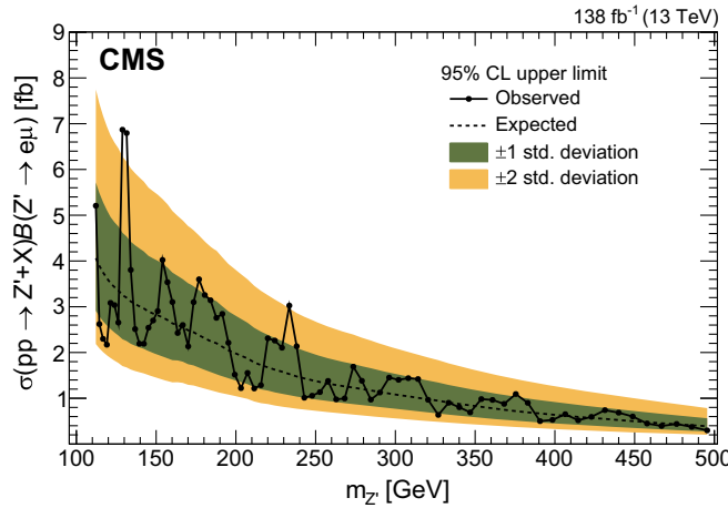
FIG. 15. Expected and observed 95% CL upper limits on \sigma(pp \rightarrow Z' + X)\mathcal{B}(Z' \rightarrow e\mu) for Z' masses between 110 and 500 GeV. The solid black line connects filled circles representing the observed upper limits at the scan points, and the dashed line with filled error bands shows the expected limit.
