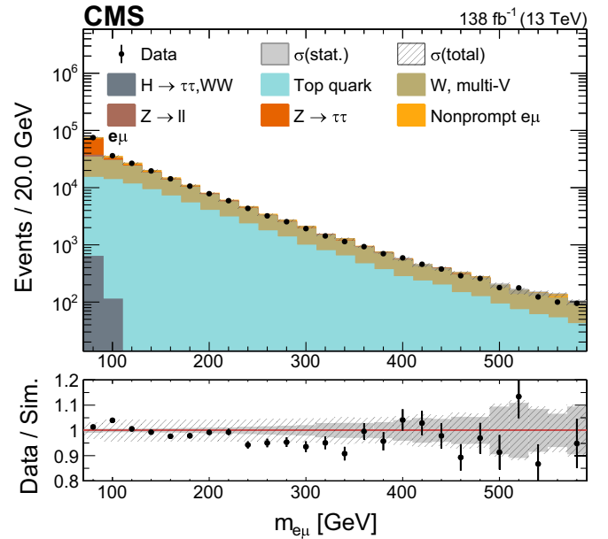
FIG. 4. Invariant mass of the e\mu system for data (points) and simulated background (stacked filled histograms), for events that pass the baseline selection except for that selection’s upper limit on the invariant mass. The lower panel shows the ratio of the data to simulated yields, with the statistical (combined systematic and statistical) uncertainty in the simulated yield indicated by the filled (hatched) gray band.
