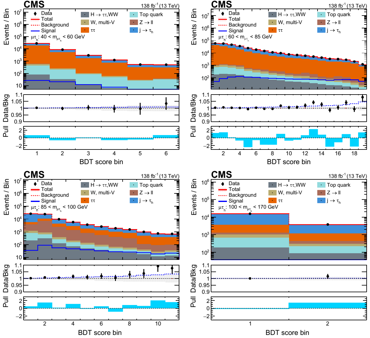
FIG. 11. Transformed BDT score distributions for the Z \rightarrow \mu\tau_h channels in the m_{\mu\tau} ranges: (upper left) 40–60 GeV, “ \tau\tau ”; (upper right) 60–85 GeV, “signal-like”; (lower left) 85–100 GeV, “ Z \rightarrow \ell\ell ”; (lower right) 100–170 GeV, “misID.” In each plot, the upper panel shows the data (points), the total yield from the signal + background fit (red open histogram), the signal component (blue open histogram), and the background components (stacked filled histograms). The middle panel shows the ratio to the background of the data (points with bars showing the statistical uncertainty in the data) and the combined signal + background (blue dotted histogram). The shaded band shows the systematic uncertainty in the background estimate. The lower panel shows the pull defined in the text (light-blue filled histogram).
