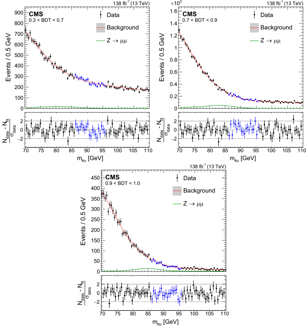
FIG. 3. Fits of the data sidebands with the background functions for the BDT score ranges 0.3–0.7 (upper left), 0.7–0.9 (upper right), and 0.9–1.0 (lower). In the upper panel of each plot, the black (blue) points with bars show the data with statistical uncertainties in the sideband (signal) region, the solid red line shows the average background prediction, and the green curve shows the Z \rightarrow \mu\mu^* \rightarrow \mu\mu\gamma background component. The lower panel in each plot shows the ratio of the difference between the data and the average background prediction to the uncertainty in the data, and the gray band shows the spread of the background estimates from the separate families of parametric functions.
