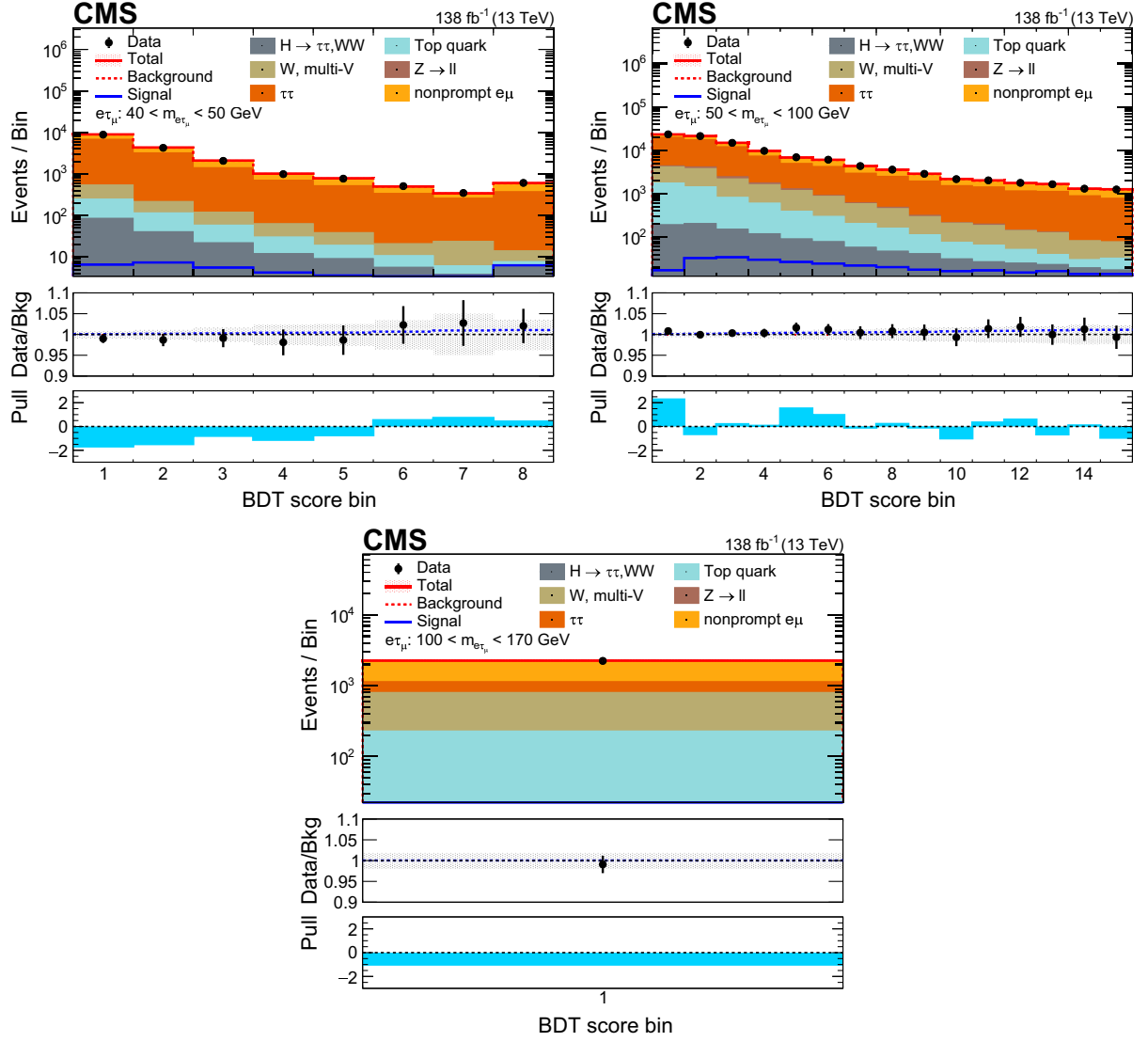
FIG. 10. Transformed BDT score distributions for the Z \rightarrow e\tau_\mu channels in the m_{e\tau} ranges: (upper left) 40–50 GeV, “ \tau\tau ”; (upper right) 50–100 GeV, “signal-like”; (lower) 100–170 GeV, “misID.” In each plot, the upper panel shows the data (points), the total yield from the signal + background fit (red open histogram), the signal component (blue open histogram), and the background components (stacked filled histograms). The middle panel shows the ratio to the background of the data (points with bars showing the statistical uncertainty in the data) and the combined signal + background (blue dotted histogram). The shaded band shows the systematic uncertainty in the background estimate. The lower panel shows the pull defined in the text (light-blue filled histogram).
