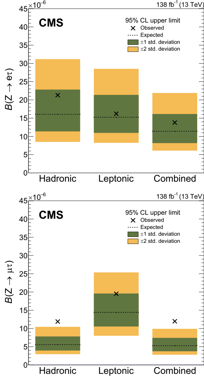
FIG. 13. Observed and expected 95% CL upper limit by category, as well as for the final combined fit, for the Z \rightarrow e\tau (upper) and Z \rightarrow \mu\tau (lower) searches. The observed limits are denoted by the markers, while the expected limits with their 68% and 95% uncertainties are denoted by the horizontal dashed lines and green and yellow bands, respectively.
