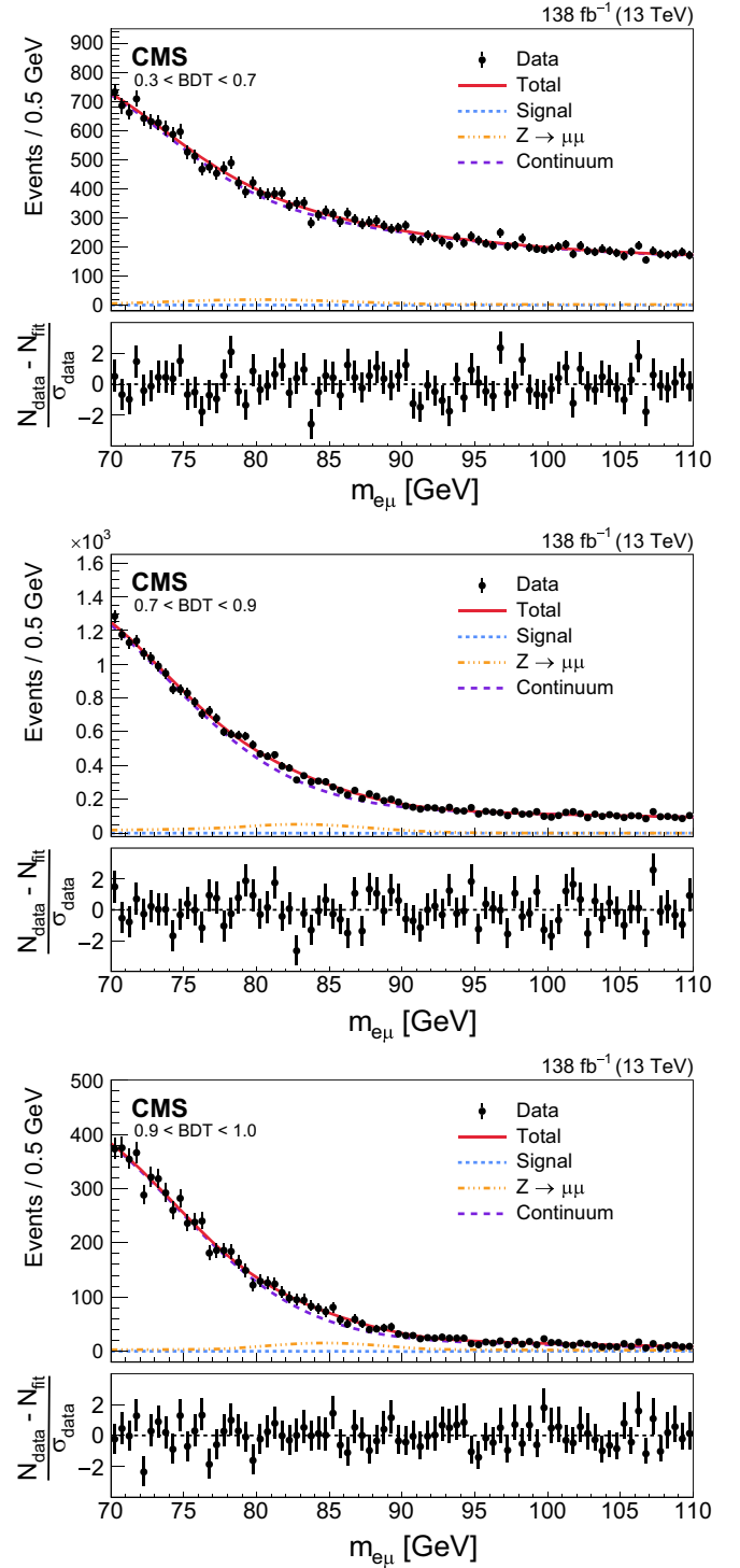
FIG. 7. For the Z \rightarrow e\mu search, the invariant mass fit results for the BDT score ranges 0.3–0.7 (upper), 0.7–0.9 (middle), and 0.9–1.0 (lower). In each plot, the upper panel shows the data (points with bars showing the statistical uncertainties) together with the fit distribution curve (red) and its separate signal (blue dotted) Z \rightarrow \mu\mu (yellow dash-dotted) and continuum background (purple dashed) components, and the lower panel shows the deviations of the data from the fit function divided by the data uncertainty.
