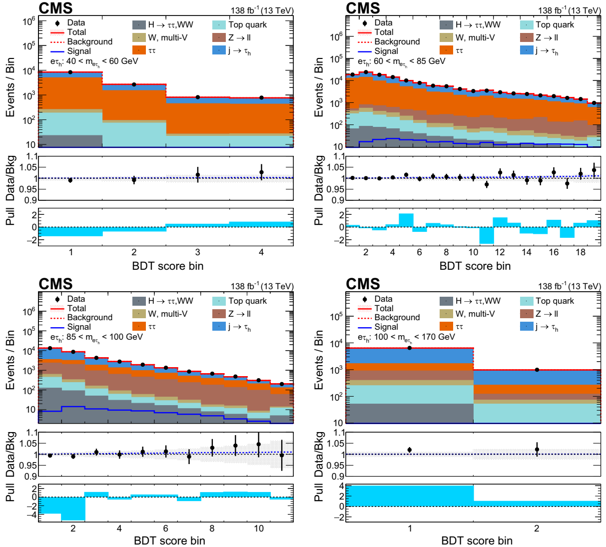
FIG. 9. Transformed BDT score distributions for the Z \rightarrow e\tau_h channels in the m_{e\tau} ranges: (upper left) 40–60 GeV, “ \tau\tau ”; (upper right) 60–85 GeV, “signal-like”; (lower left) 85–100 GeV, “ Z \rightarrow \ell\ell ”; (lower right) 100–170 GeV, “misID.” In each plot, the upper panel shows the data (points), the total yield from the signal + background fit (red open histogram), the signal component (blue open histogram), and the background components (stacked filled histograms). The middle panel shows the ratio to the background of the data (points with bars showing the statistical uncertainty in the data) and the combined signal + background (blue dotted histogram). The shaded band shows the systematic uncertainty in the background estimate. The lower panel shows the pull defined in the text (light-blue filled histogram).
