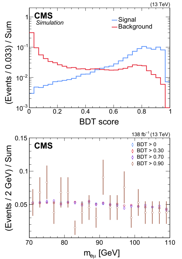
FIG. 2. The upper plot shows unity-normalized distributions of the Z \rightarrow e\mu BDT score for simulated events from the BDT test samples satisfying 70 < m_{e\mu} < 110 GeV. The blue and red histograms represent the signal and WW background, respectively. The lower plot displays the unity-normalized distribution of m_{e\mu} for events in the t\bar{t} data CR used to check for BDT mass-spectrum bias, for several BDT thresholds; the vertical bars show the statistical uncertainties.
