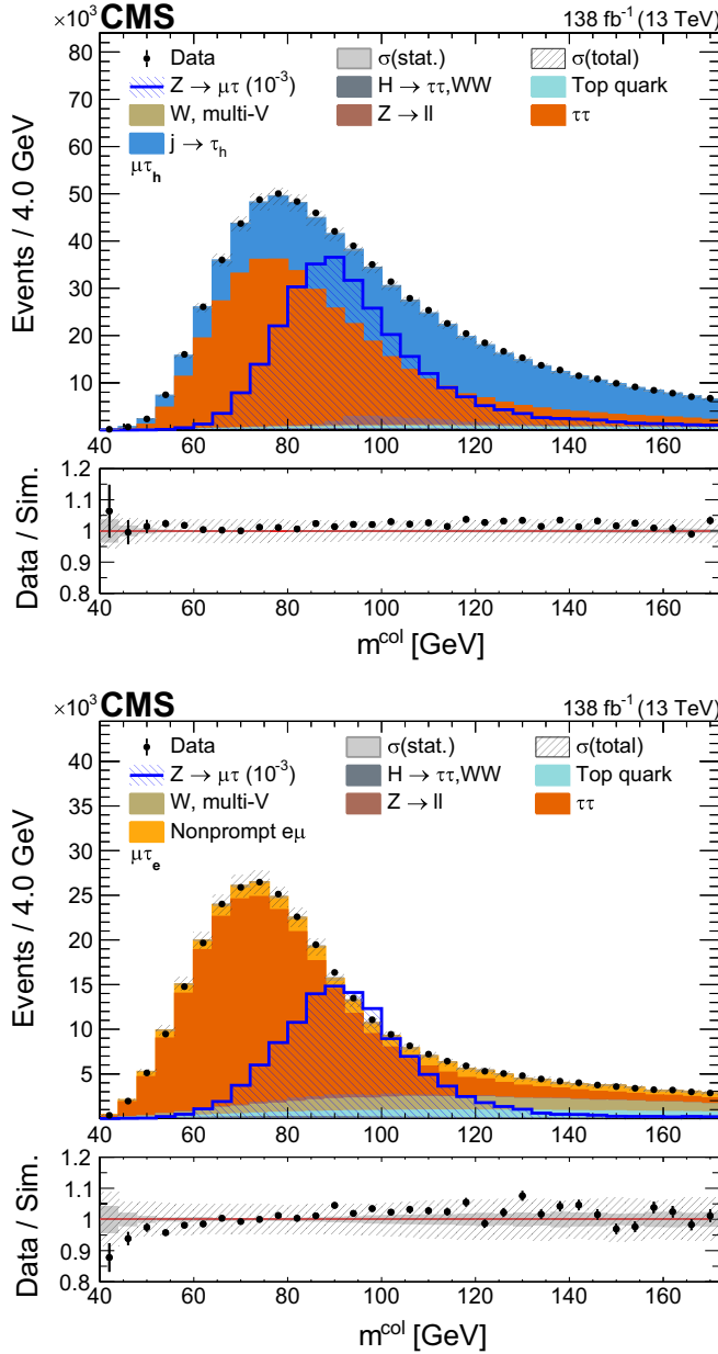
FIG. 5. The \mu\tau_h (upper) and \mu\tau_e (lower) m^{\text{col}} distributions, for the data (black markers with bars showing the statistical uncertainties) and the simulated backgrounds (filled stacked histograms). The hatched blue histogram shows the shape of the signal, normalized to a branching fraction of 10^{-3} , for comparison. The lower panel shows the ratio of the data to simulated yields, with the statistical (combined systematic and statistical) uncertainty in the simulated yield indicated by the filled (hatched) gray band.
