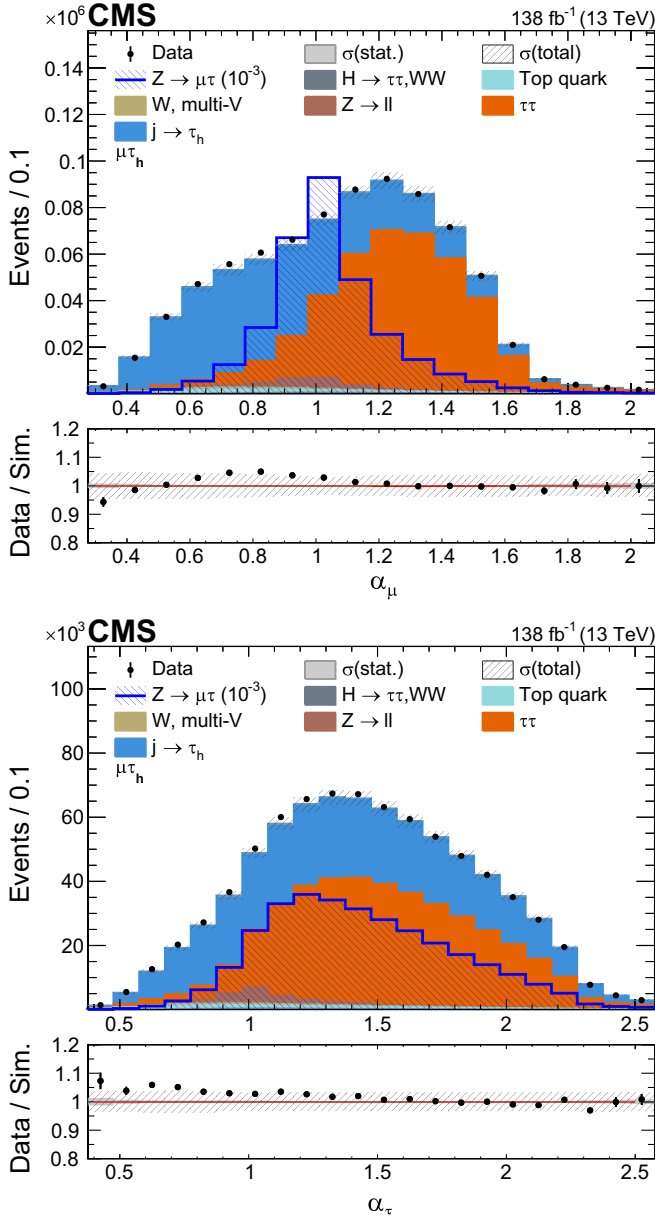
FIG. 6. Distributions of \mu\tau_h signal and estimated backgrounds in \alpha_\mu (upper), \alpha_\tau (lower), for the data (black markers with bars showing the statistical uncertainties) and the simulated backgrounds (filled stacked histograms). The hatched blue histogram shows the shape of the signal, normalized to a branching fraction of 10^{-3} , for comparison. The lower panel shows the ratio of the data to simulated yields, with the statistical (combined systematic and statistical) uncertainty in the simulated yield indicated by the filled (hatched) gray band.
