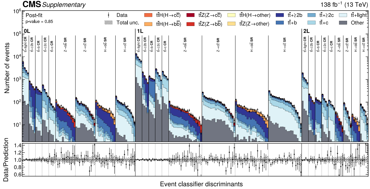
FIG. 6. Distributions of the ParT discriminants in data (points) and predicted signal and backgrounds (colored histograms) after the fit to data. The vertical bars on the points represent the statistical uncertainties in data. The hatched band represents the total uncertainty in the sum of the signal and background predictions. The lower panel shows the ratio of the data to the sum of the signal and background predictions.
