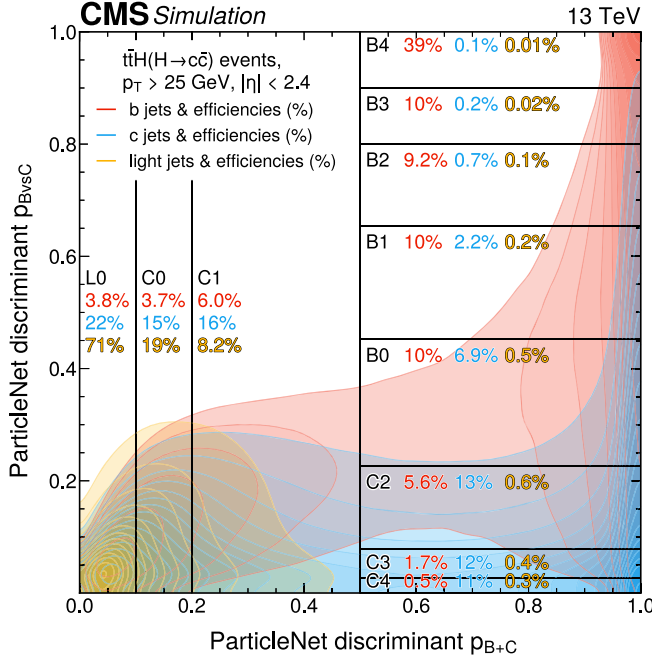
FIG. 1. Distribution of b , c , and light jets in the two-dimensional ParticleNet discriminant plane. The vertical and horizontal lines correspond to the edges of the tagging categories. The numbers in each bin correspond to the tagging efficiencies for b (red), c (blue), and light (yellow) jets, evaluated on a sample of simulated t\bar{t}H(H \rightarrow c\bar{c}) events. The contour lines represent constant density values for each jet type in steps of 5%.
