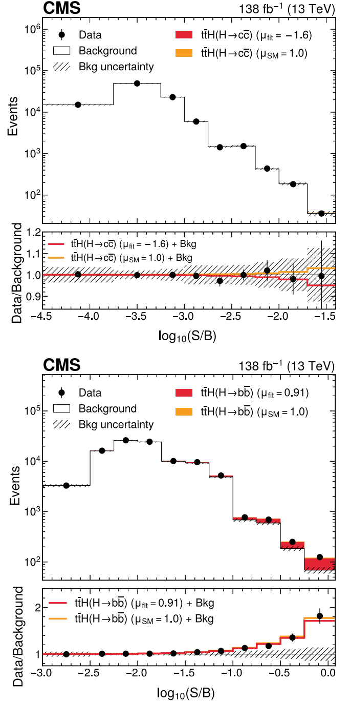
FIG. 2. Observed and expected event yields from all SRs and CRs as a function of \log_{10}(S/B) , where S are the expected t\bar{t}H(H \rightarrow c\bar{c}) (upper) and t\bar{t}H(H \rightarrow b\bar{b}) (lower) yields, and B are the post-fit total background yields. Signal contributions are shown for the best fit signal strength (red) and for the SM prediction, \mu = 1 (orange). The lower panel shows the ratio of the data to the post-fit background predictions, compared to the signal-plus-background predictions.
