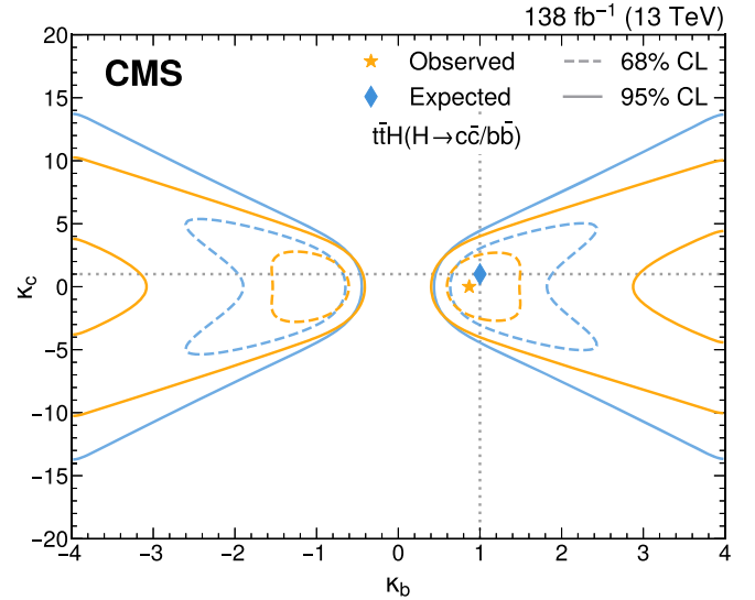
FIG. 4. Constraints on the Higgs boson coupling modifiers \kappa_c and \kappa_b . The 68% (95%) CL intervals are indicated by the dashed (solid) lines. The observed (expected) best fit values are shown by the orange (blue) markers.
