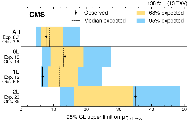
FIG. 3. The 95% CL upper limits on \mu_{t\bar{t}H(H\rightarrow c\bar{c})} . The yellow and blue bands indicate the expected 68% and 95% CL regions, respectively, under the background-only hypothesis. The vertical red line indicates the SM value \mu_{t\bar{t}H(H\rightarrow c\bar{c})} = 1 .
