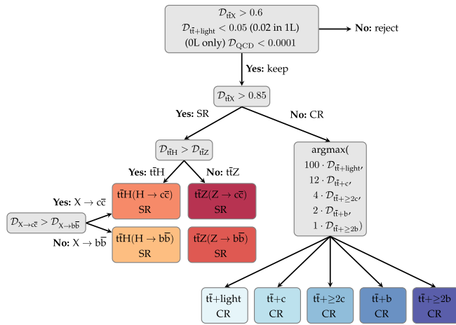
FIG. 5. Event categorization flowchart.
