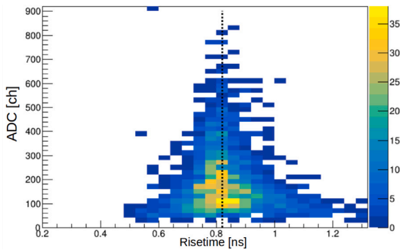
Fig. 5. For pad #6: Correlation distribution between signal rise-time and signal amplitude shown as ADC channels. The 17% larger rise-time is almost constant with the signal amplitude.
