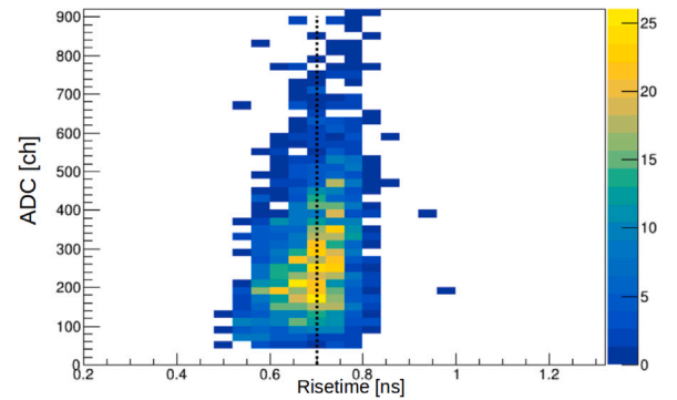
Fig. 4. For pad #5: Mild correlation between signal rise-time and signal amplitude shown as ADC channels. The good rise-time of 0.7 ns has slightly increased with the signal amplitude.
