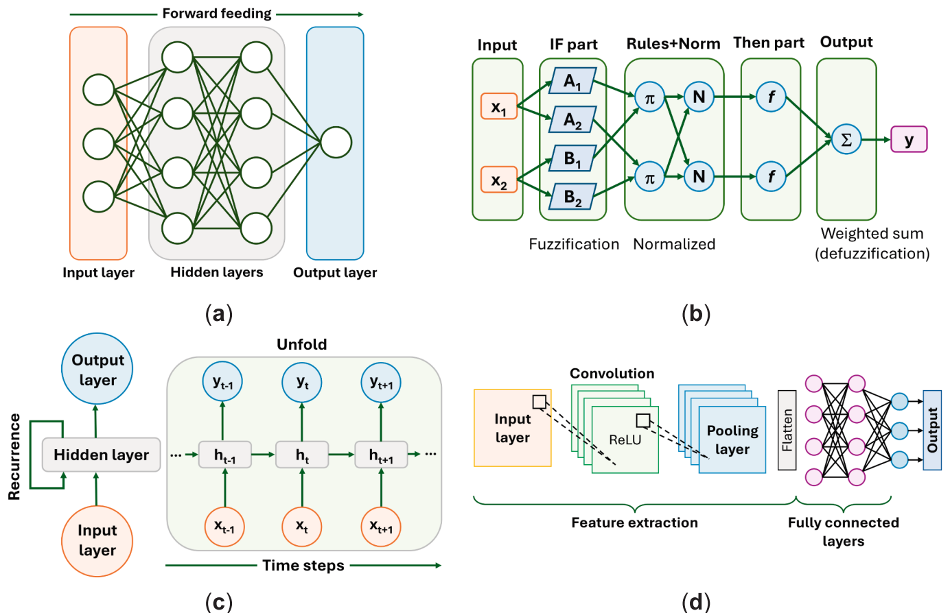
Fig. 8. Representative ANN models applied in PV/T systems: (a) FFNN; (b) ANFIS; (c) RNN; (d) CNN.
