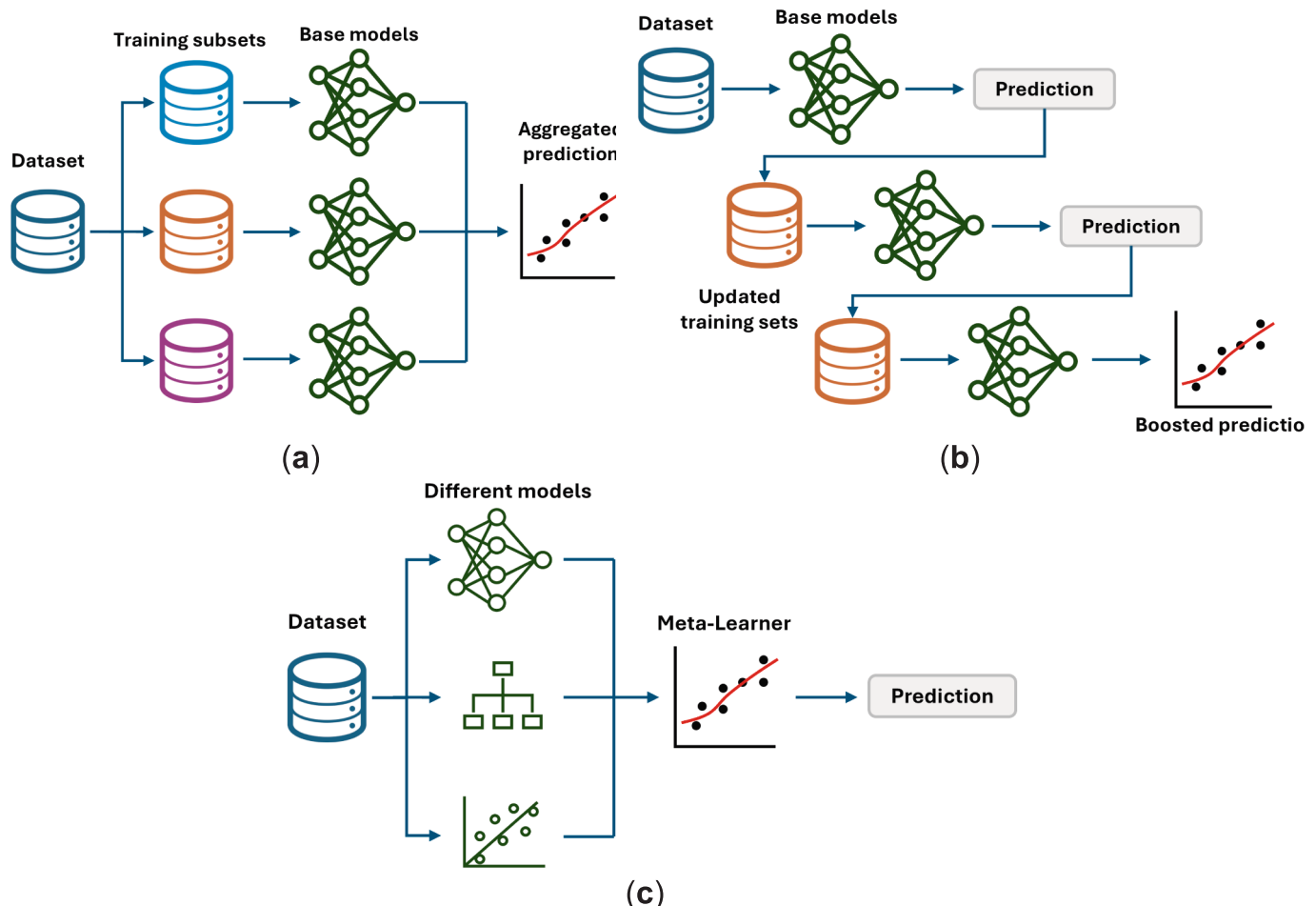
Fig. 10. Schematic representation of ensemble learning strategies: (a) Bagging; (b) Boosting; (c) Stacking.
