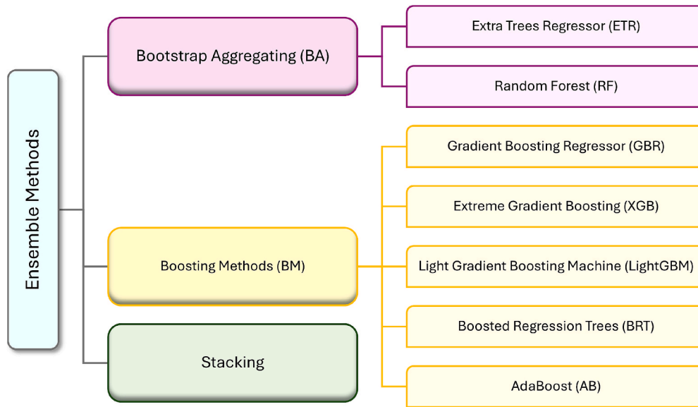
Fig. 11. Categorization of ensemble machine learning methods used in PV/T modeling.
