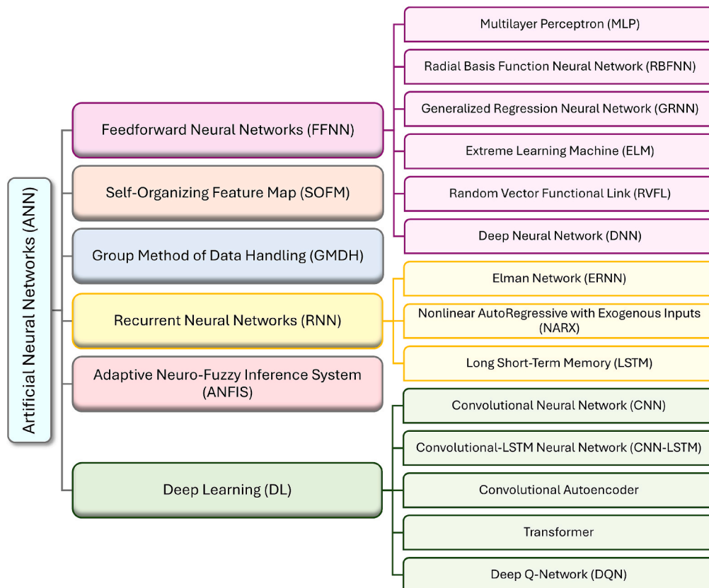
Fig. 9. Categorization of ANN models used in PV/T modeling.
