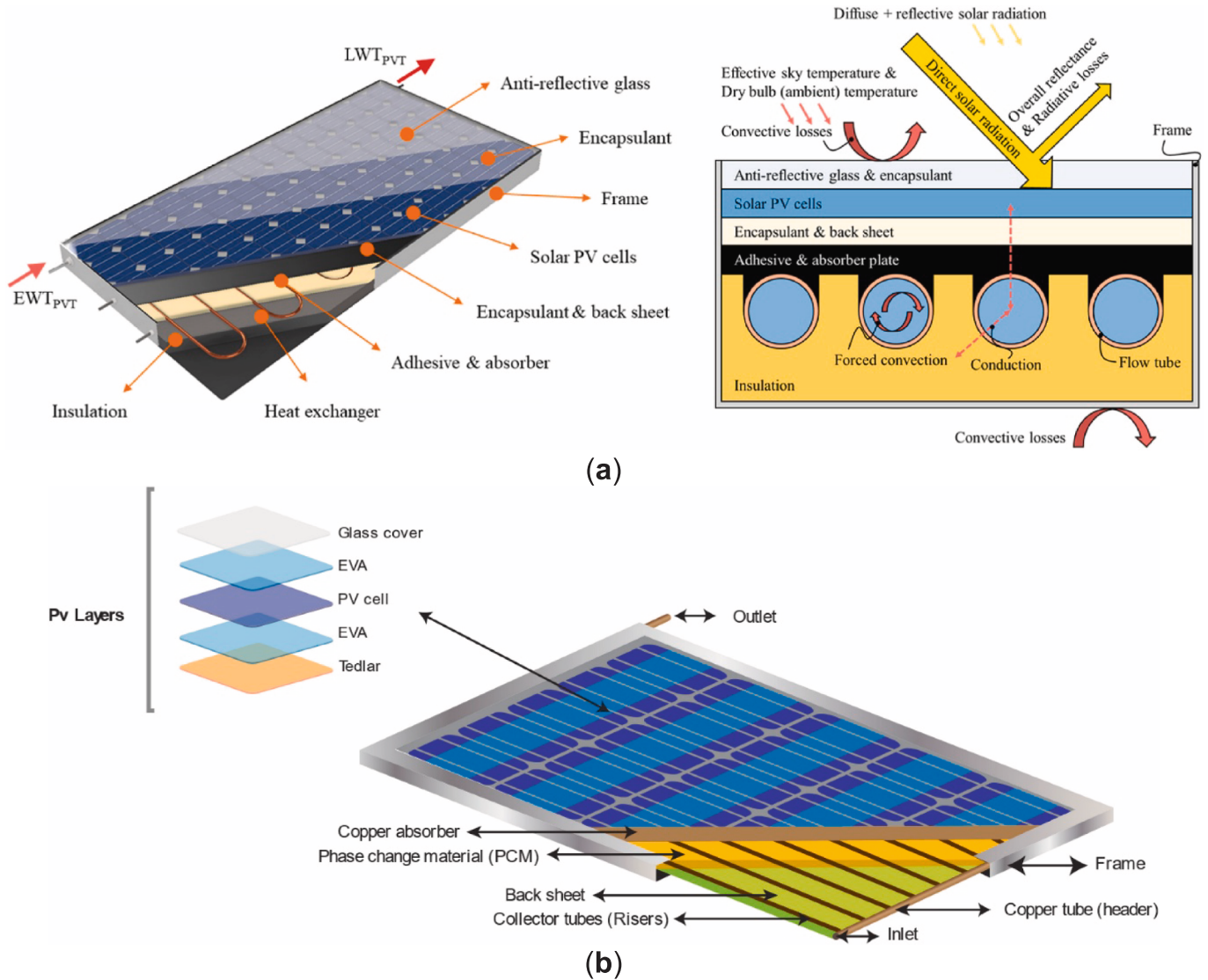
Fig. 1. Liquid-based photovoltaic-thermal (PV/T) system configurations: (a) Energy conversion processes and heat transfer mechanisms in basic PV/T systems [126]; (b) Advanced multi-layered PV/T system with phase change material (PCM) [107].
