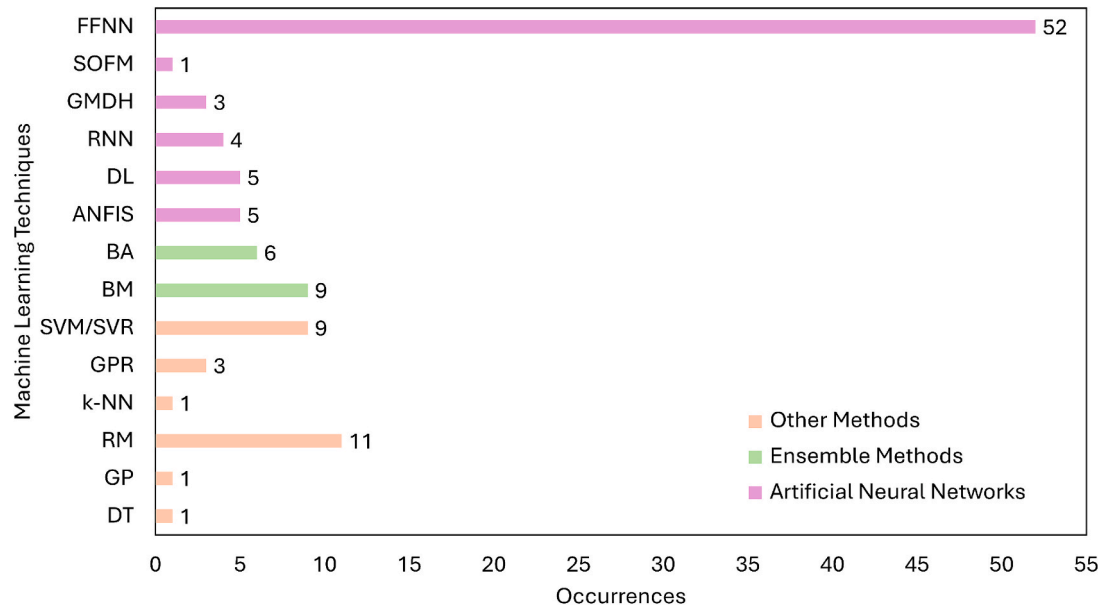
Fig. 7. Distribution of machine learning techniques used in PV/T system modeling.
