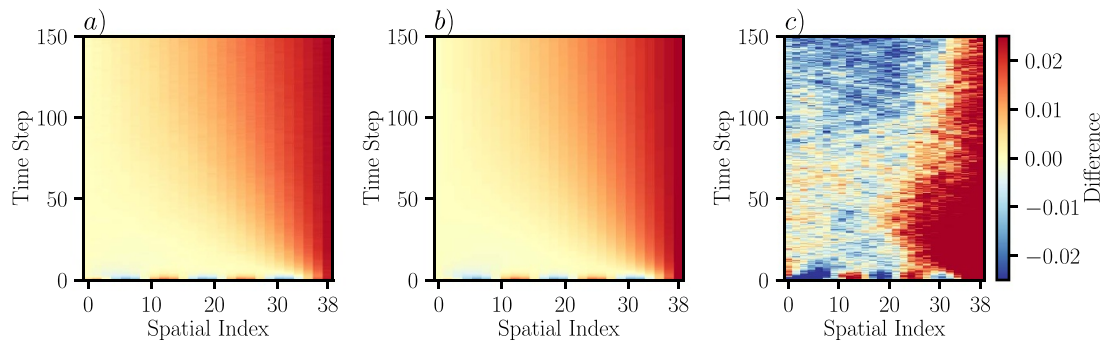
Figure 10. MD vs trained model with (a) the MD time space plot over 3000 timesteps of size 0.05, with model trained in (b) where weights are [0.984, -1.96, 0.976] and difference between the model and MD in (c) showing the extra physics in the MD simulation not captured by the mdCNN, which includes both noise as well as an apparent signal, which may indicate local viscosity variation, near the top boundary. The colour map in panels (a) and (b) represent the local solutions of MD and trained model (mdCNN). In panel (c) the colour map represents difference between (a) and (b).
