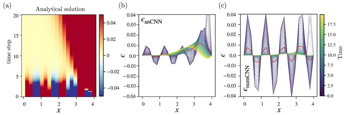
Figure 6. Comparison of CNN kernel training against the analytical solution for Couette flow bBC = 0.0 , tBC = 1.0 and u_0 = \sin(2.0\pi x) . (a) Analytical (exact) solution for Couette flow. The error curves (difference between the analytical solution and the solution obtained from the CNN models) at different timesteps for CNN trained on (b) analytical data, and (c) numerical data. The color bar at the far right denotes time and applies to both these panels. The red curve in both panels denotes the error when time-averaged over the entire simulation. The colour map represents in panel (a) represents the local values of u(x,t) . The simulation parameters used are: \mu = 0.02 , \Delta t = 0.1 , n_x = 20 , L_x = 4.0 , N_t = 200 , \Delta x = L_x/(n_x - 1) .
