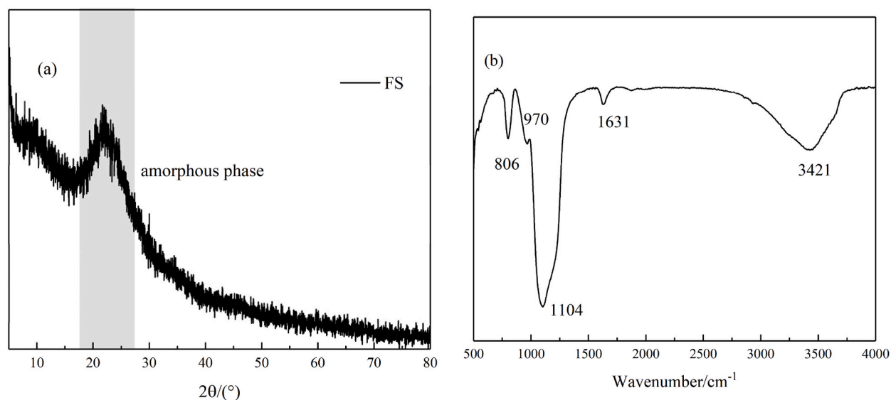
Fig. 1. XRD pattern and FTIR spectra of FS.
