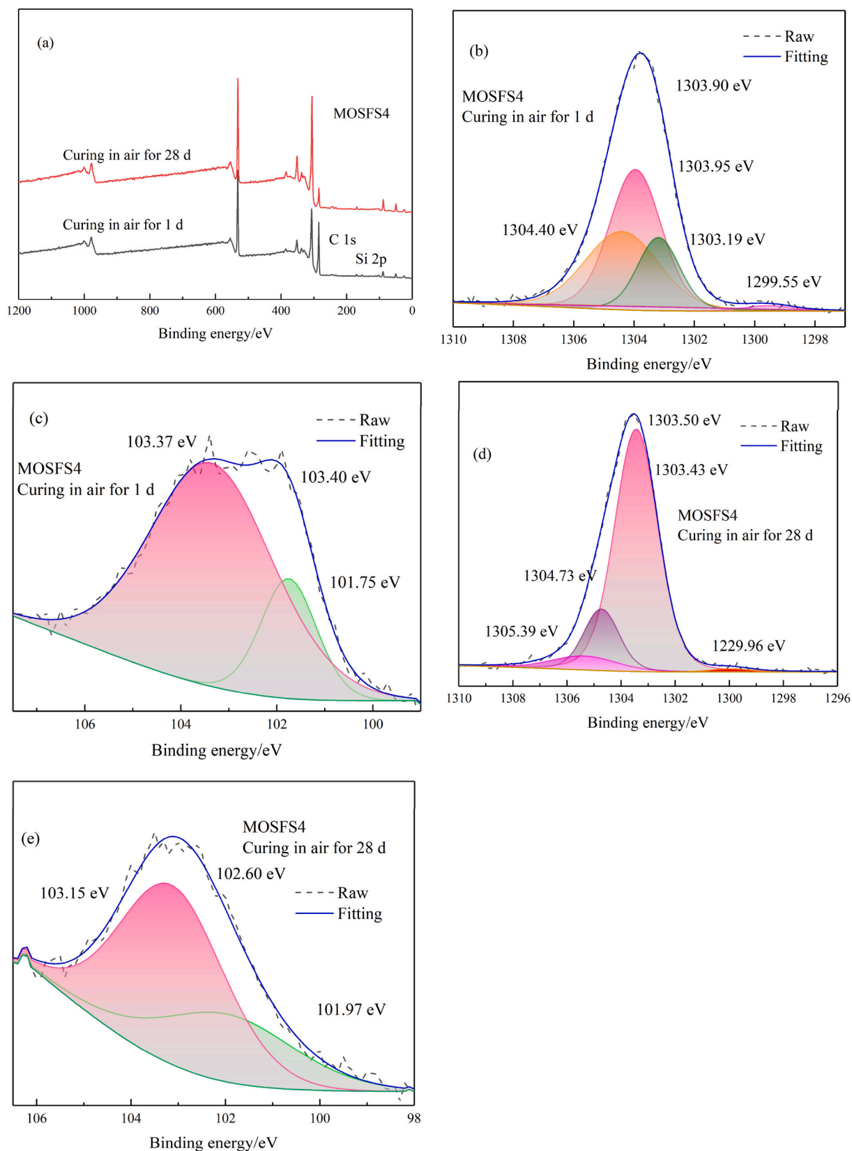
Fig. 9. XPS data of MOSFS4: (a): XPS spectra; (b), (d): Mg 1s; (c), (e): Si 2p.
