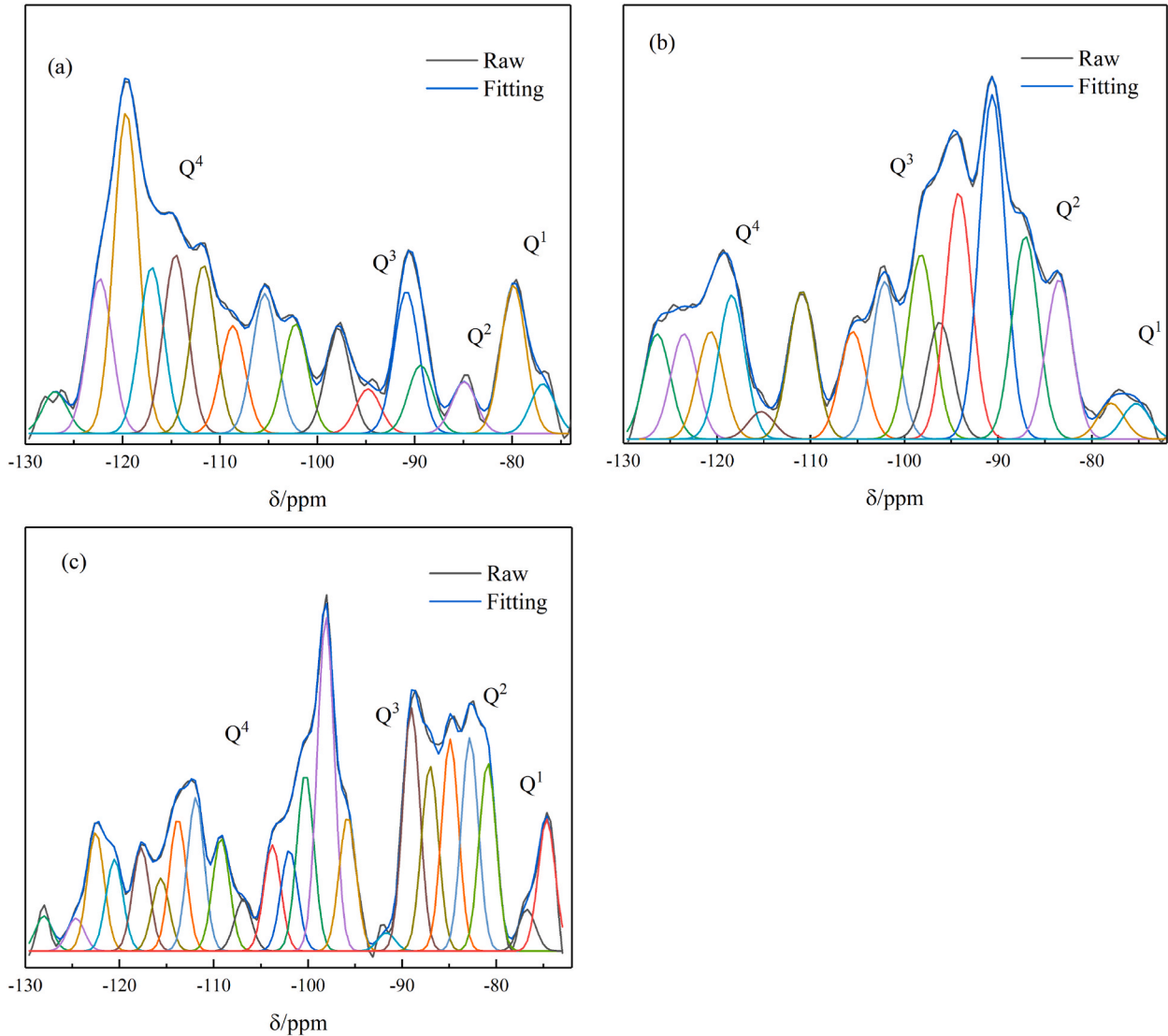
Fig. 6. 29 Si NMR spectra of MOSFS4 cured in air for (a) 1 d; (b) 7 d; and (c) 28 d.
