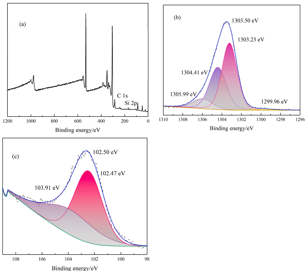
Fig. 13. XPS data of MOSFS4 after 90 d of water immersion: (a) XPS spectra; (b) Mg 1s; (c) Si 2p.
