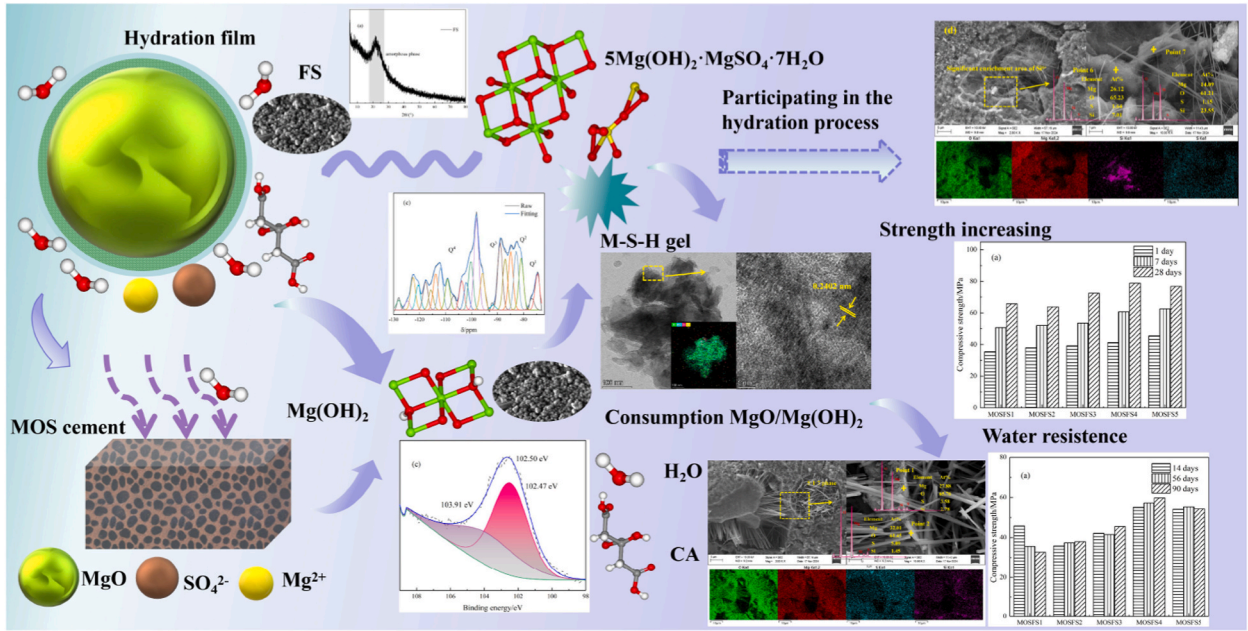
Fig. 16. Proposed hydration and strengthening mechanism of white carbon black (FS) in magnesium oxysulfate (MOS) cement.
