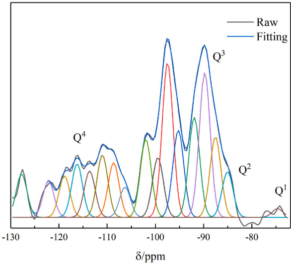
Fig. 14. ^{29}\text{Si} NMR spectra of MOSFS4.
