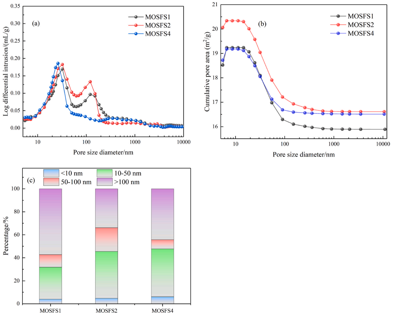
Fig. 7. Pore structure of MOS cement: (a) pore size distribution; (b) pore area; (c) pore contents with different sizes.
