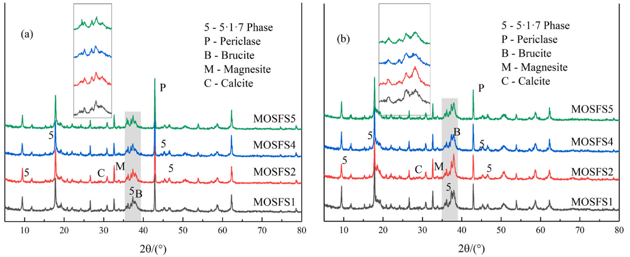
Fig. 4. XRD patterns (a) 1 d; and (b) 28 d.
