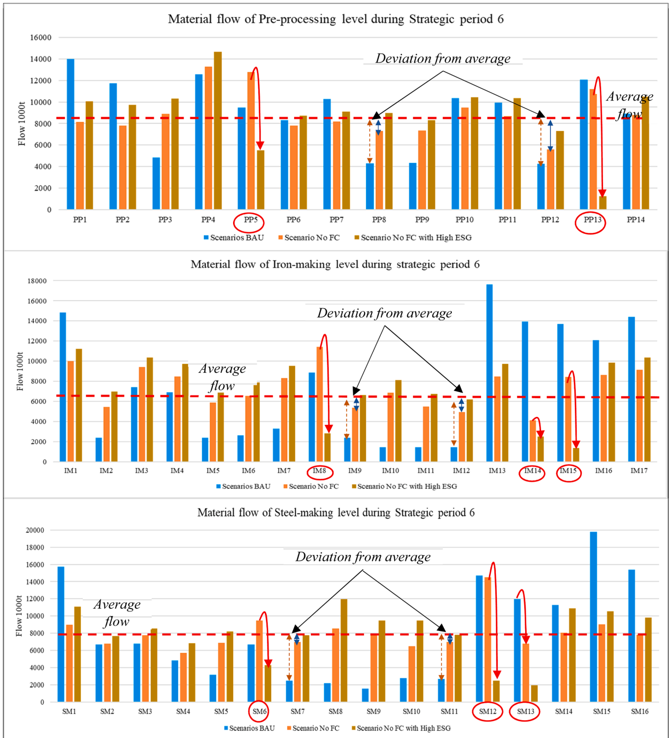
Fig. 7. Material Flow of units at different levels of steel SCN during period 6, under Scenarios BAU, No FC, and No FC with High ESG.
