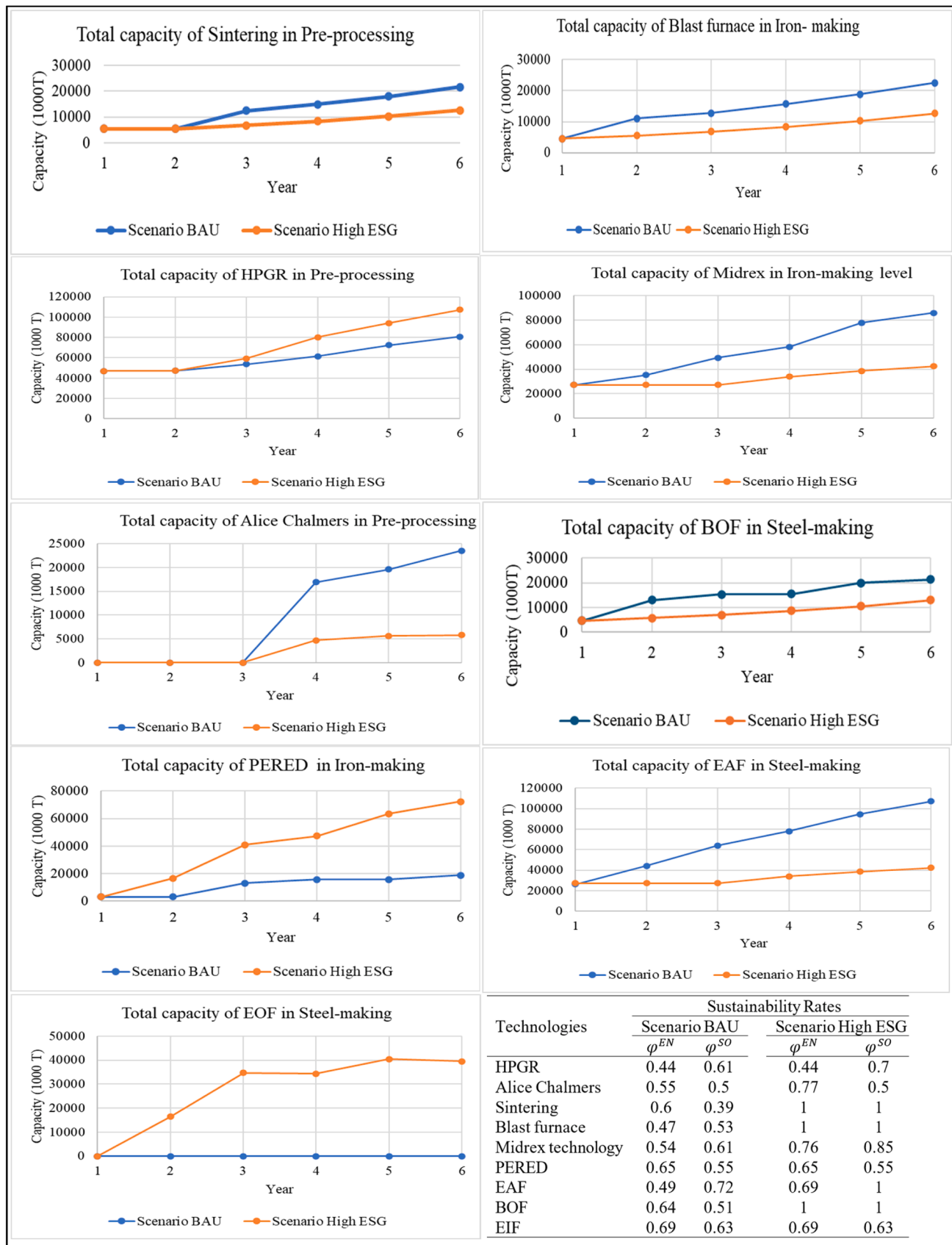
Fig. 6. Capacity choices for each technology under sustainability rate scenarios.
