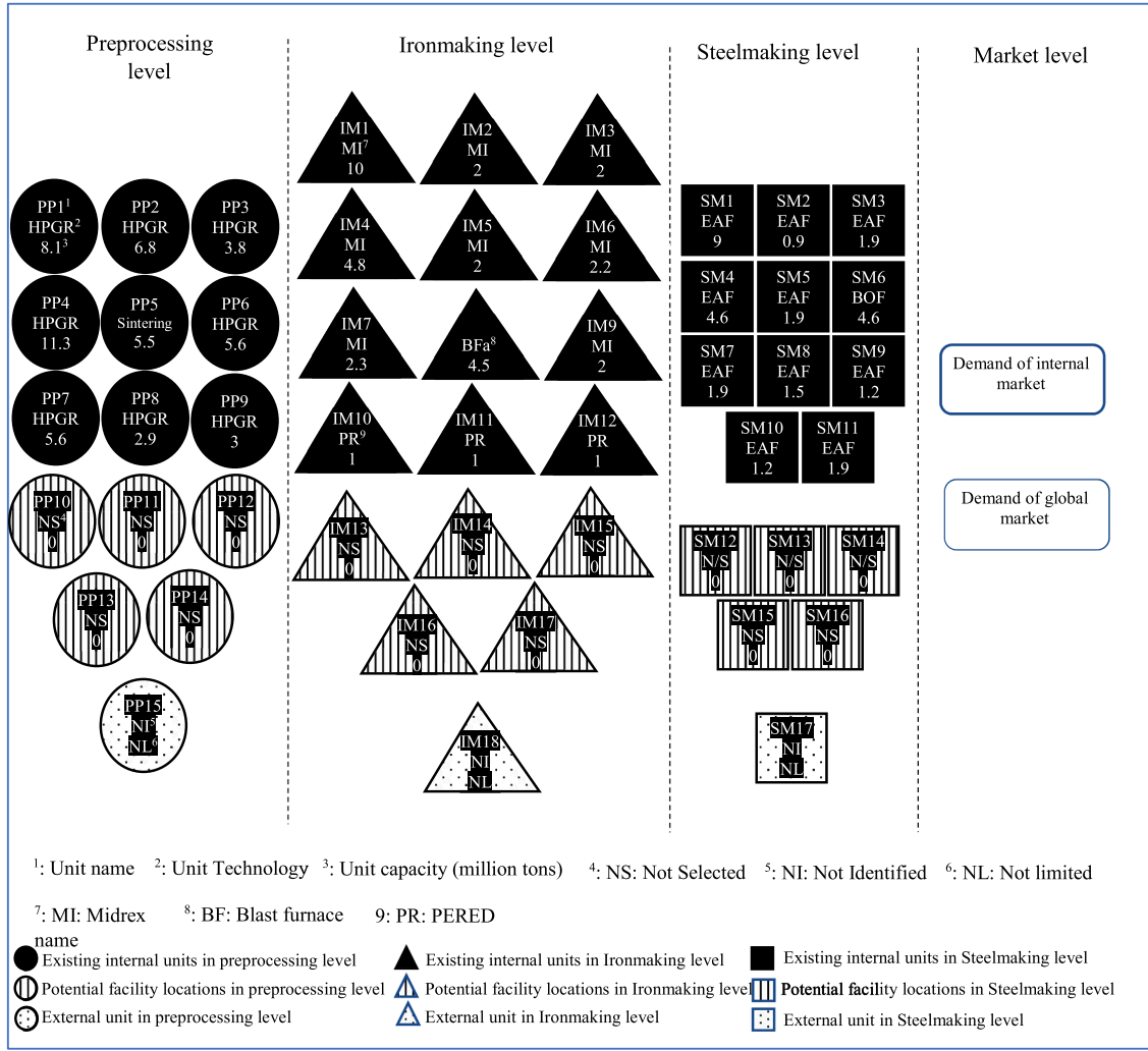
Fig. 3. Current Steel SCN in our case study.
