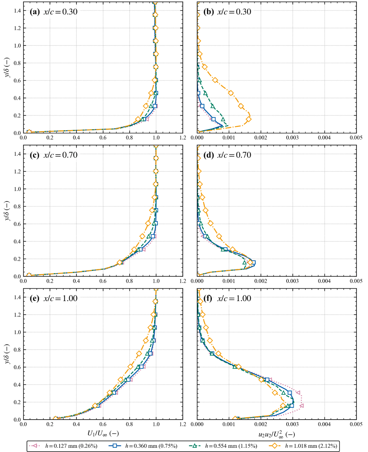
Fig. 12. Evolution of boundary layer structure for varying trip height h at Re_c = 1.0 \times 10^6 . The left column (a,c,e) shows the normalised mean velocity profiles U_1/U_\infty , while the right column (b,d,f) presents the corresponding wall-normal Reynolds stress distributions \overline{u_2 u_2}/U_\infty^2 . Profiles are shown at three streamwise stations: x/c = 0.30, 0.70 , and 1.00 . The results illustrate the influence of trip height on transition onset, turbulence development, and downstream recovery.
