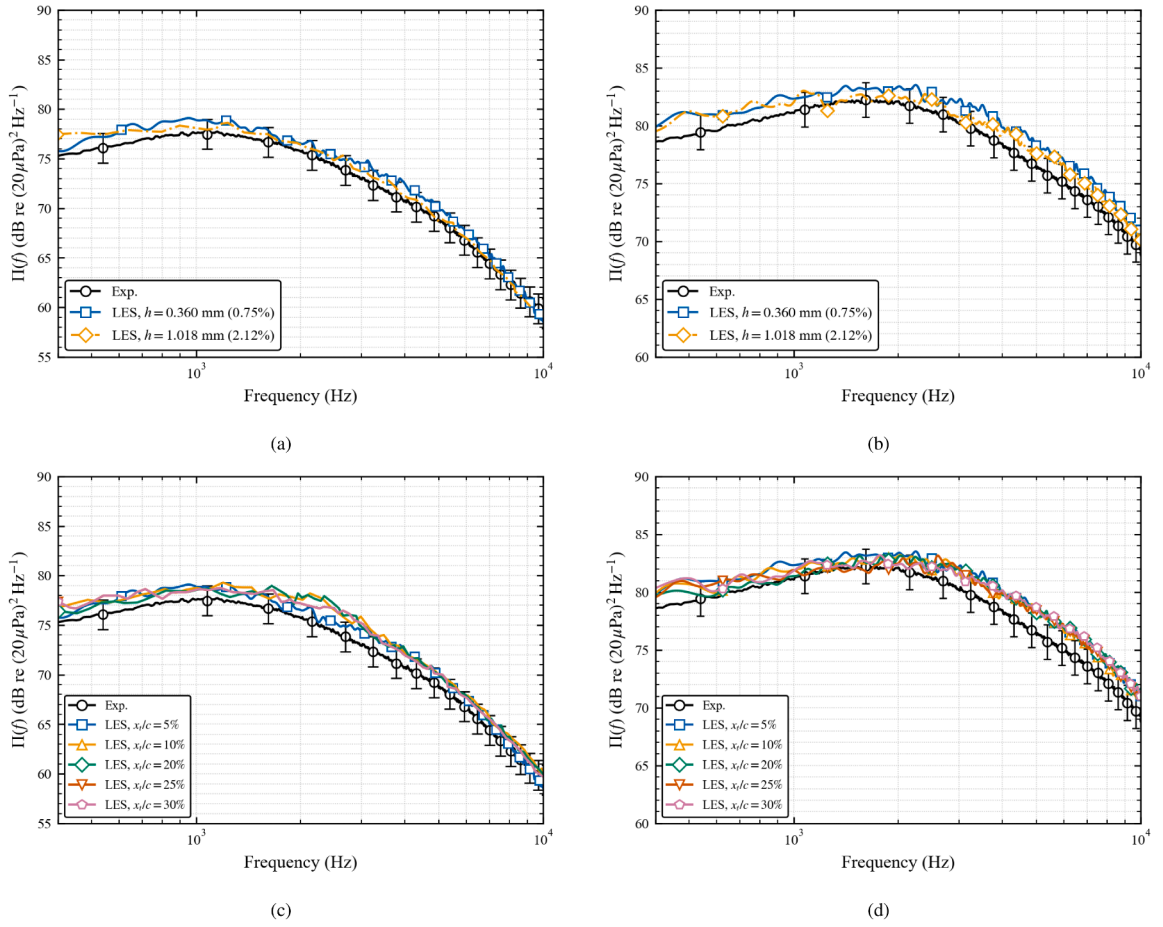
Fig. 14. Effect of trip height (a,b) and trip location (c,d) on trailing-edge wall-pressure spectra. Left column (a,c): Re_c = 1.0 \times 10^6 ; right column (b,d): Re_c = 1.5 \times 10^6 . Experimental measurements are shown for reference [25].
