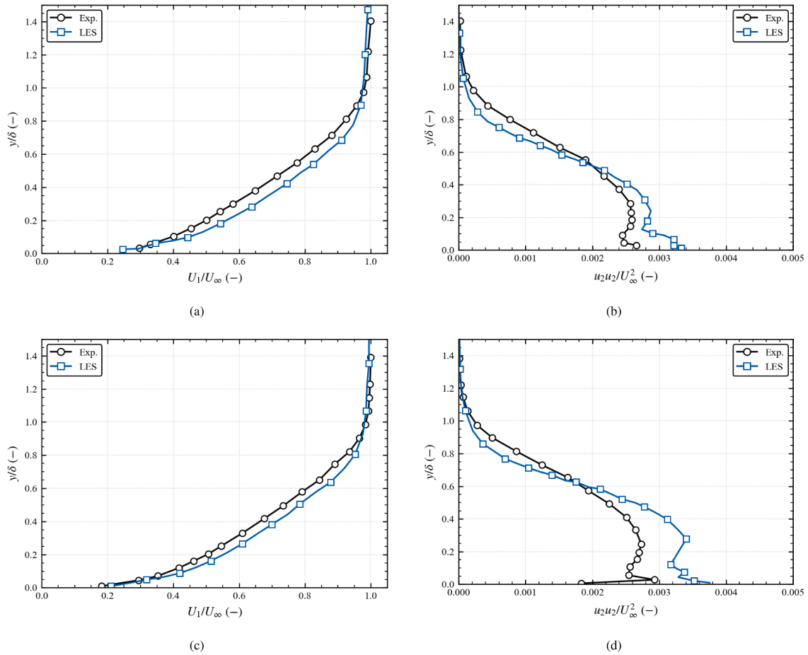
Fig. 7. Comparison of boundary-layer profiles at x/c = 1.0038 : mean velocity U_1/U_\infty for (a) Re_c = 1.5 \times 10^6 and (c) Re_c = 1.0 \times 10^6 , and wall-normal Reynolds stress \overline{u_2 u_2}/U_\infty^2 for (b) Re_c = 1.5 \times 10^6 and (d) Re_c = 1.0 \times 10^6 . WMLES results (LES) are compared with the BANC-III experiment (Exp.).
