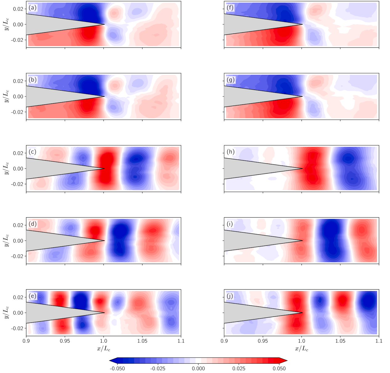
Fig. 16. Spatial structures of the leading POD modes and of the conditionally-averaged difference field around the airfoil trailing edge, for two trip heights: left column (a–e) h = 0.127 mm and right column (f–j) h = 1.018 mm. All panels share the same dimensionless colour scale: the POD spatial modes \phi_j(\mathbf{x}) are unit-normalised eigenvectors ( \int \phi_j^2 d\mathbf{x} = 1 ), and the conditionally-averaged difference field \Delta Q is scaled by 2\sigma_{a_1} so that \Delta Q/(2\sigma_{a_1}) is directly comparable in magnitude to \phi_1 . (a, f) First POD mode \phi_1 ; (b, g) conditionally-averaged difference field \Delta Q (Eq. (24)); (c, h) second POD mode \phi_2 ; (d, i) third POD mode \phi_3 ; (e, j) fourth POD mode \phi_4 .
