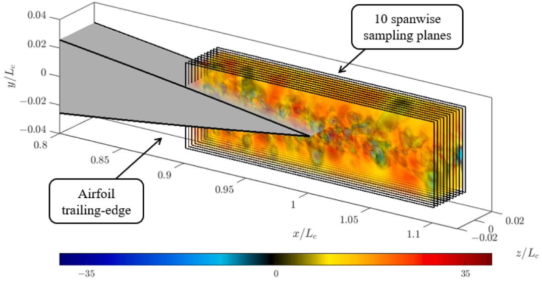
Fig. 3. Instantaneous near-field pressure fluctuation, Q(\mathbf{x}, t) (Eq. (16)), sampled on the ten spanwise planes used for the POD analysis.
