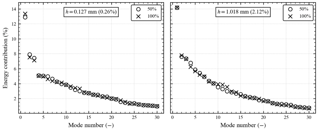
Fig. 15. Relative modal energy for two trip heights: (a) h = 0.127 mm and (b) h = 1.018 mm. Results obtained using 50% and 100% of the available snapshots are compared, confirming negligible sensitivity of the energy distribution to the number of time samples.
