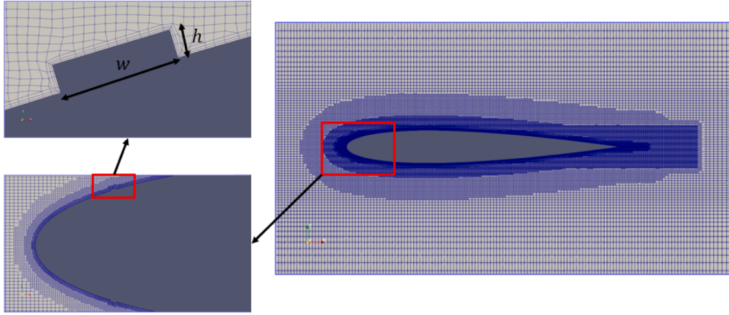
Fig. 2. Computational mesh topology for the NACA 0012 airfoil showing the leading-edge step trip (top left), the leading-edge region (bottom left), and the overall mesh distribution around the airfoil (right).
