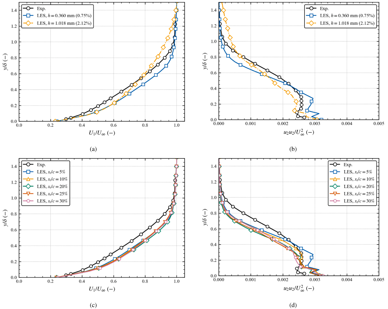
Fig. 11. Effect of trip height and trip location on boundary layer structure at x/c = 1.0038 and Re_\rho = 1.5 \times 10^6 . The left column (a,c) shows the normalised mean velocity profiles U_1/U_\infty and the right column (b,d) shows the corresponding wall-normal Reynolds stress distributions u_2 u_2 / U_\infty^2 . The top row corresponds to variations in trip height, and the bottom row corresponds to variations in trip location. Experimental data (Exp. [25]) are included for reference.
