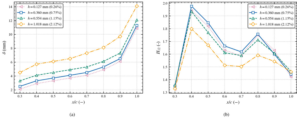
Fig. 13. Influence of trip height h on integral boundary-layer parameters at Re_c = 1.0 \times 10^6 . The left panel shows the streamwise evolution of boundary layer thickness \delta , while the right panel presents the corresponding shape factor H_{12} = \delta^*/\theta . Larger trip heights promote earlier transition and produce a thicker boundary layer downstream.
