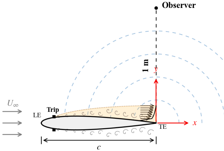
Fig. 1. Schematic of the NACA 0012 airfoil, coordinate system, and observer location. The microphone is positioned 1 m vertically above the trailing edge (TE). Top and bottom trip devices are symmetrically positioned to preserve the axial symmetry of the NACA 0012 airfoil profile.
