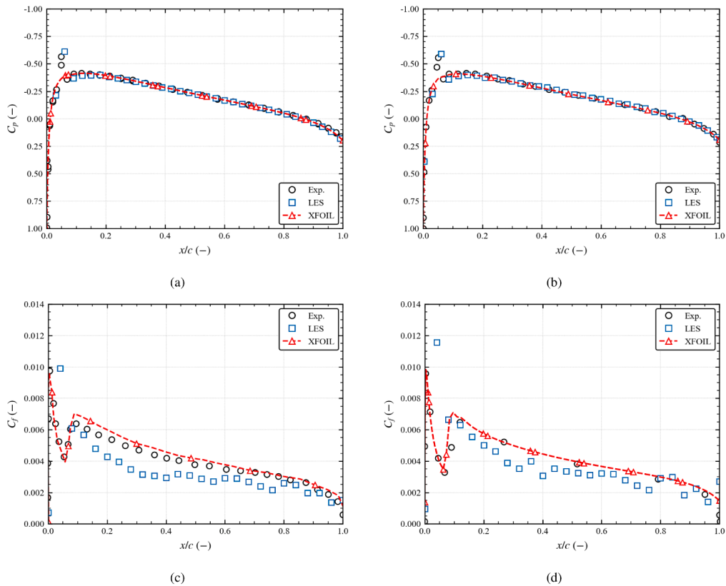
Fig. 6. Comparison of the pressure coefficient C_p for (a) Re_c = 1.5 \times 10^6 and (b) Re_c = 1.0 \times 10^6 , and the skin-friction coefficient C_f for (c) Re_c = 1.5 \times 10^6 and (d) Re_c = 1.0 \times 10^6 , comparing the WMLES results (LES), BANC-III experiment (Exp.), and empirical XFOIL model.
