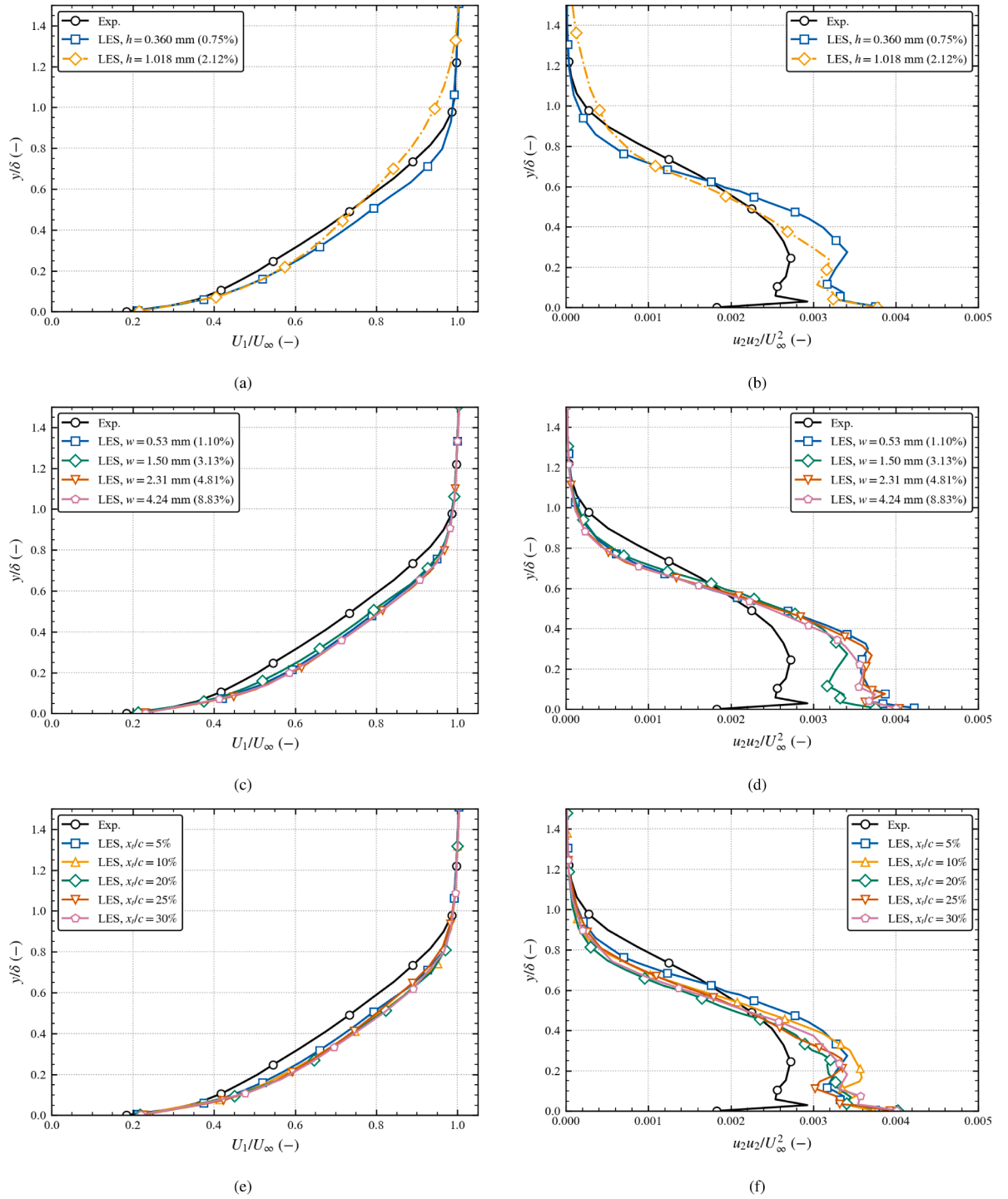
Fig. 10. Effect of trip parameters on the boundary layer structure at x/c = 1.0038 and Re_c = 1.0 \times 10^6 : left column (a,c,e) shows the normalised mean velocity profiles U_1/U_\infty and right column (b,d,f) shows the corresponding wall-normal Reynolds stress distributions \bar{u}_2 \bar{u}_2 / U_\infty^2 . Rows correspond to variations in trip height (top), trip width (middle), and trip location (bottom). Experimental data (Exp. [25]) are included for reference.
