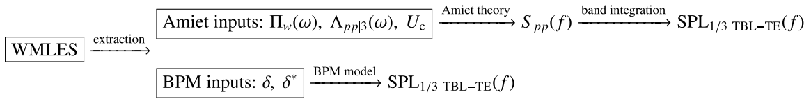
Fig. 4. Workflow for far-field noise prediction. Flow statistics extracted from the WMLES are used as inputs to Amiet’s analytical trailing-edge noise theory and the empirical BPM model.
