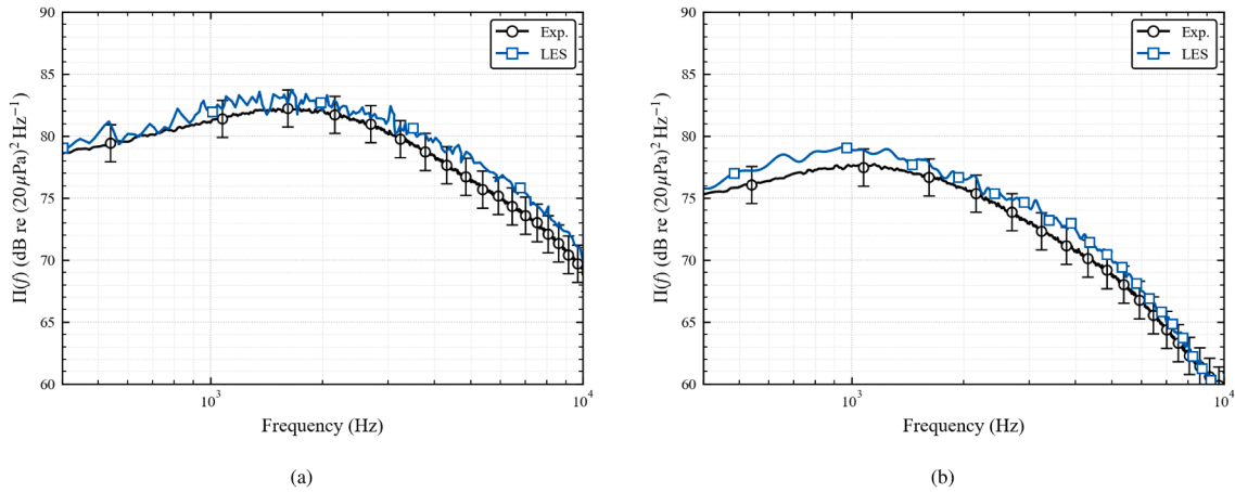
Fig. 8. Comparison of trailing-edge wall-pressure spectra at x/c = 0.989 and \alpha = 0^\circ for (a) Re_c = 1.5 \times 10^6 and (b) Re_c = 1.0 \times 10^6 , comparing the WMLES predictions (LES) and BANC-III experiment (Exp.). Error bars of \pm 1.5 dB are included in accordance with the BANC-III uncertainty reported by Herr et al. [25].
