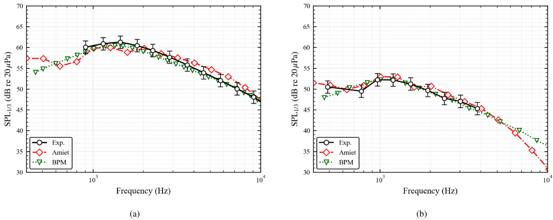
Fig. 9. Comparison of third-octave noise spectra for (a) Re_c = 1.5 \times 10^6 and (b) Re_c = 1.0 \times 10^6 predicted by the Amiet model and the BPM model based on the same LES solutions with the acoustic measurements (Exp.). The observer angle is \Theta = 90^\circ , and the sound pressure level is normalised to a reference distance of 1 m.
