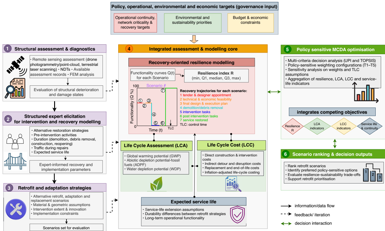
Fig. 1 | Decision-oriented framework for bridge adaptation under uncertainty. Presents an integrated six-step methodology linking structural diagnostics, expert-informed recovery modeling, sustainability assessment, and policy-sensitive decision optimization for ageing bridges. Governance inputs include operational continuity and recovery targets, environmental and sustainability priorities, and budget and economic constraints. Step 1 integrates structural assessment and diagnostics using remote sensing, non-destructive testing, inspection records, and numerical modeling to identify deterioration and damage states. Step 2 applies structured expert elicitation to define intervention and recovery parameters, including restoration strategies, implementation sequencing, intervention durations, operational continuity during works, and expected service life. Step 3 defines retrofit and adaptation scenarios, spanning repair, strengthening, and replacement strategies, while accounting for material assumptions, intervention extent, and
