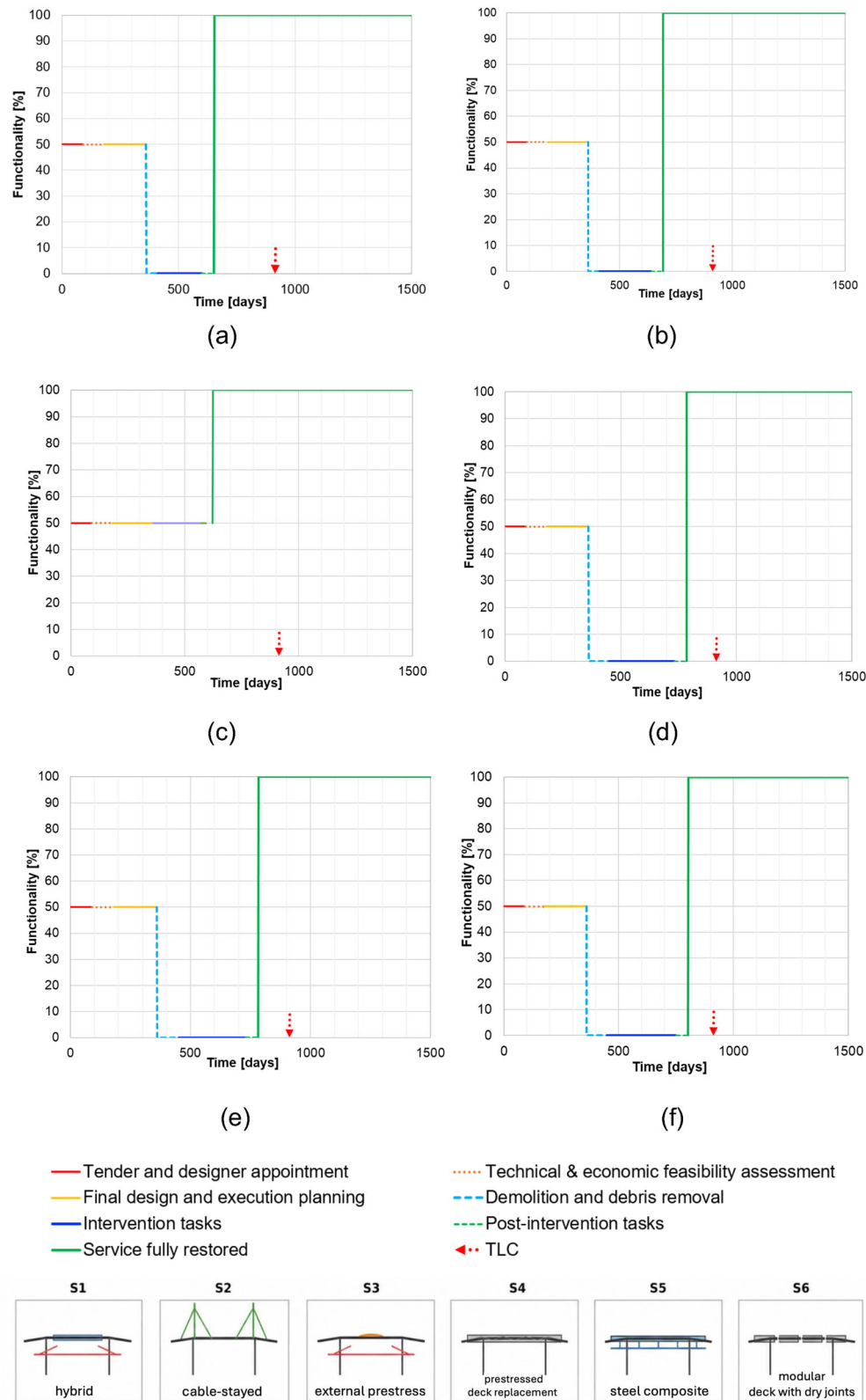
Fig. 3 | Functionality curves for six retrofit scenarios (median values, Q2). a Scenario #1; b Scenario #2; c Scenario #3; d Scenario #4; e Scenario #5; f Scenario #6. These ex-ante curves, constructed for comparative evaluation within a decision-oriented framework, illustrate distinct recovery profiles. Scenario #3 achieves full recovery in approximately 21 months while uniquely maintaining partial service throughout the intervention. Scenarios #1 and #2 recover efficiently in just under
