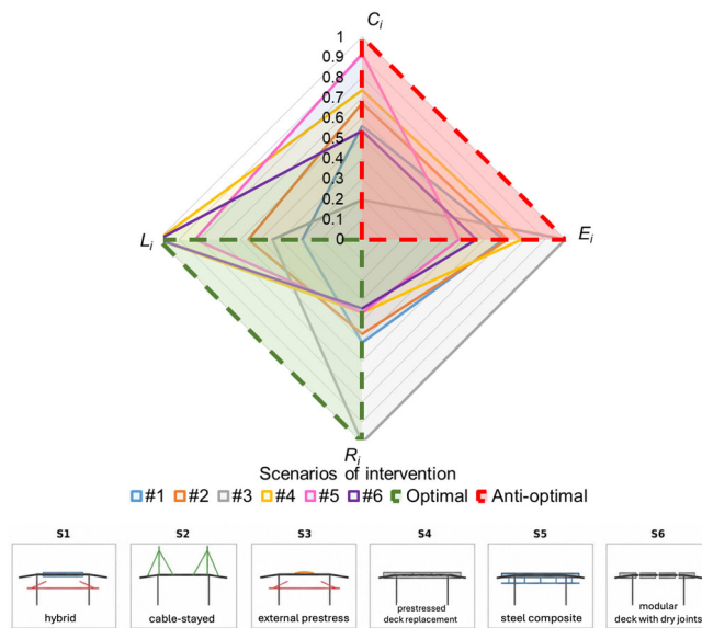
Fig. 10 | Multi-criteria decision space for retrofit strategy selection. Normalized multi-criteria representation of the retrofit scenarios, minimizing cost ( C_i ) and environmental impact ( E_i ) while maximizing resilience ( R_i ) and service life ( L_i ). Each marker corresponds to a retrofit scenario (#1–#6), positioned according to its normalized performance across the considered criteria. The shaded region identifies the subset of solutions that achieve favorable trade-offs across all objectives under the selected weighting scheme, defining the preferred decision space. Axes represent normalized criteria values, with higher values indicating improved performance. The green dashed region indicates the preferred decision space, whereas the red dashed region represents non-optimal solutions.
