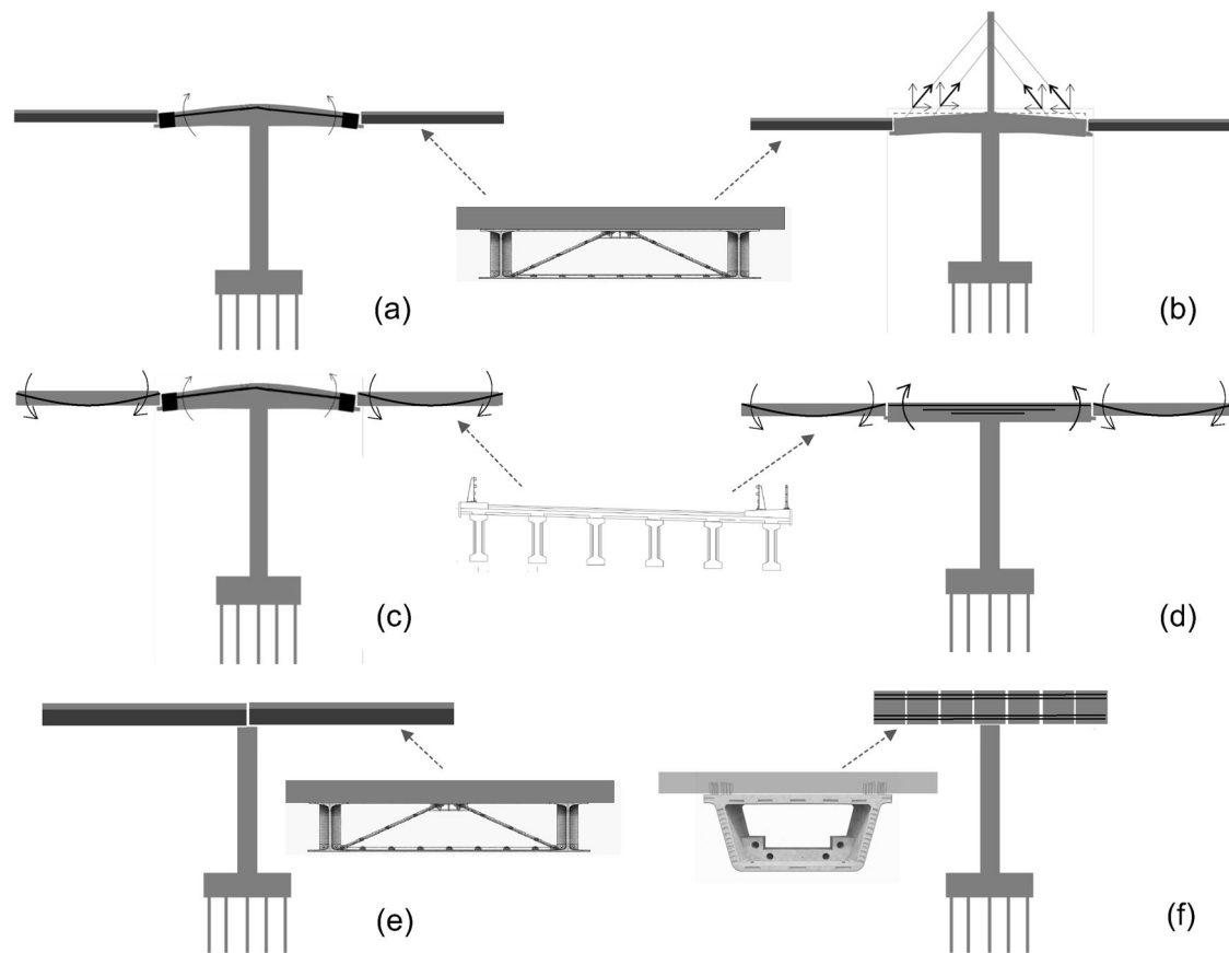
Fig. 2 | Retrofit scenarios for the defected part of the bridge deck. It is proposed that the balanced cantilever part of the deck can be retrofitted by: a Scenario #1 – hybrid intervention with preservation of cantilever beams, replacement of simply supported members with steel beams, and application of external prestressing. b Scenario #2 – stay cable augmentation with new pylons and stays anchored to the main piers to redistribute forces and increase structural redundancy. c Scenario #3 – external prestressing solution retaining cantilevers and simply supported beams
