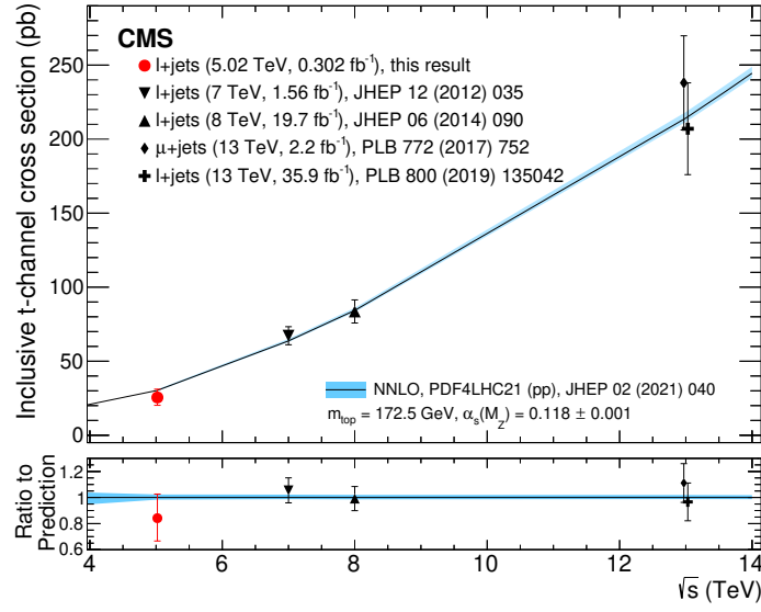
Figure 9. Summary of the CMS measurements of the t -channel single top quark production cross section as a function of \sqrt{s} .
