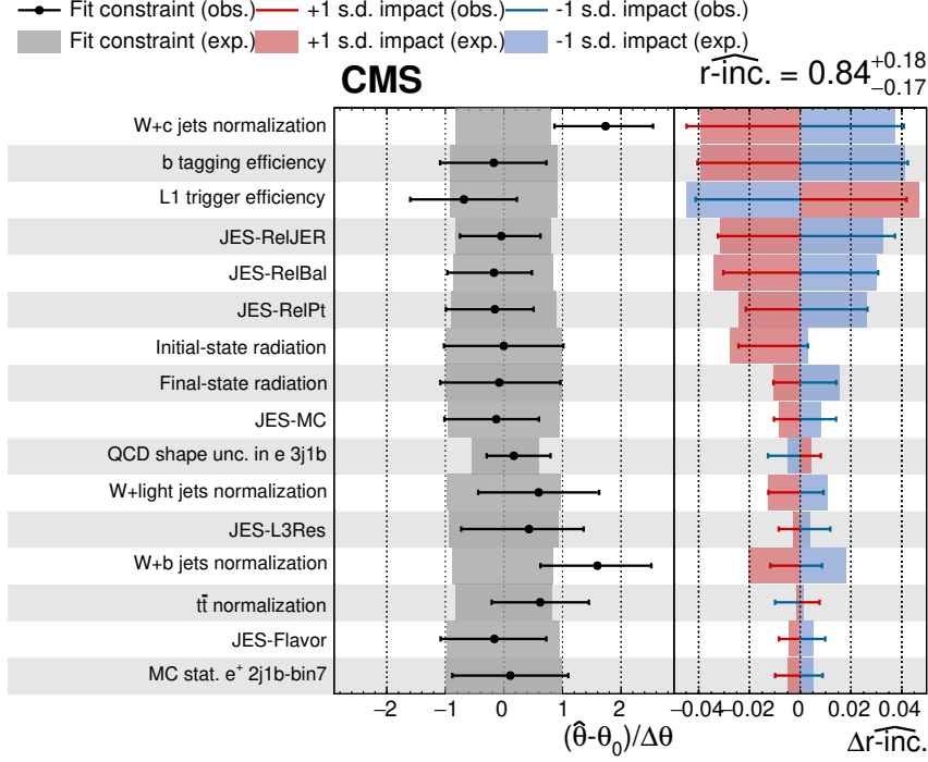
Figure 7. The largest impacts of nuisance parameters on the signal strength, \Delta \widehat{r\text{-inc.}} (right column) and ratios (\hat{\theta} - \theta_0)/\Delta\theta (middle column) for the nuisance parameters listed in the left column from the ML fit used to determine the measured tq + \bar{t}q cross section. The horizontal bars in the middle column show the ratio of the uncertainties of the fit result to the pre-fit ones, indicating the constraint on the nuisance parameter. The JES uncertainties are divided into several sources related to the various methods used to extract the uncertainties as described in ref. [31].
