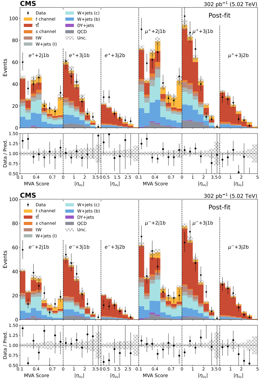
Figure 6. Distributions for the \ell^+ + \text{jets} (upper) and \ell^- + \text{jets} (lower) categories where the prediction parameters are set to the values obtained in the fit. They show the MVA score and |\eta_{u_0}| distributions, which are the fitted variables in the ML fit in the 2j1b category and the categories with three jets, respectively. The vertical error bars represent the statistical uncertainty associated to the data, and the hatched band the uncertainty of the prediction, after the fit. All uncertainties considered in the analysis are included in the uncertainty band. The lower panels show the ratio of data to prediction. The first and last bins in the MVA output distributions include underflow and overflow events, respectively.
