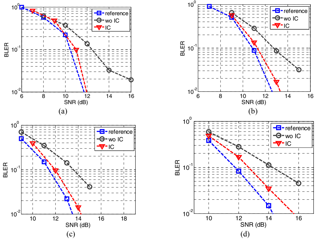
Fig. 6 BLER performance of different Doppler frequency scenarios: (a). 5 Hz; (b). 70 Hz; (c). 150 Hz; (d). 200 Hz
