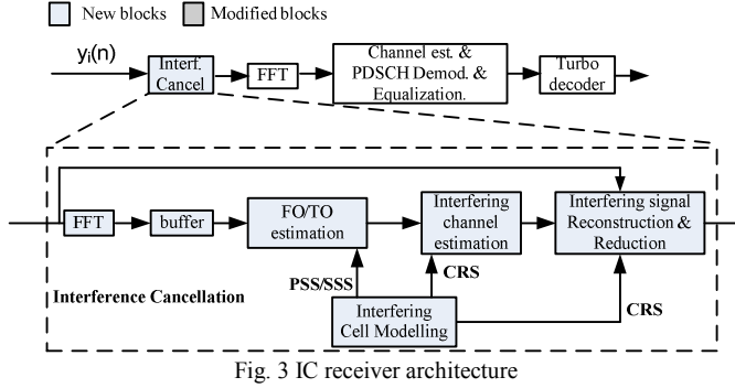
Fig. 3 IC receiver architecture
