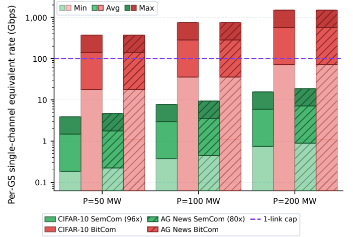
Fig. 3. Per-GS equivalent single-channel data rate required to achieve X_{\max} on the CIFAR-10 and AG News datasets under different SDC power budgets.
