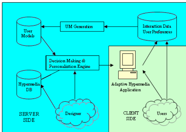
Fig. 1. Generic Architecture of an Adaptive Hypermedia Application.
