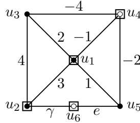
FIGURE 14. Hypergraph representation (H', \{5, -3\}) of M_e^* , where 5 is incident with colored vertices and -3 is incident with boxed vertices.
