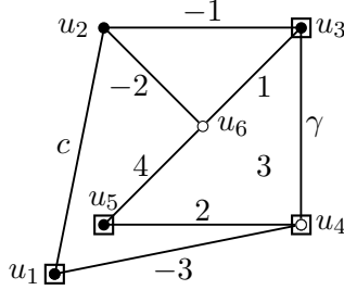
FIGURE 12. Hypergraph representation (H', \{5, -4\}) of M_c^* , where 5 is incident with colored vertices and -4 is incident with boxed vertices.
