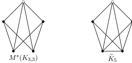
FIGURE 3. Graft representations of M^*(K_{3,3}) and \tilde{K}_5 .
