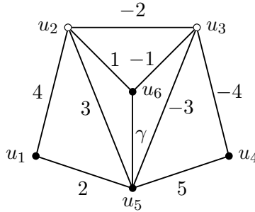
FIGURE 10. A graft representation, (H', a) , of M_a^* , where a is incident with colored vertices.
