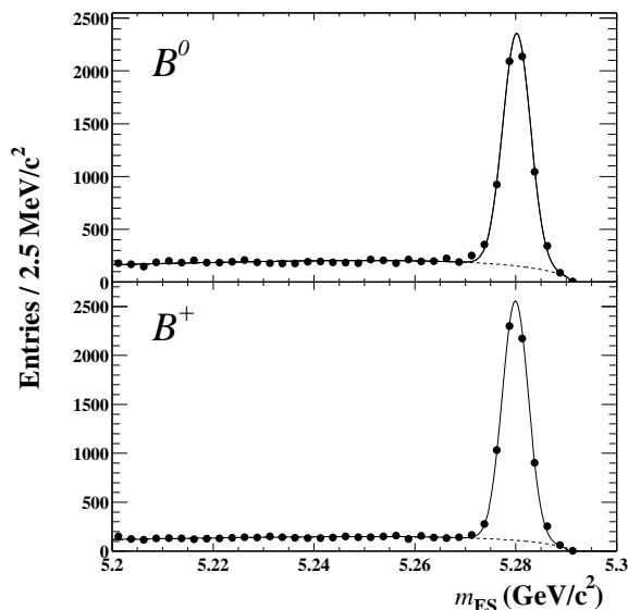
FIG. 1: m_{\text{ES}} distributions of the selected neutral (top) and charged (bottom) B_{\text{rec}} candidates.
