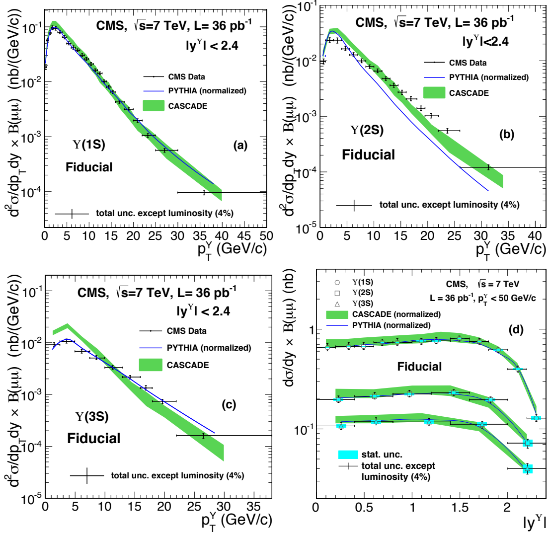
Figure 2: Differential fiducial cross section of (a) Y(1S) , (b) Y(2S) , and (c) Y(3S) as a function of p_T^Y in the rapidity range |y^Y| < 2.4 , and comparison to the predictions from CASCADE and PYTHIA. (d) Differential fiducial cross section of the Y(nS) as a function of rapidity and comparison to the predictions from CASCADE and PYTHIA. The PYTHIA prediction is normalized to the measured total cross section, in order to facilitate the comparison of the shape of the dependences. The full CASCADE prediction is shown in (a), (b), and (c); the normalised CASCADE prediction is shown in (d). The bands indicate the estimated uncertainties in the CASCADE prediction.
