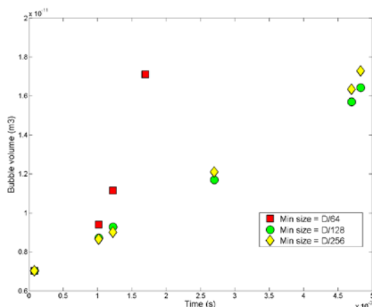
Fig 2. Bubble growth with different mesh sizes
