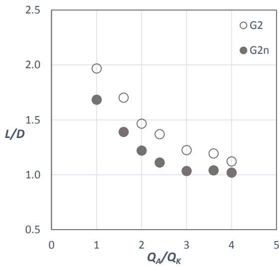
Figure 6: Effect of the type of aqueous phase on the slug size.
