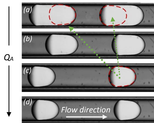
Figure 4: Effect of flow rate on the slug size for G2n and for Q_A ( \mu\text{L}/\text{min} ): (a) 50, (b) 100, (c) 150, (d) 200.
