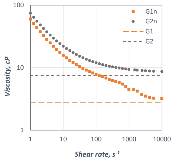
Figure 7: Viscosity vs shear rate for the fluids used.
