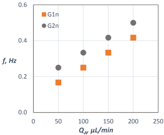
Figure 10: Effect of the aqueous-phase viscosity on the slug frequency (non-Newtonian fluids).
