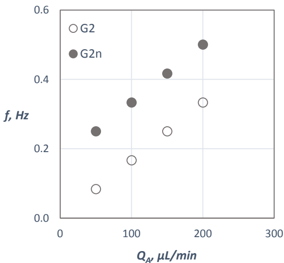
Figure 11: Effect of the aqueous-phase viscosity (non-Newtonian and Newtonian) on the slug frequency.
