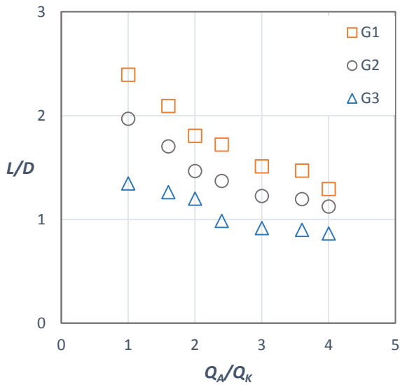
Figure 5 Effect of the aqueous-phase viscosity on the slug size (Newtonian fluids).
