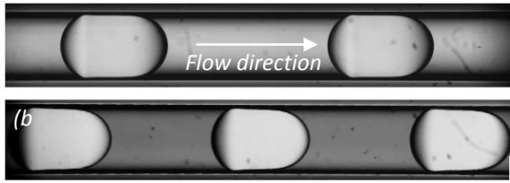
Figure 9: Effect of aqueous-phase viscosity on the size, shape and frequency of slugs for (a) G1n , (b) G2n (non-Newtonian fluids, Q_A = 100 \mu\text{L}/\text{min} ).
