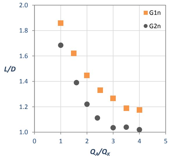
Figure 8: Effect of the non-Newtonian aqueous-phase viscosity on the slug size.
